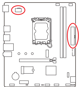
CPU_PWR1
