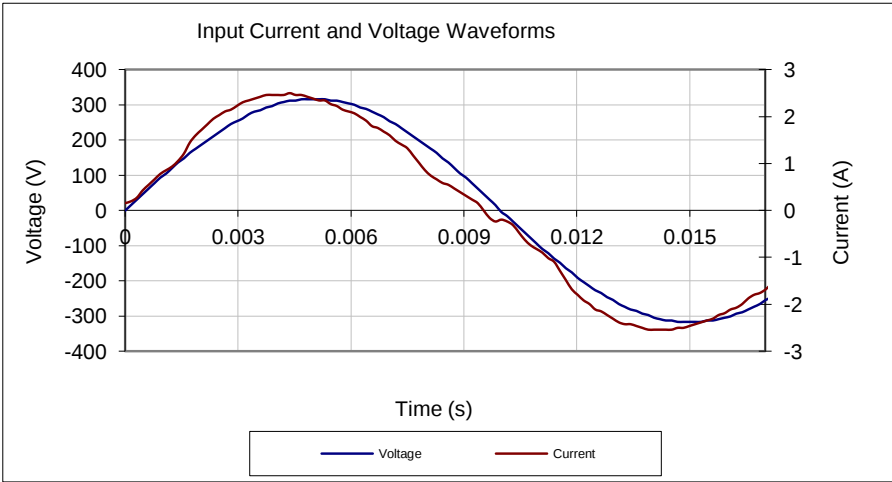
Input AC Current Waveform (ITHD = 8.4%, 50% Load)
