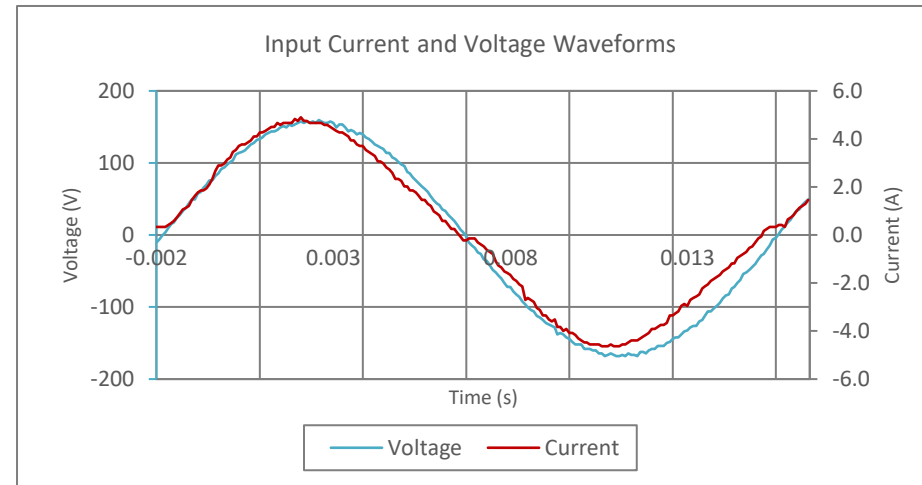
Input AC Current Waveform (ITHD = 8.08%, 50% Load)
