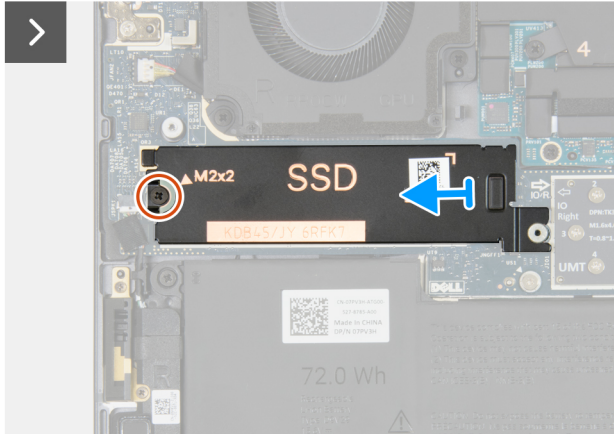
Figure 23. Removing the M.2 2280 solid state drive
