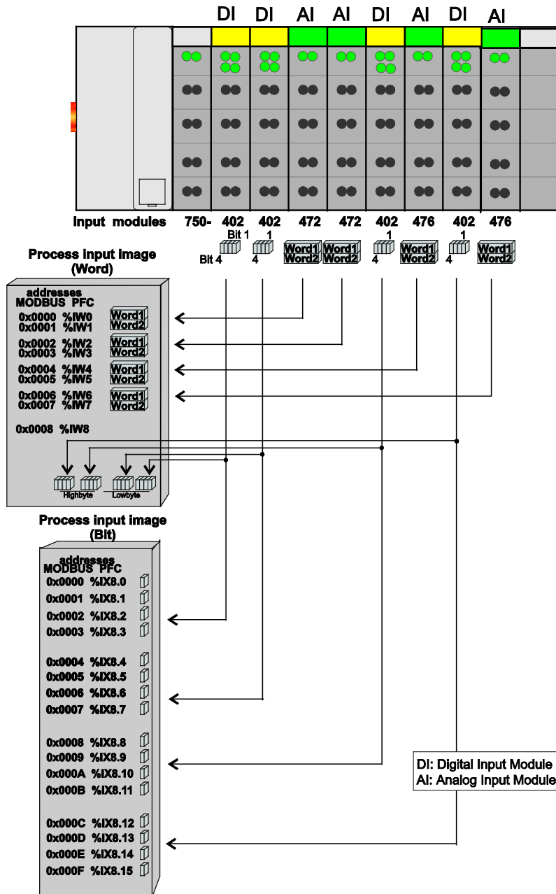
Figure 39: Example of Process Image for Input Data
