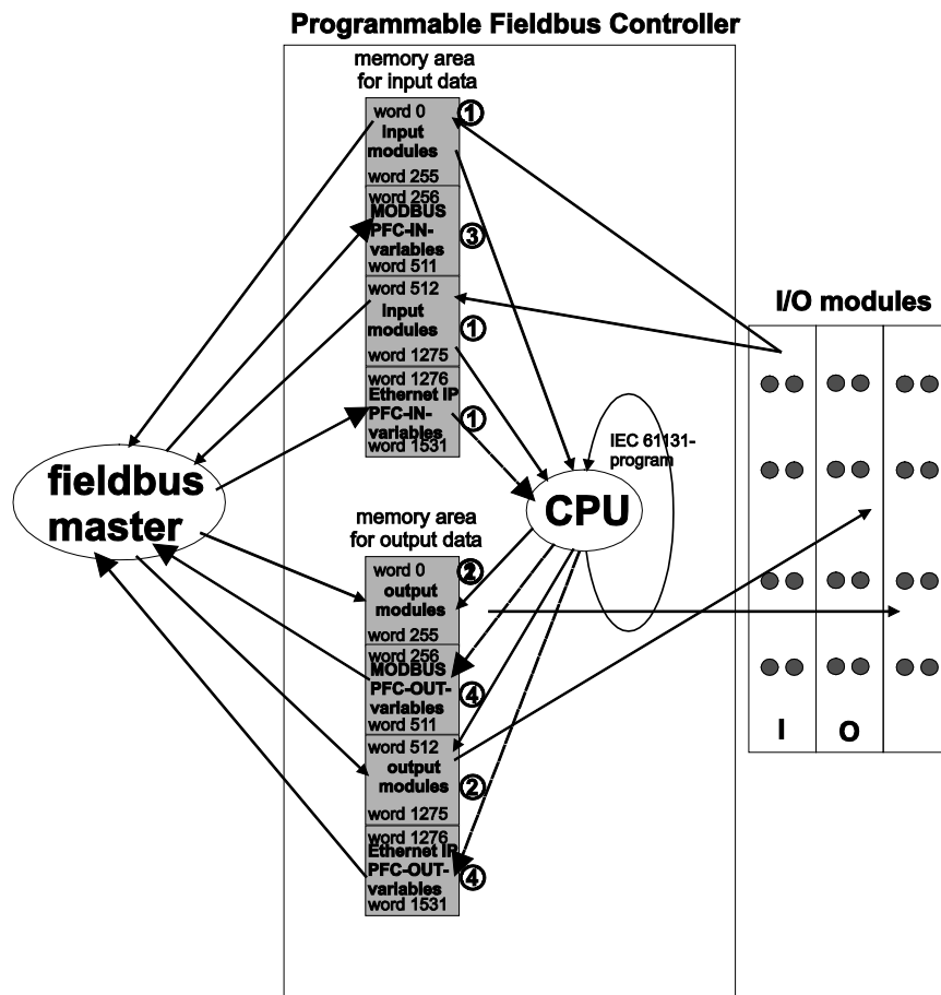
Figure 41: Memory areas and data exchange
