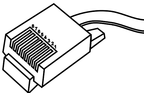
Figure 25: RJ-45 Connector
