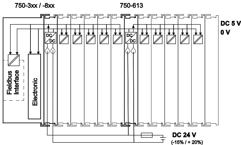
Figure 7: System Voltage for Standard Couplers/Controllers and Extended ECO Couplers
