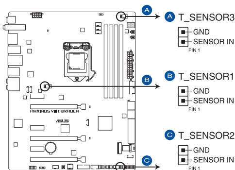
MAXIMUS VIII FORMULA T_SENSOR connectors
