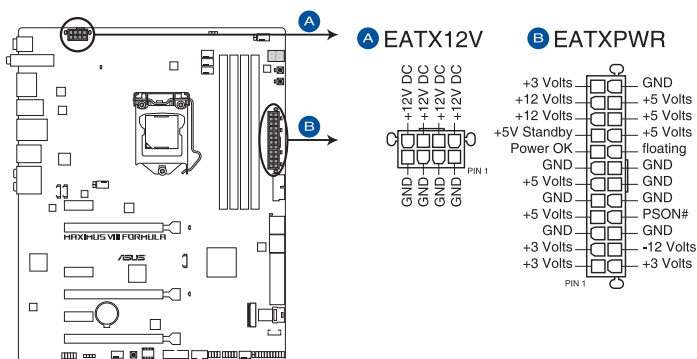
MAXIMUS VIII FORMULA ATX power connectors
