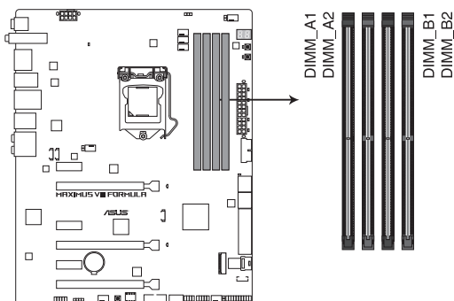
MAXIMUS VIII FORMULA 288-pin DDR4 DIMM socket
