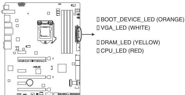
MAXIMUS VIII FORMULA CPU/ DRAM/ BOOT_DEVICE/ VGA LED
