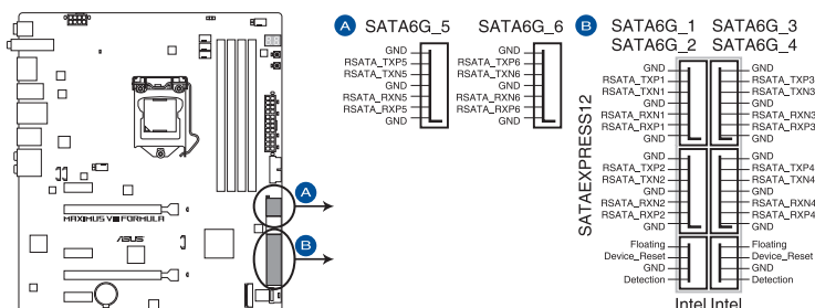
MAXIMUS VIII FORMULA Intel® SATA 6 Gb/s connectors
