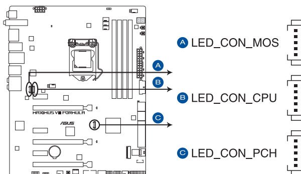
MAXIMUS VIII FORMULA LED connectors
