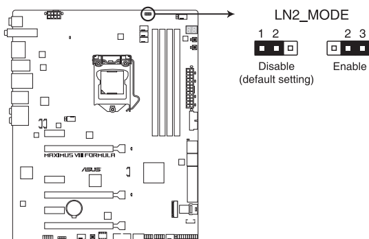
MAXIMUS VIII FORMULA LN2_MODE setting
