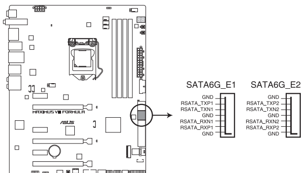
MAXIMUS VIII FORMULA ASMedia® SATA 6 Gb/s connectors
