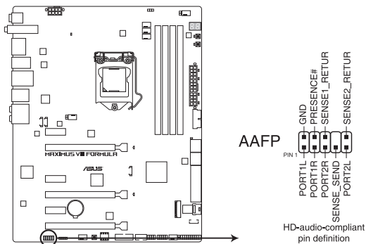
MAXIMUS VIII FORMULA Analog front panel connector
