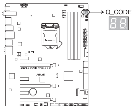
MAXIMUS VIII FORMULA Q-Code LED
