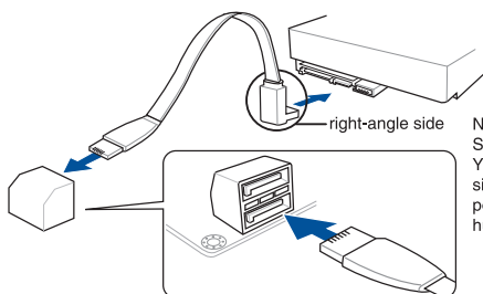
MAXIMUS VIII FORMULA Intel® SATA 6 Gb/s connectors
