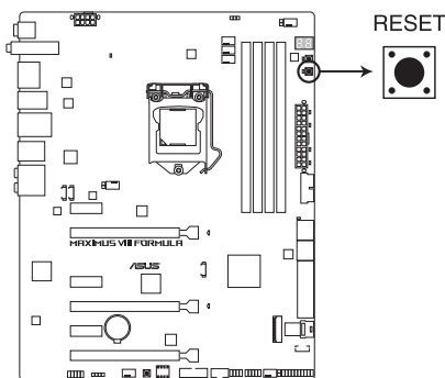
MAXIMUS VIII FORMULA RESET button
