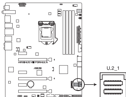
MAXIMUS VIII FORMULA U.2 connector
