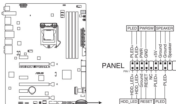
MAXIMUS VIII FORMULA System panel connector
