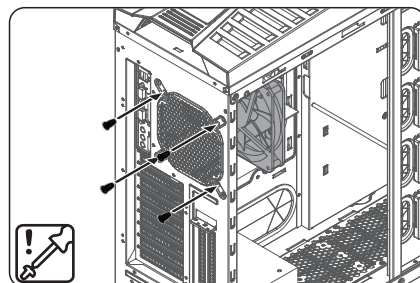
2.7.3 Install rear fan (1 x 120/140mm fan)
