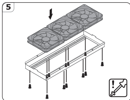
2.7.2 Install top fan (2 x 120/140mm fans or 1 x 200mm fan)
