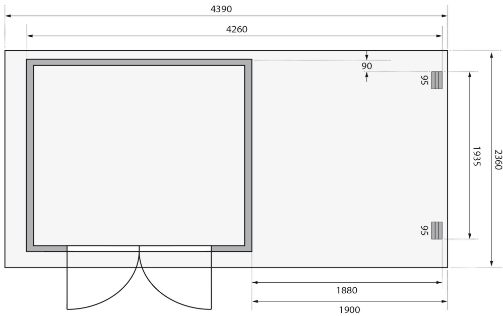
Fundamentplan (in mm)
