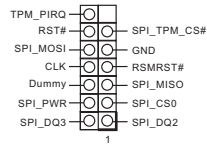
SPI_TPM_J1
