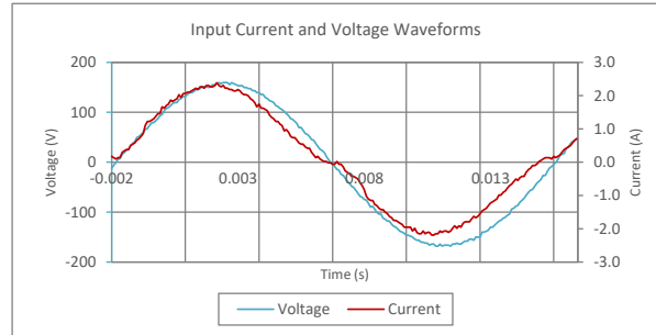
Input AC Current Waveform (ITHD = 10.58%, 50% Load)
