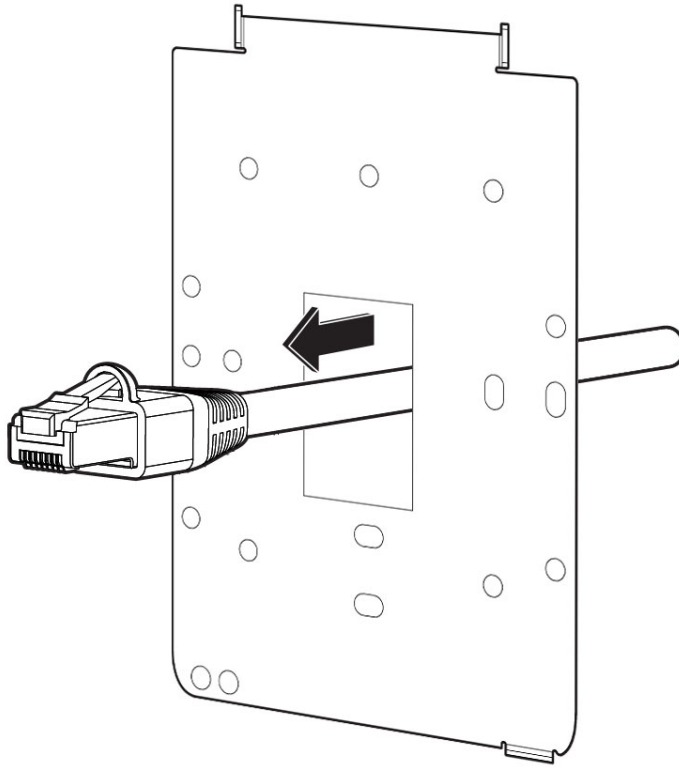
Figure 4: CW-MNT-H1 or MA-MNT-MR-H1A: Routing the passthrough cable from the back
