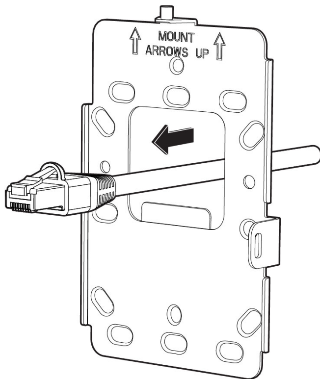
Figure 5: AIR-AP-BRACKET-W4: Routing the passthrough cable from the back
