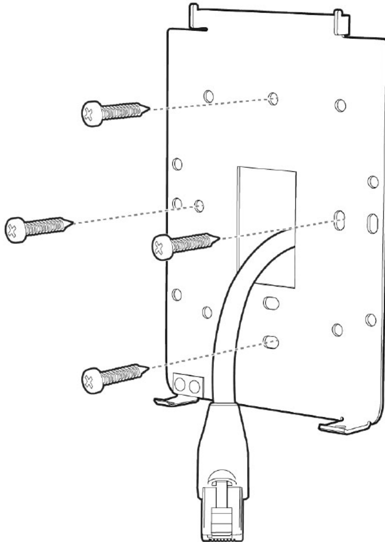
Figure 6: Fasten CW-MNT-H1 or MA-MNT-MR-H1A to the wall
