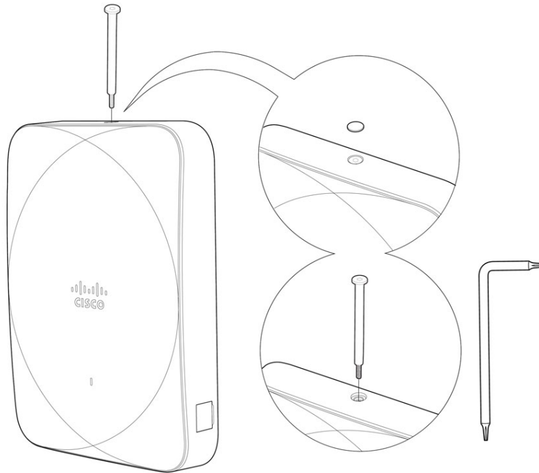
Figure 11: Secure AP to AIR-AP-BRACKET-W4
