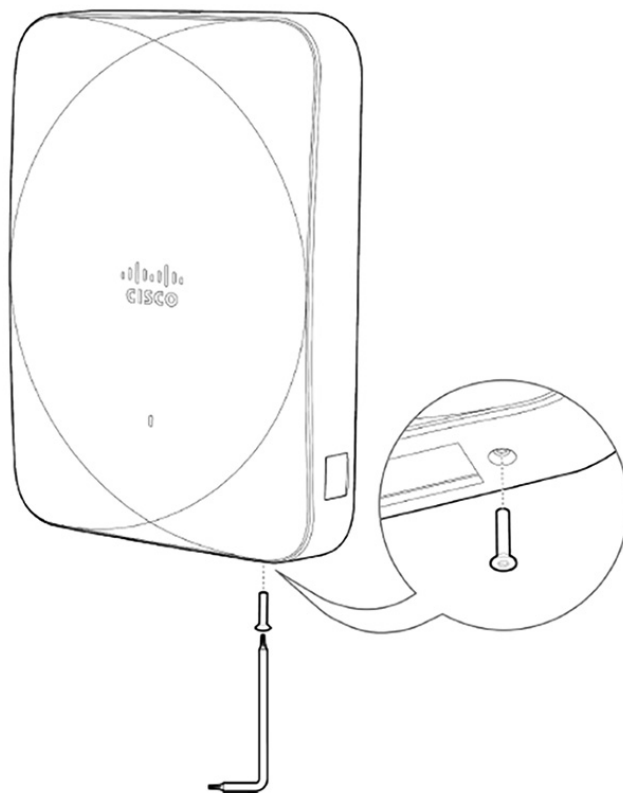
Figure 10: Secure AP to CW-MNT-H1 or MA-MNT-MR-H1A
