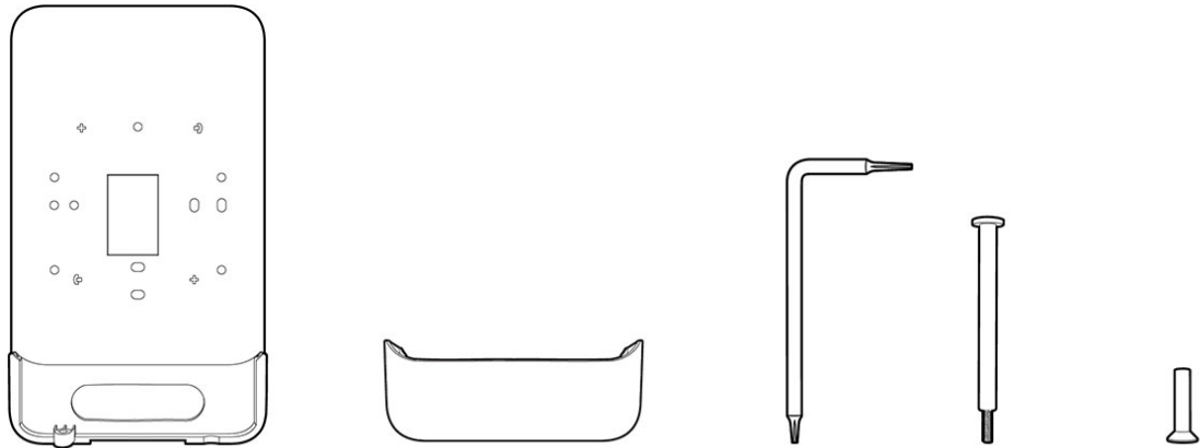
Figure 13: Port lock accessory (CW-MNT-H3-00) kit contents
