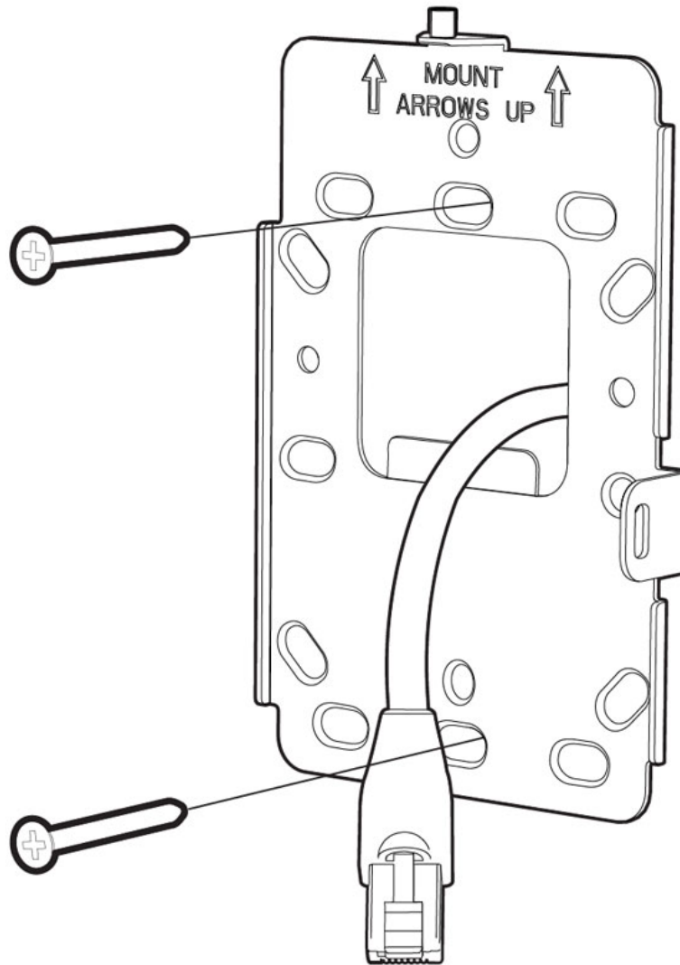
Figure 7: Fasten AIR-AP-BRACKET-W4 to the wall
