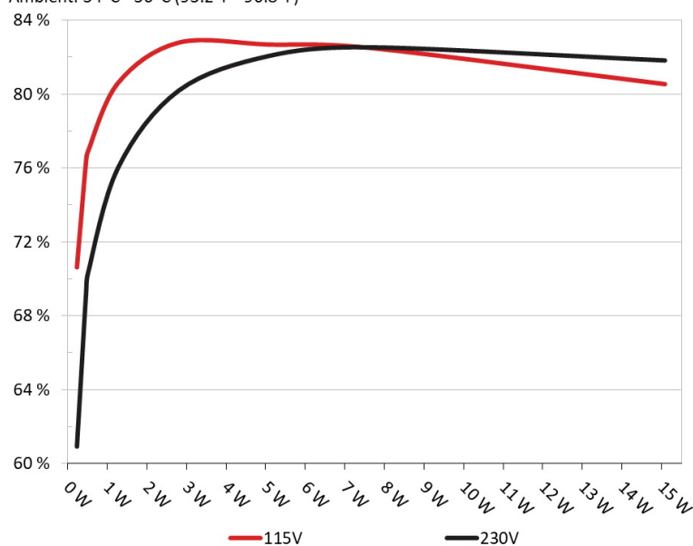
5VSB Efficiency: Cooler Master XG Plus 850 Platinum
