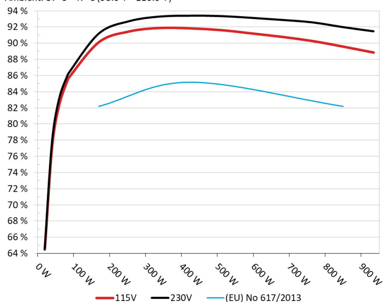
Efficiency: Cooler Master XG Plus 850 Platinum
