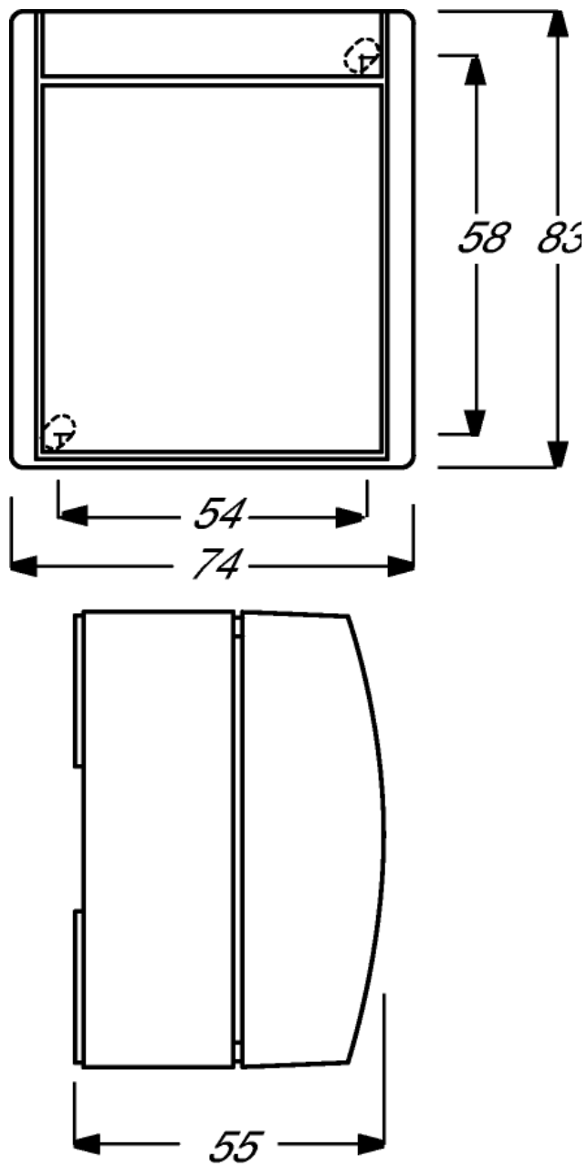
ocean® 1gang box with drilling dimensions
