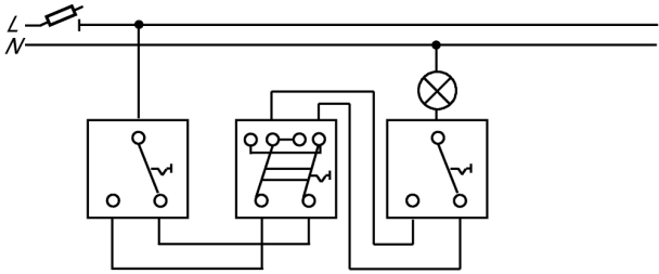
1gang 2way with 1gang intermediate and 1gang 2way
