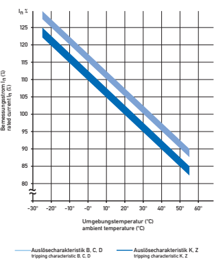
Diagramm Derating
