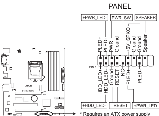
B150M-PLUS System panel connector
