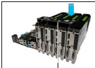
4-Way SLI bridge
