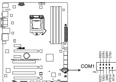
P8Z77-V PRO/THUNDERBOLT Serial port connector
