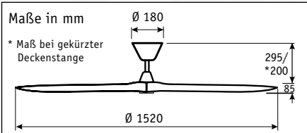
ECO AIRSCREW 152
