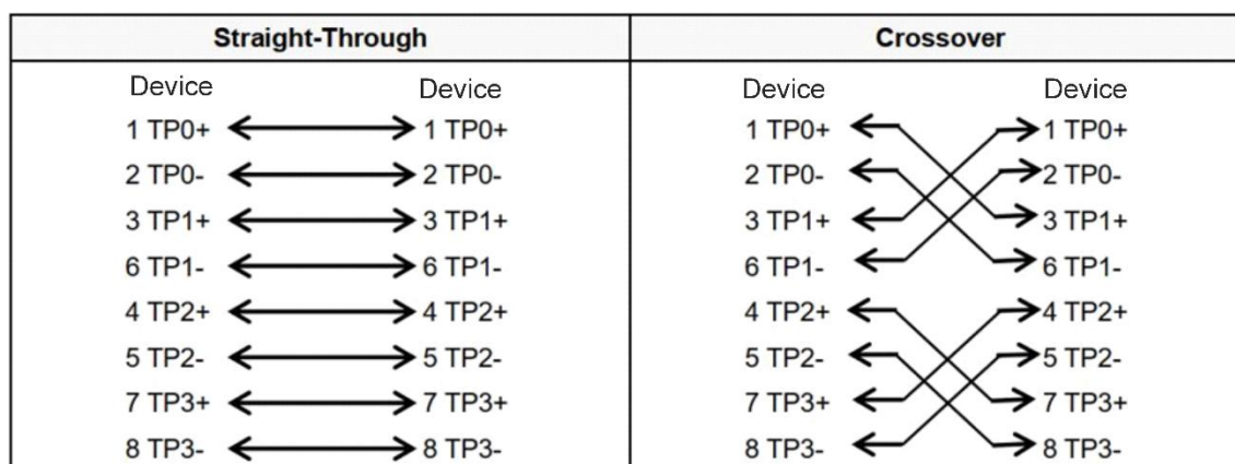
Figure 6-1 2500BASE-T/1000BASE-T Connection
