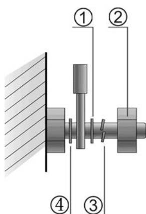
Figure 6-7 Cable Fastening
