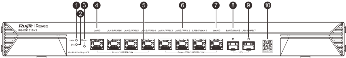
Figure 1-2 Front Panel of RG-EG1510XS
