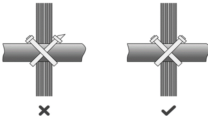
Figure 6-5 Bundling Cables (2)
