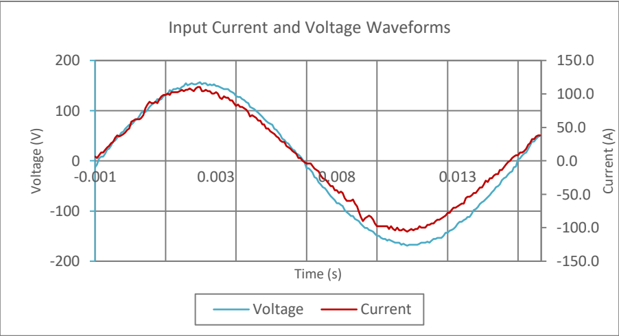
Input AC Current Waveform (ITHD = 4.86%, 50% Load)
