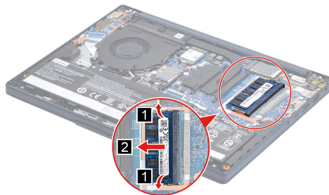
Figure 11. Remove the memory module (14-inch models/15-inch models)
