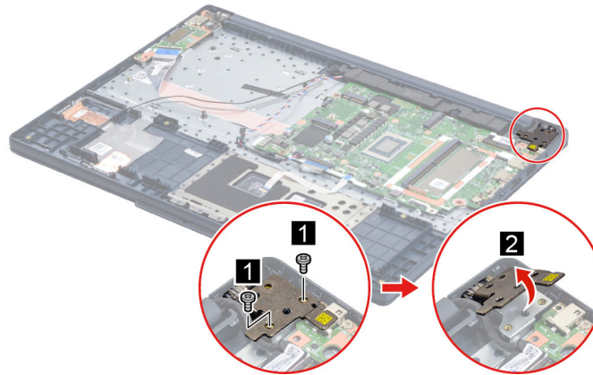
Figure 35. Remove two screws and flip the hinge
