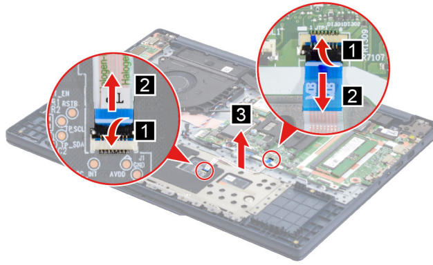
Figure 16. Remove the touchpad cable
