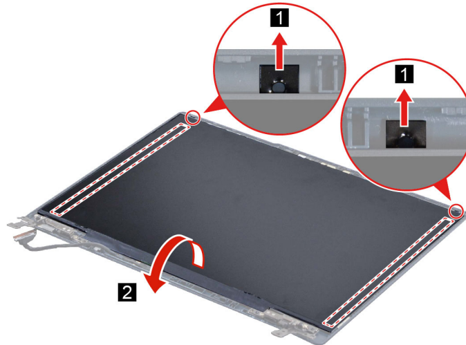
Figure 45. Remove the removable tape and turn over the panel
