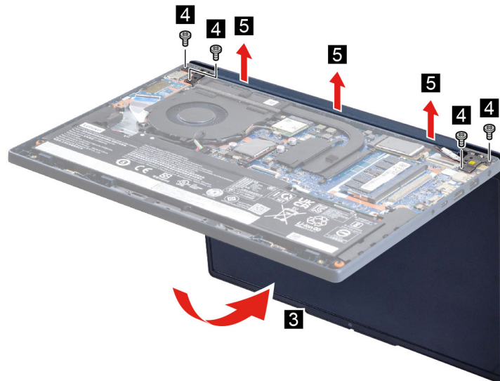
Figure 40. Remove the display assembly (14-inch models)
