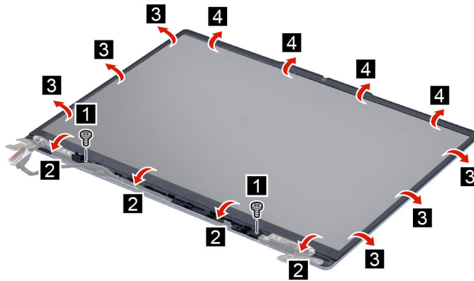
Figure 44. Remove the panel bezel
