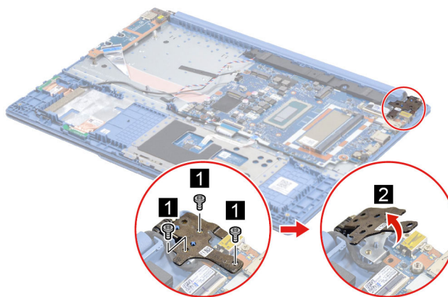
Figure 31. Remove three screws and flip the hinge
