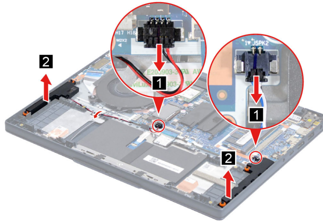
Figure 17. Remove the speaker (14-inch models)
