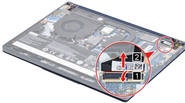
Figure 39. Disconnect the EDP cable from the system board
