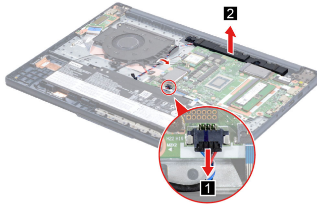
Figure 18. Remove the speaker (15-inch models/16-inch models)
