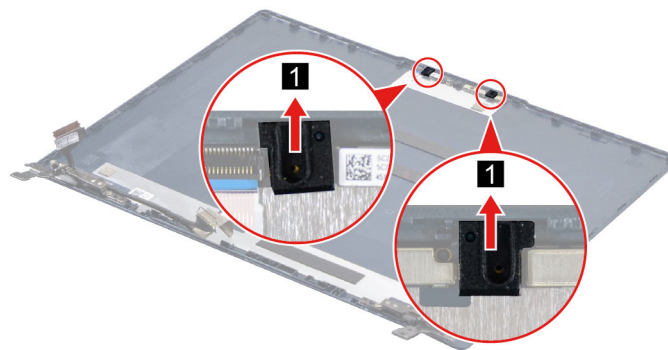
Figure 49. Remove the microphone rubbers
