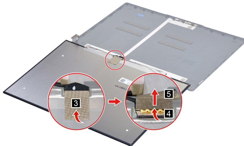
Figure 46. Remove the panel
