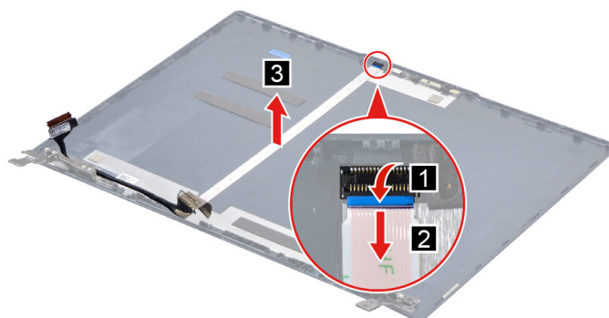
Figure 50. Remove the EDP cable
