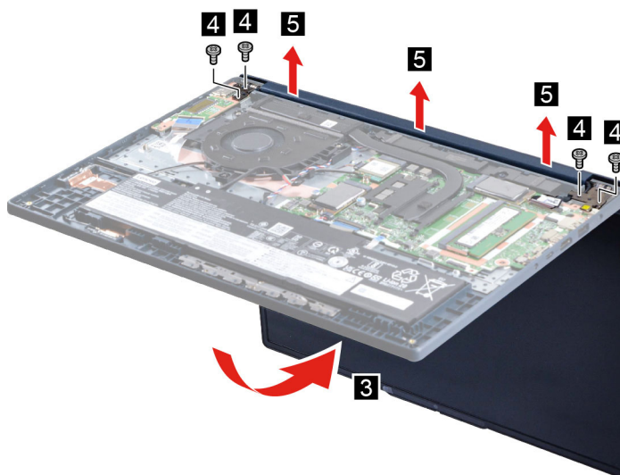
Figure 42. Remove the display assembly (16-inch models)
