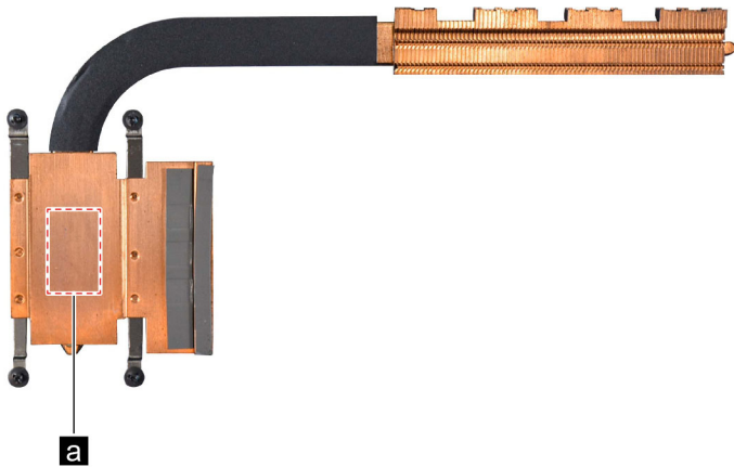
Figure 20. Areas on the heat sink where thermal interface materials should be applied
