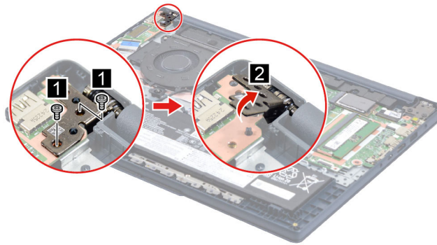
Figure 25. Flip the hinge (15-inch models/16-inch models)
