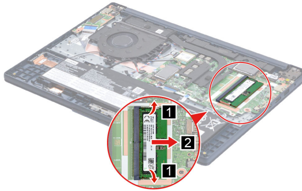
Figure 12. Remove the memory module (16-inch models)
