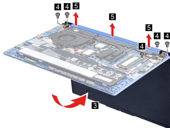
Figure 41. Remove the display assembly (15-inch models)
