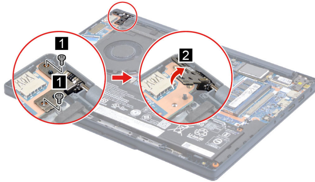
Figure 24. Flip the hinge (14-inch models)
