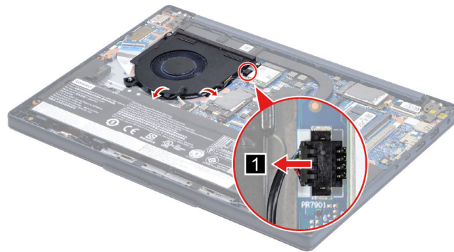
Figure 22. Disconnect the fan cable
