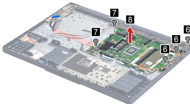
Figure 37. Remove the system board
