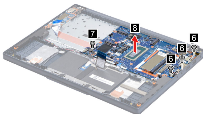
Figure 29. Remove the system board
