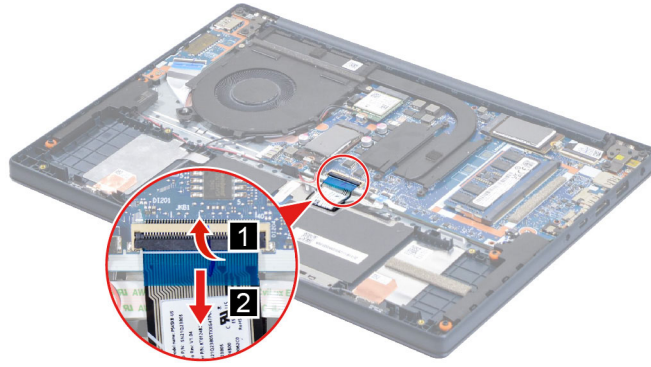
Figure 14. Disconnect the keyboard cable
