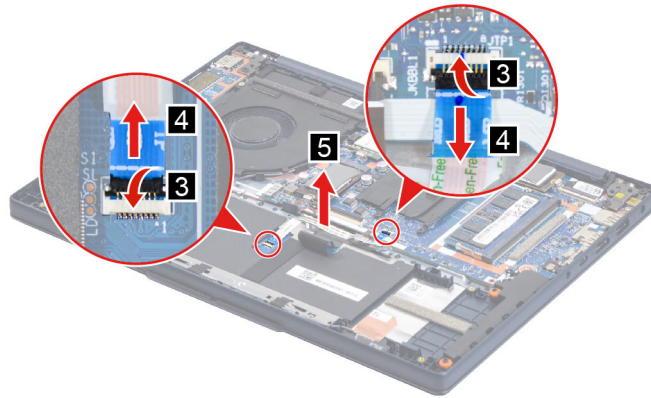
Figure 15. Remove the touchpad cable
