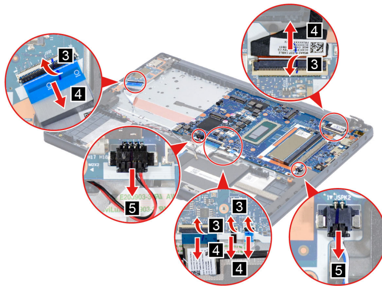
Figure 28. Disconnect cables connected to the system board
