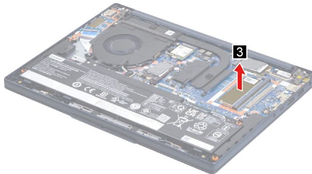
Figure 13. Remove the DDR absorber
