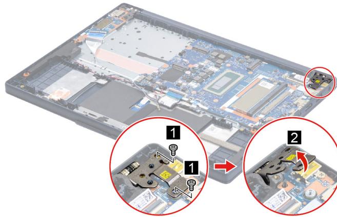
Figure 27. Remove two screws and flip the hinge
