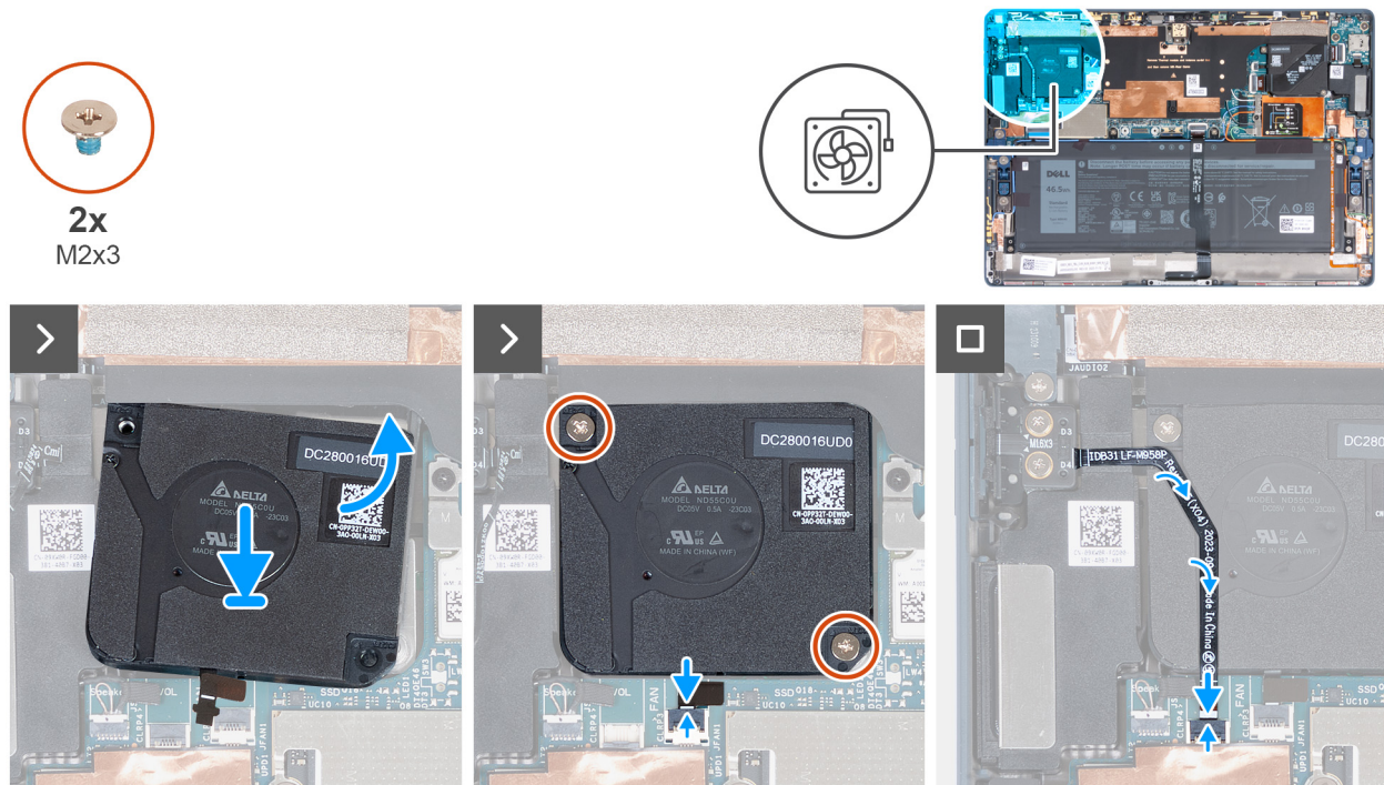
Figure 35. Installing the left fan
