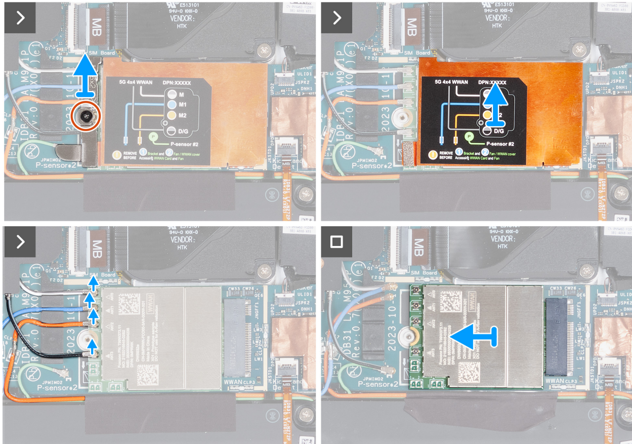
Figure 31. Removing the WWAN card
