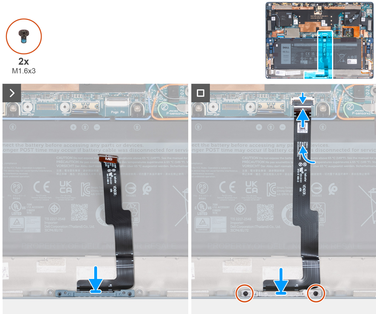
Figure 27. Installing the docking connector
