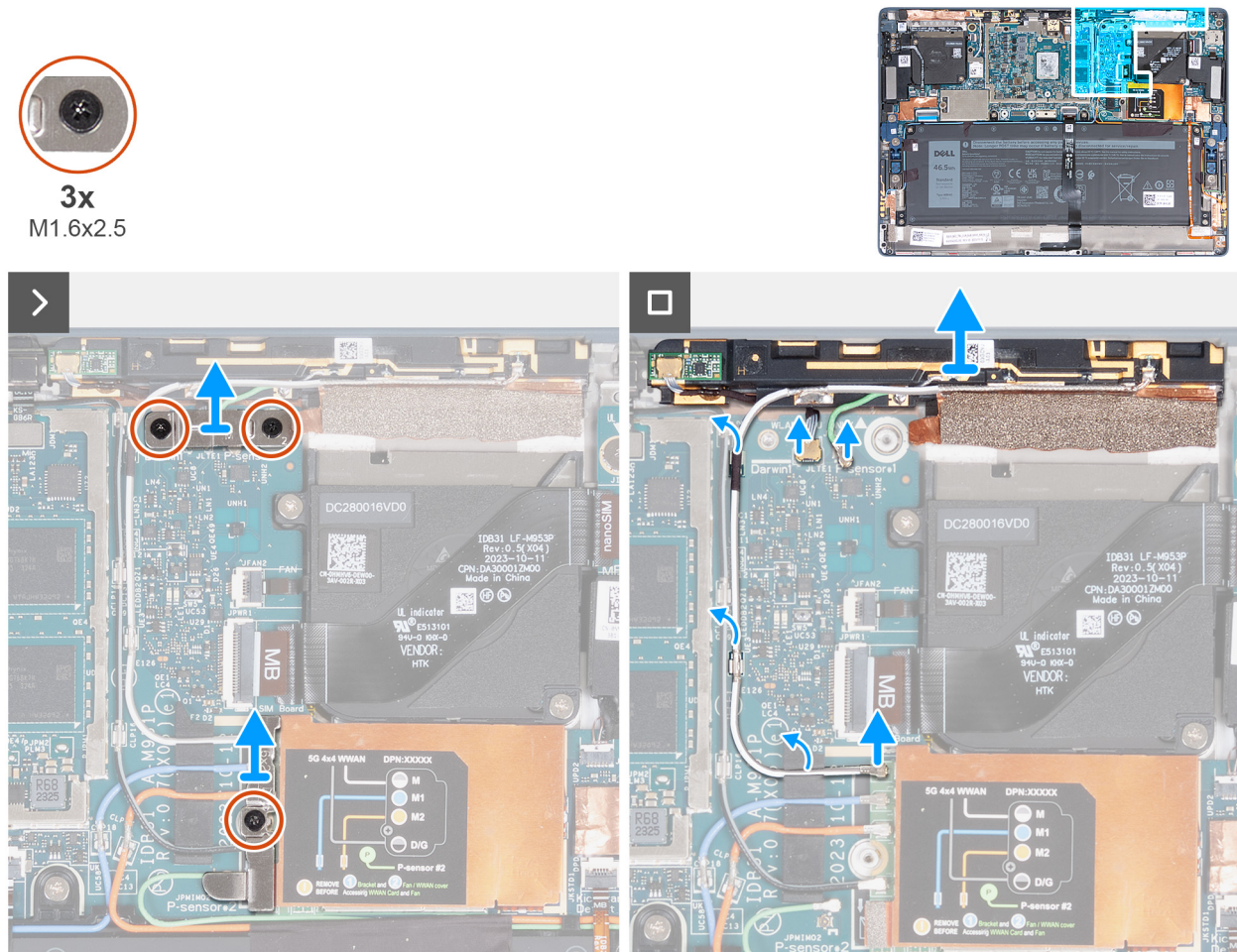
Figure 59. Removing the WWAN-antenna module
