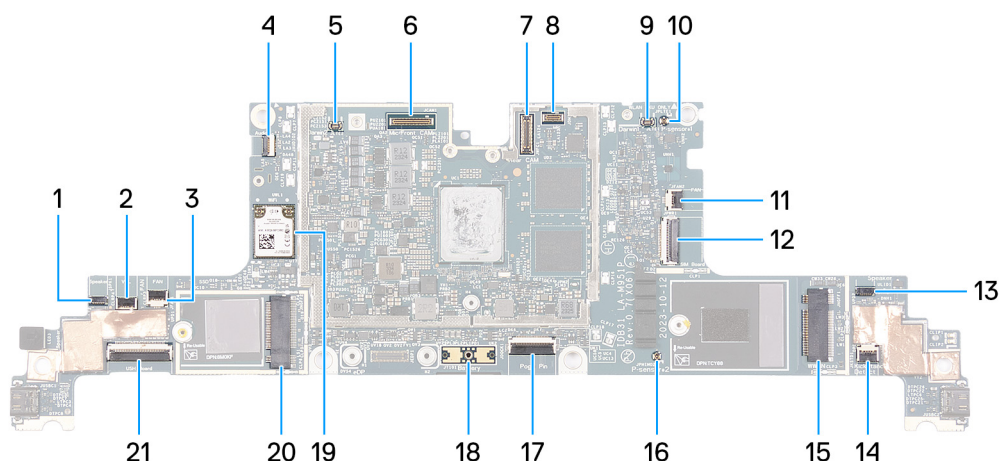
Figure 70. System-board connectors
