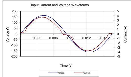
Input AC Current Waveform (ITHD = 11.47%, 50% Load)
