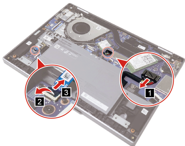
Figure 13. Disconnect cables
