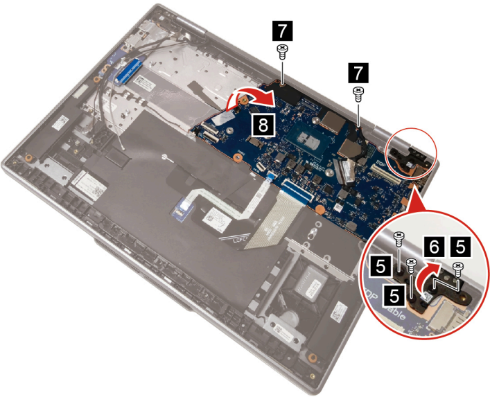
Figure 29. Remove the system board with USB board cable
