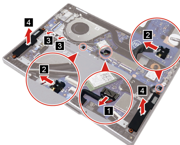
Figure 9. Disconnect and remove the speakers
