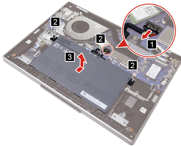
Figure 5. Loosen three screws and the battery pack
