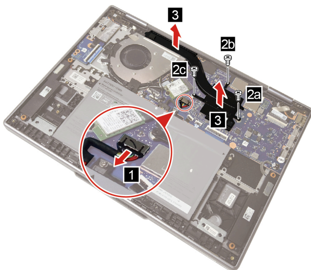
Figure 8. Remove the heat sink
