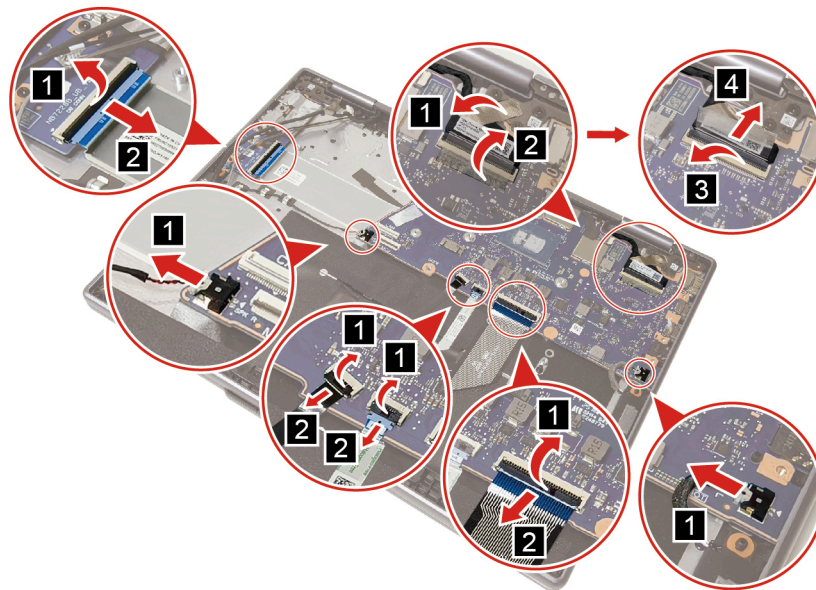
Figure 28. Disconnect all cables
