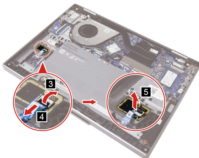
Figure 11. Disconnect the fingerprint reader board cable and remove the fingerprint reader board
