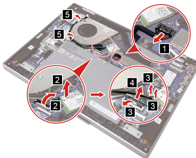
Figure 6. Disconnect and pull out cables
