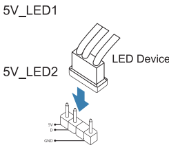
Addressable RGB LED Device Header (5V_LED)
