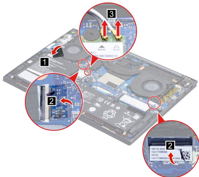
Figure 29. Peel off the tape, the mylar and detach the antenna cables
