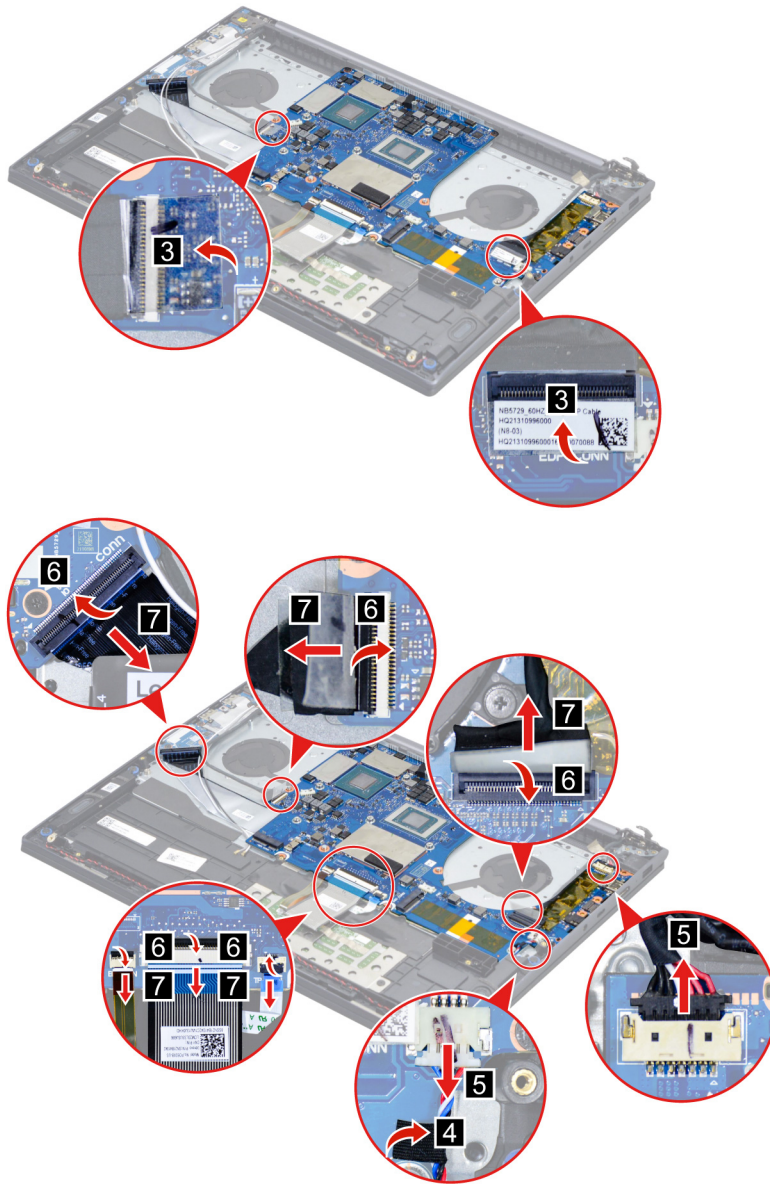
Figure 26. Disconnect cables connected to the system board and disconnect the I/O board cable
