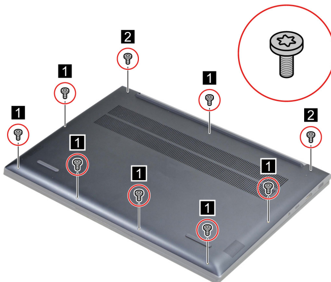
Figure 2. Remove nine screws
