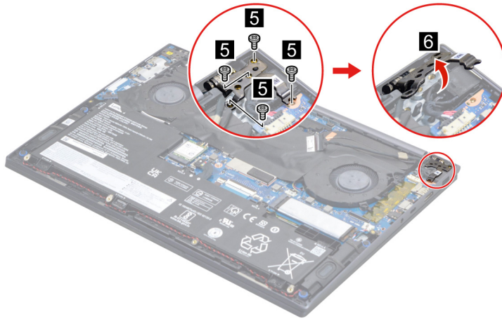
Figure 16. Remove four screws and open the hinge
