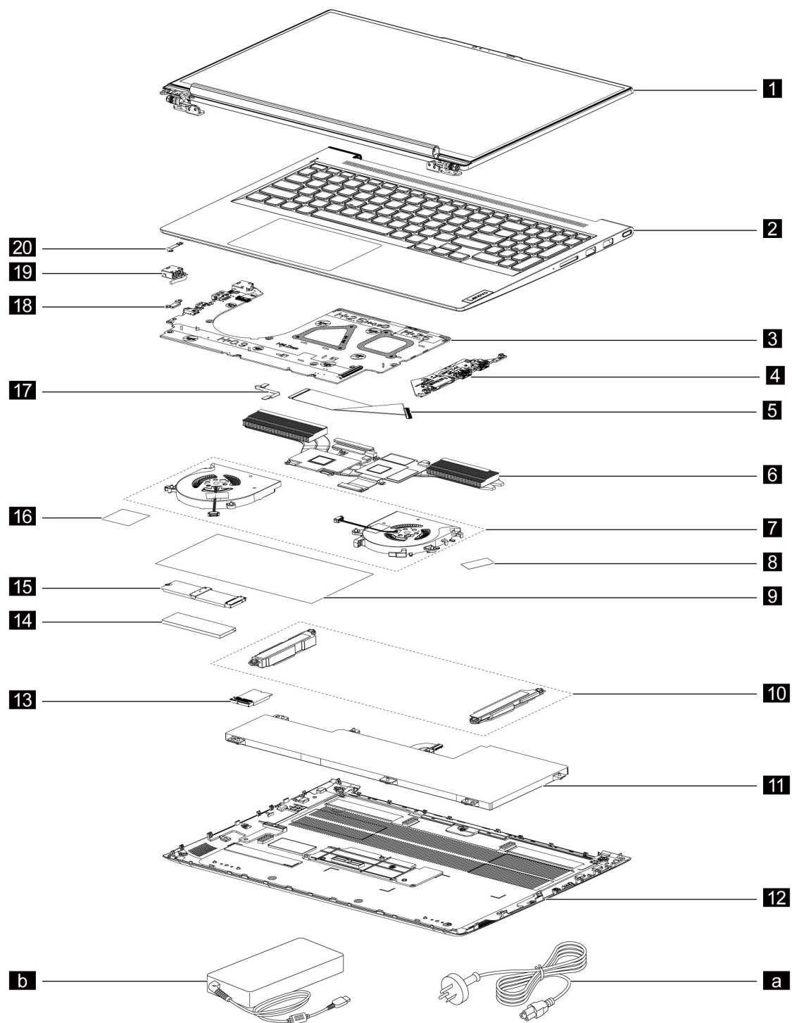
Figure 1. Yoga Slim 7 Pro 16ACH6 exploded view
