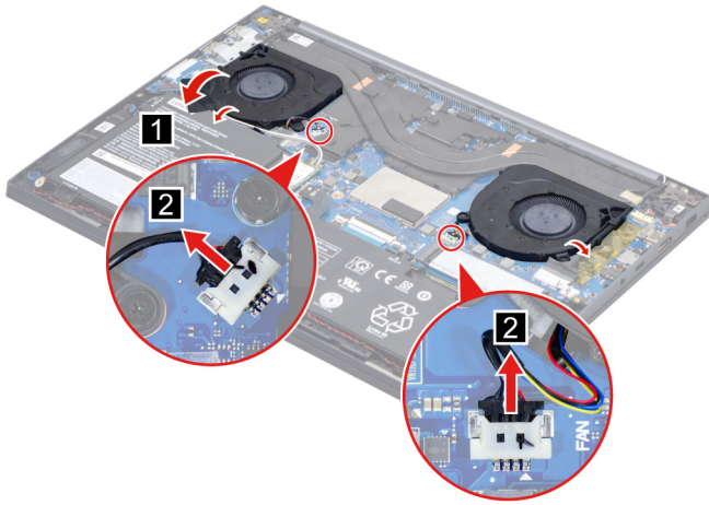
Figure 21. Disconnect the fan cables and then release the cables
