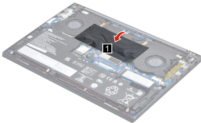
Figure 18. Peel off the D cover mylar
