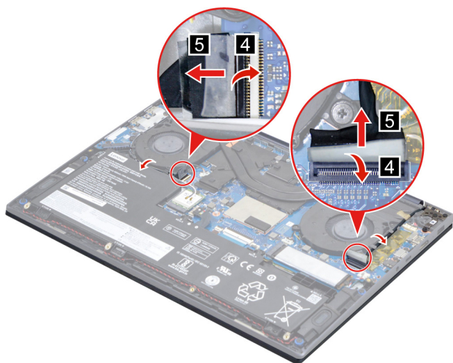
Figure 30. Disconnect the sensor cable and the EDP cable and release the cables
