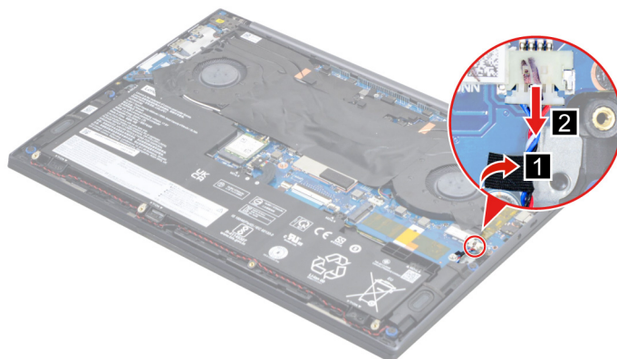
Figure 8. Disconnect the speaker cable from the system board
