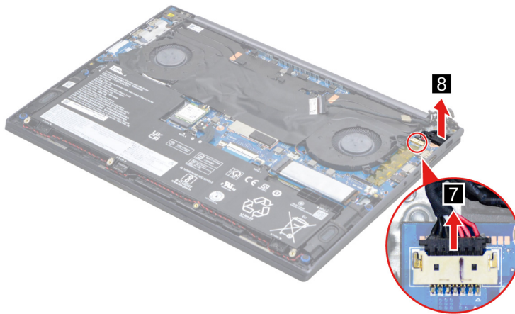
Figure 17. Remove the DC-in cable
