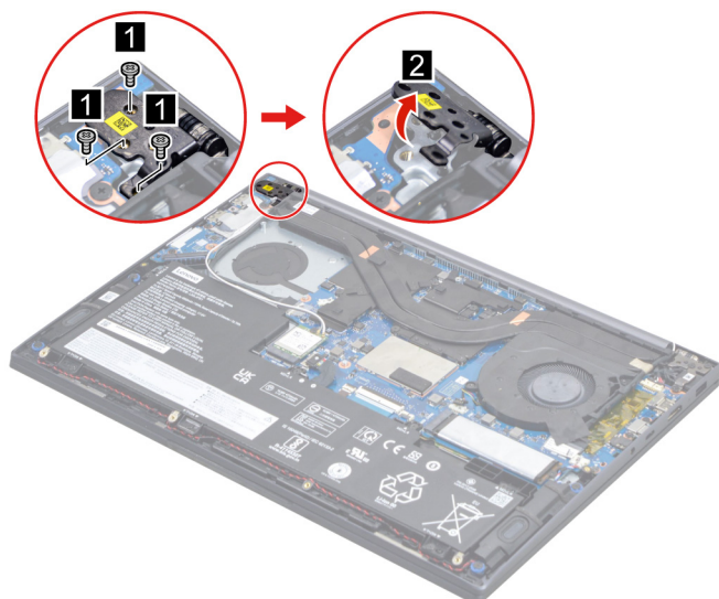
Figure 23. Remove three screws and open the hinge
