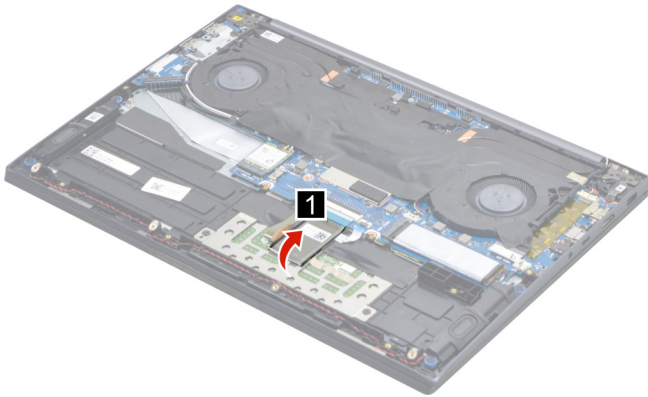
Figure 11. Peel back the tape
