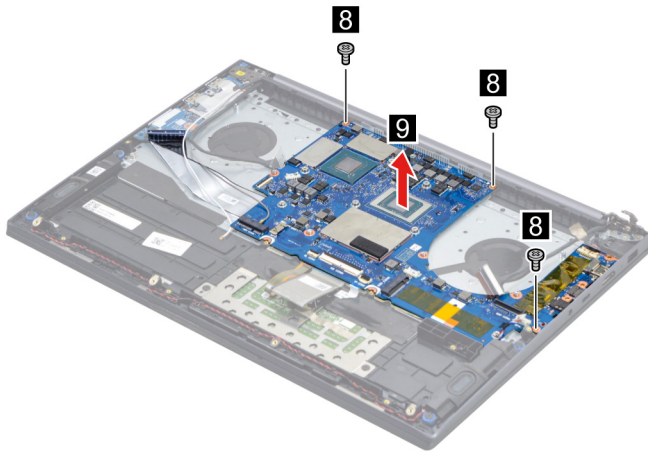
Figure 27. Remove the system board with the I/O board cable
