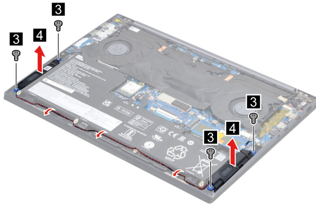
Figure 9. Remove the speakers
