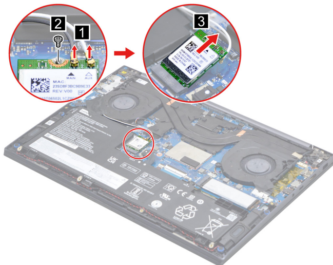
Figure 20. Remove the Wi-Fi card
