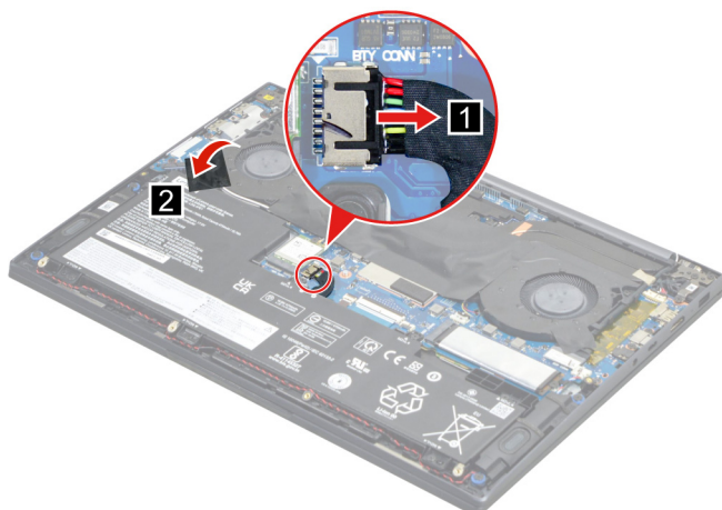
Figure 4. Disconnect the battery pack cable from the system board and peel off the tape
