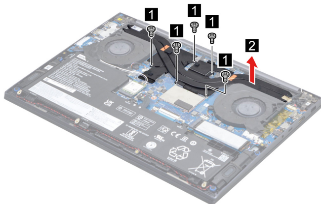
Figure 19. Remove five screws and then remove the heat sink
