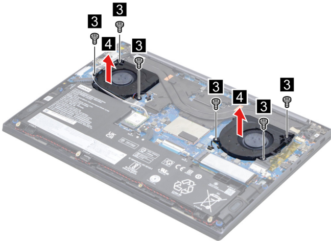
Figure 22. Remove the fans
