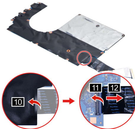
Figure 28. Remove the I/O board cable
