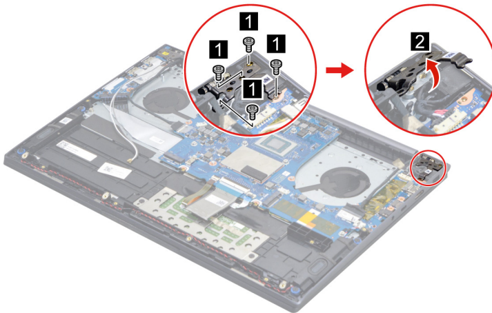
Figure 25. Remove four screws and then open the hinge
