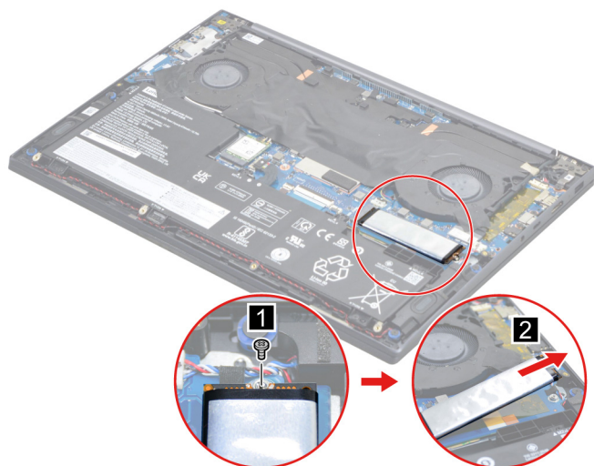
Figure 6. Remove the SSD module by pulling it away from the slot
