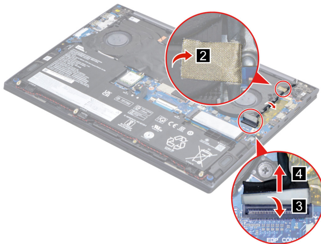
Figure 15. Release the EDP cable from the cable guide
