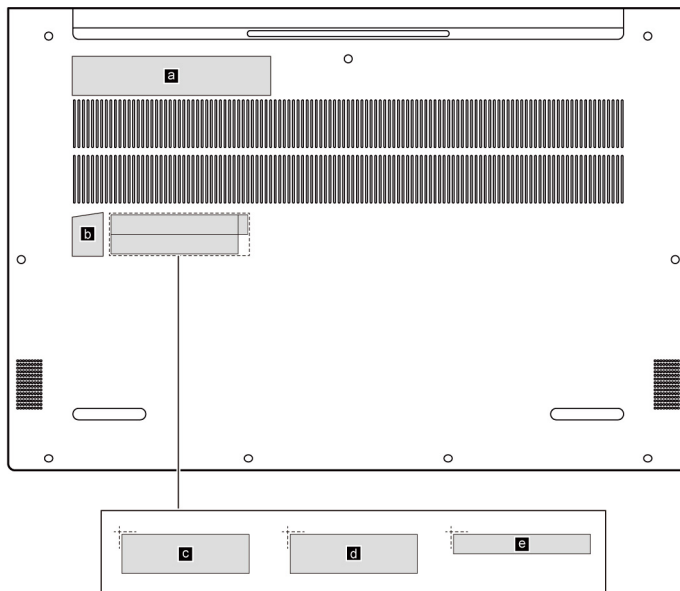
Figure 32. Label layout on the back side of the base cover
