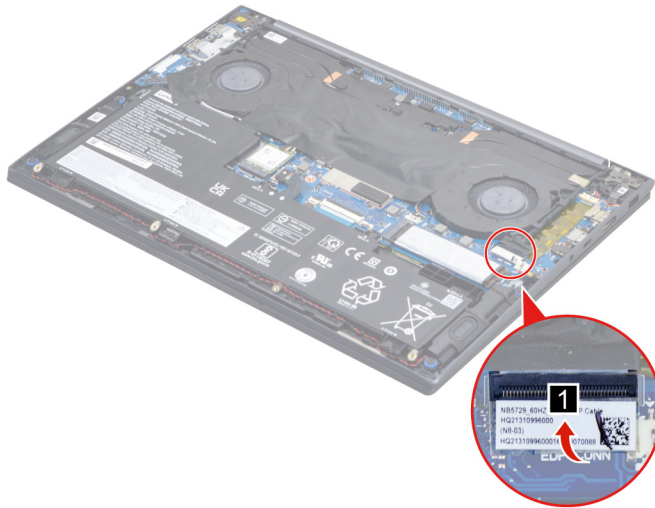
Figure 14. Peel off the mylar
