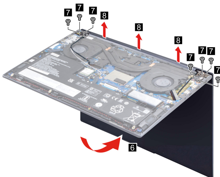
Figure 31. Remove the LCD module
