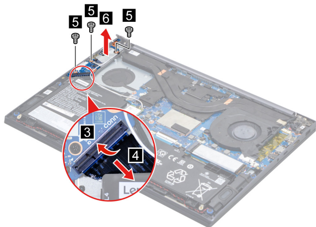
Figure 24. Remove the I/O board
