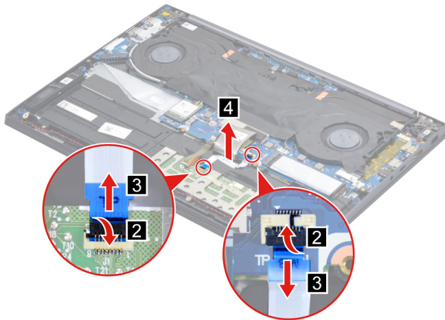
Figure 12. Remove the touchpad cable
