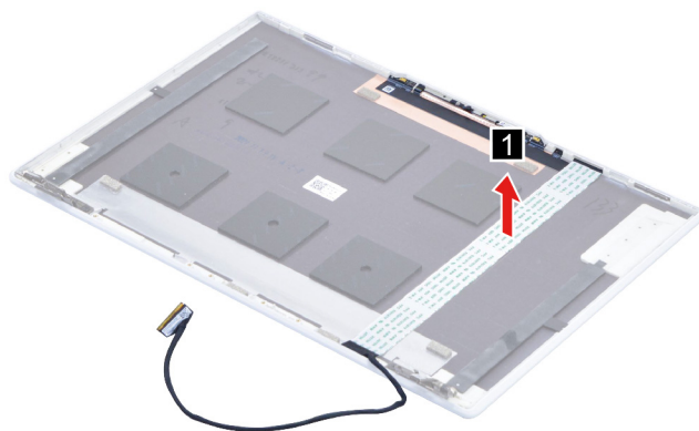
Figure 36. Remove camera with camera cable from LCD cover
