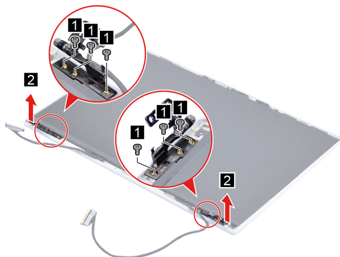
Figure 30. Remove six screws and remove the hinges
