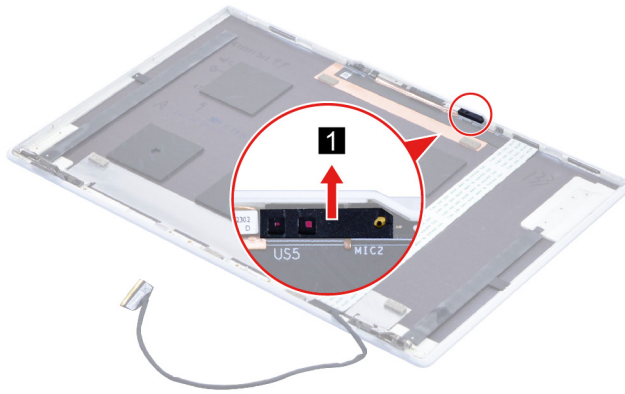
Figure 35. Remove the ToF rubber
