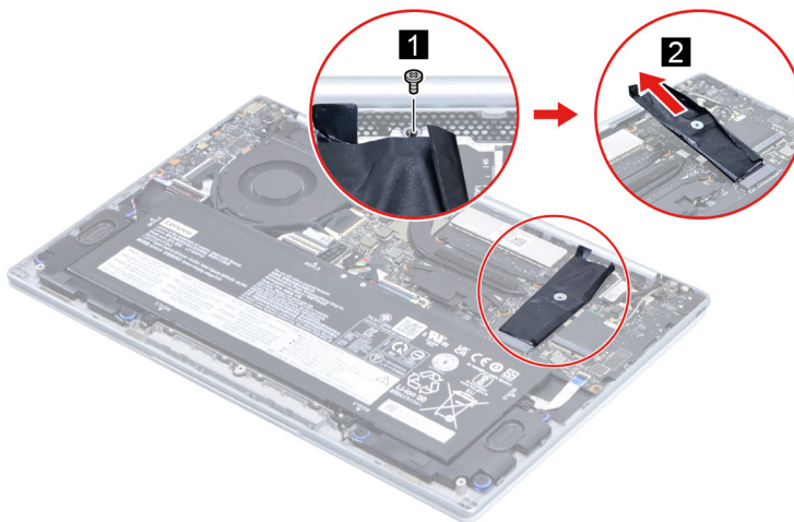
Figure 7. Remove the SSD with SSD bracket
