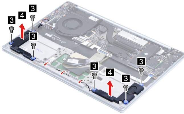
Figure 20. Remove the six screws and remove the speakers.
