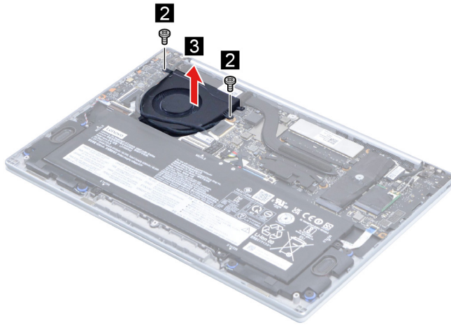
Figure 12. Remove two screws and remove the fan.
