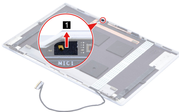
Figure 33. Remove the microphone rubber
