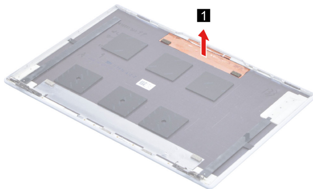
Figure 38. Remove the camera mylar
