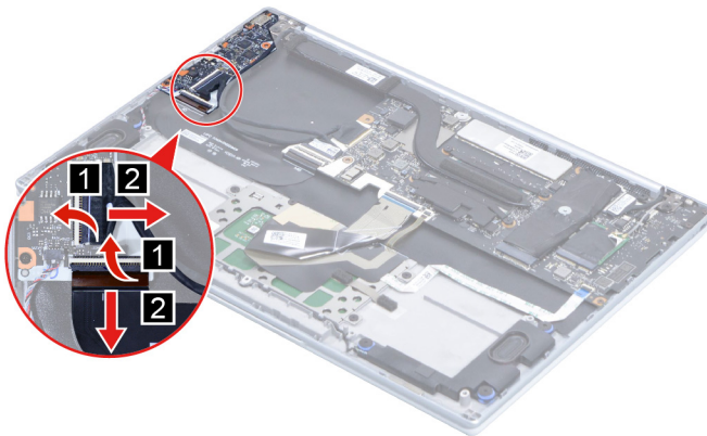
Figure 15. Disconnect cables connected to the I/O board
