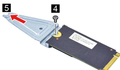
Figure 9. Remove one screw then remove the SSD bracket
