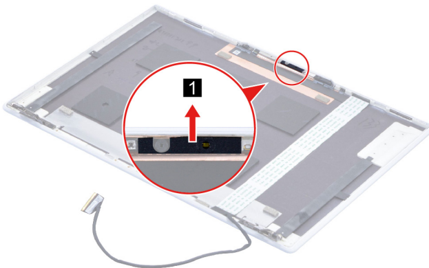
Figure 34. Remove the camera rubber
