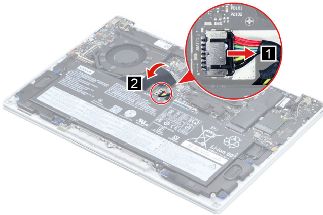
Figure 5. Remove the battery pack cable and peel off the mylar
