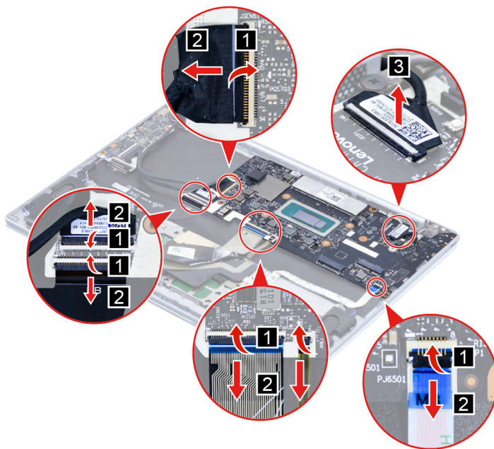
Figure 22. Disconnect cables connected to the system board
