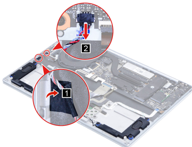
Figure 19. Disconnect the speaker cable from the I/O board
