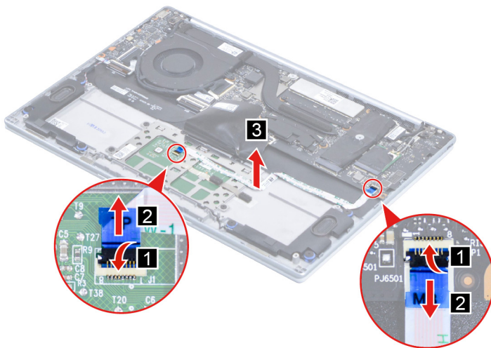
Figure 21. Remove the touchpad board cable
