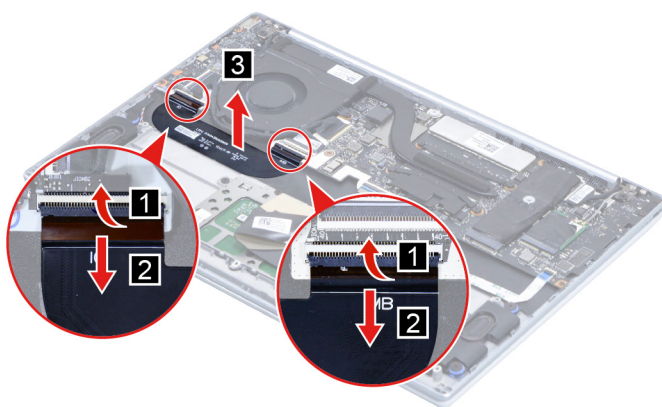
Figure 18. Remove I/O board FPC
