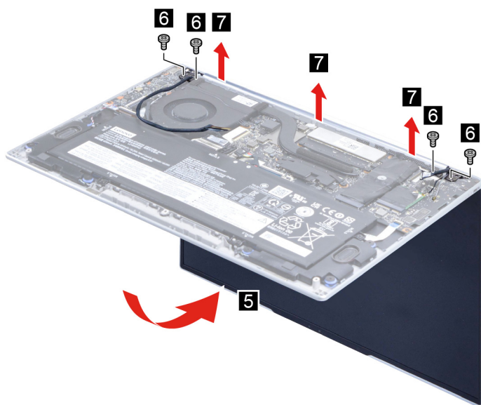
Figure 25. Remove the LCD module
