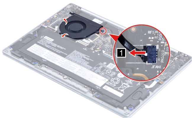
Figure 11. Disconnect the fan cable from the system board
