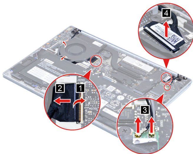
Figure 24. Disconnect the camera board cable, EDP cable and antenna cable
