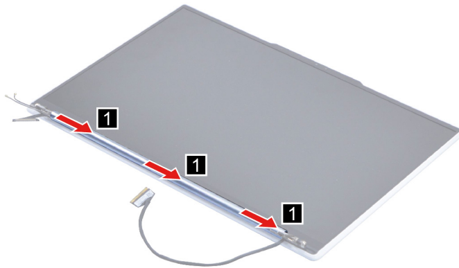
Figure 26. Remove the hinge cover
