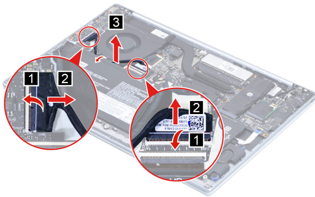
Figure 17. Remove the I/O board cable
