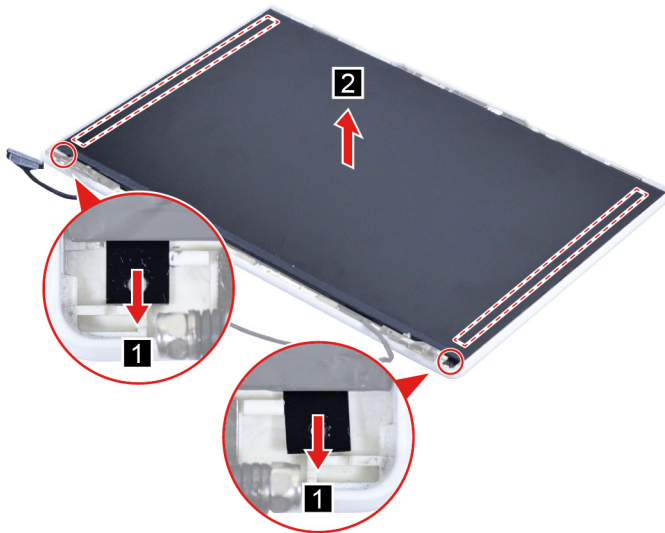
Figure 31. Remove the LCD panel
