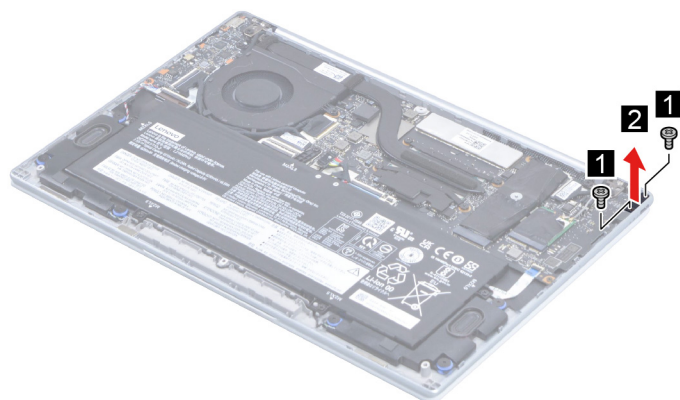
Figure 14. Remove the two screws then remove the Type-C bracket
