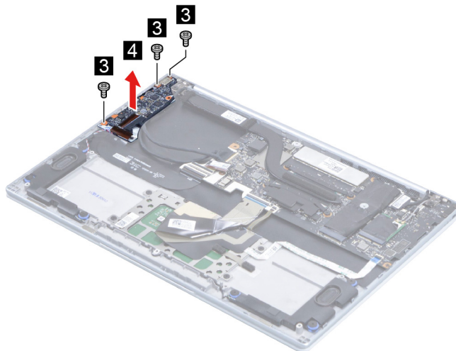
Figure 16. Remove three screws and remove the I/O board
