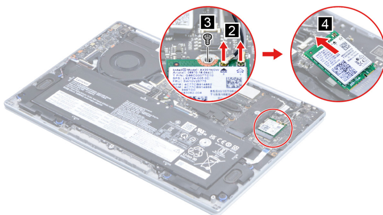
Figure 13. Remove the Wi-Fi card
