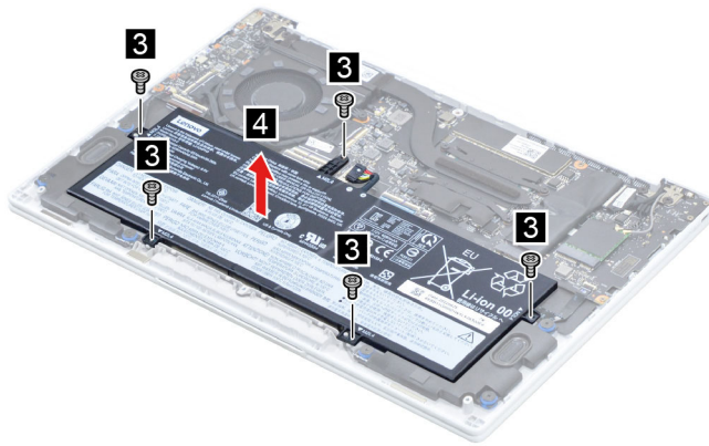
Figure 6. Remove the battery pack
