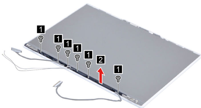
Figure 29. Remove the strip cover
