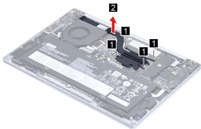
Figure 10. Remove the heat sink
