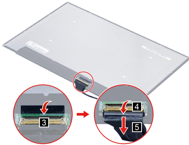
Figure 32. Detach the EDP cable
