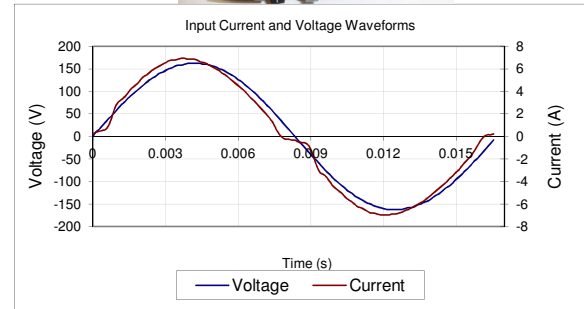
Input AC Current Waveform (ITHD = 8.19%, 50% Load)
