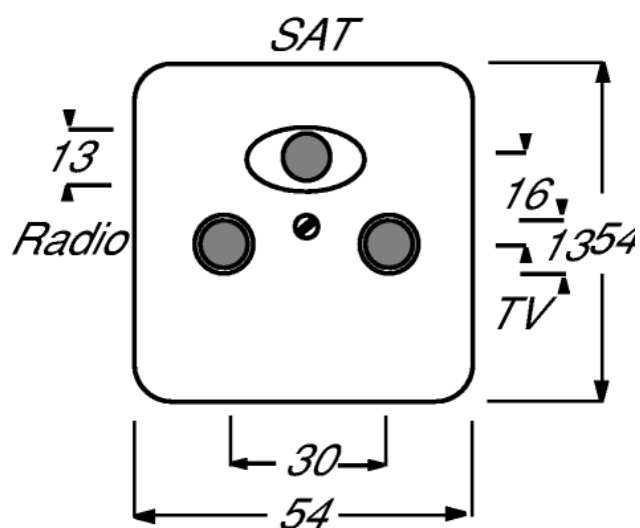
Cover plate with 3 connections for SAT /Audio /TV, 1743-03-...
