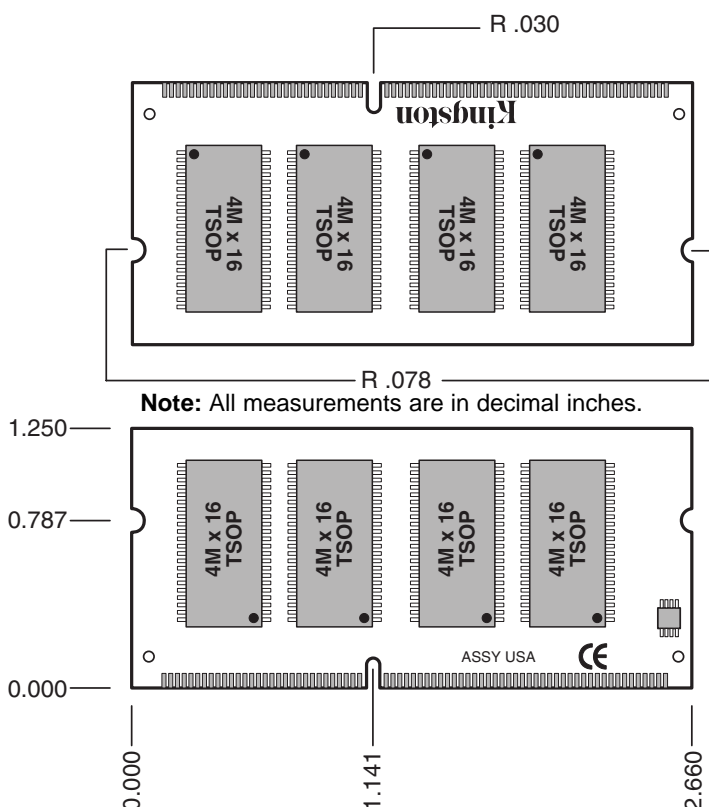
Figure 1: KVR100X64SC3/64 64MB 144-Pin SDRAM Module
