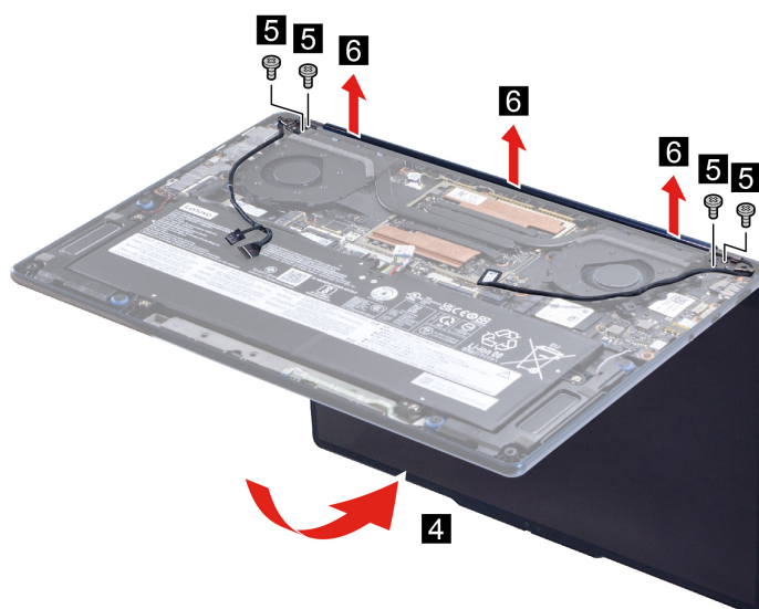
Figure 26. Remove the display assembly
