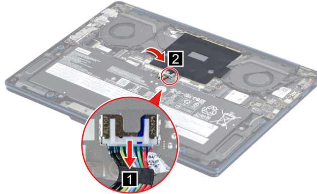
Figure 7. Remove the system board conductive tape
