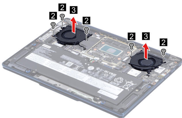
Figure 19. Remove five screws and remove two fans
