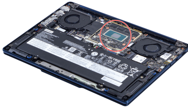
Figure 17. Areas on the system board where thermal interface materials are applied
