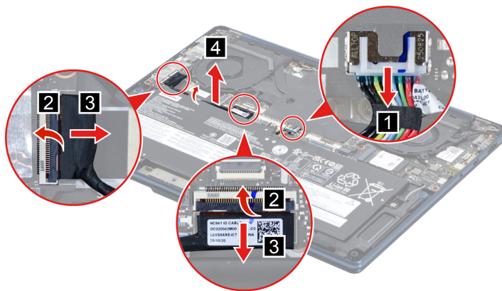
Figure 11. Remove the I/O board cable
