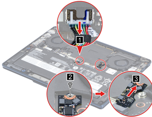
Figure 10. Remove the PMIC board
