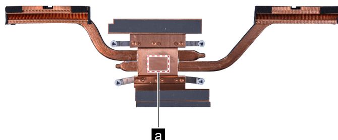
Figure 16. Areas on the heat sink where thermal interface materials should be applied
