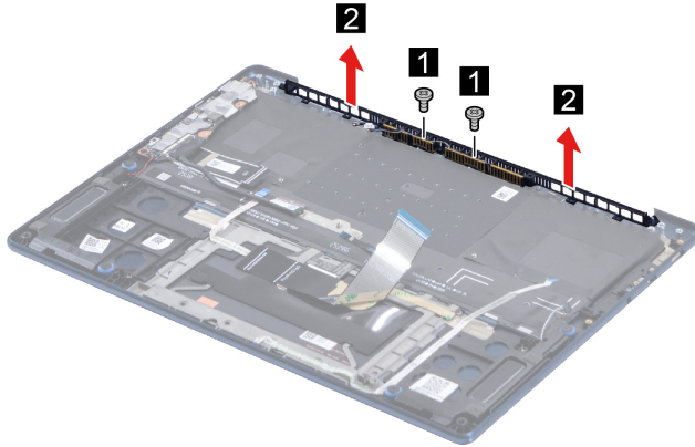
Figure 27. Remove two screws and then remove the antenna
