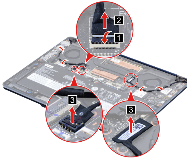
Figure 25. Disconnect the camera cable and EDP cable from the system board
