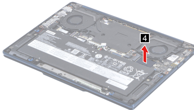
Figure 9. Remove the SSD thermal pad
