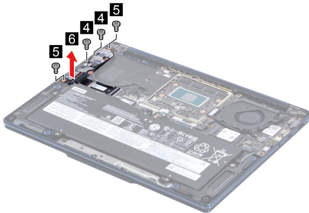
Figure 21. Remove four screws and remove the I/O board
