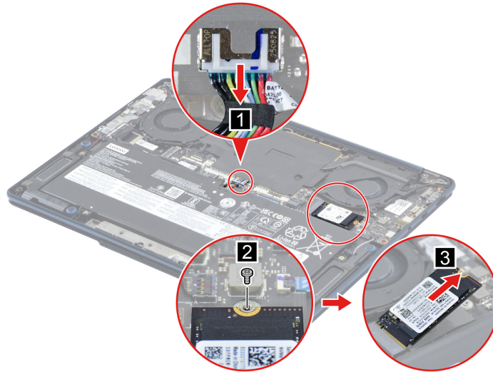
Figure 8. Remove the 2242 solid-state drive
