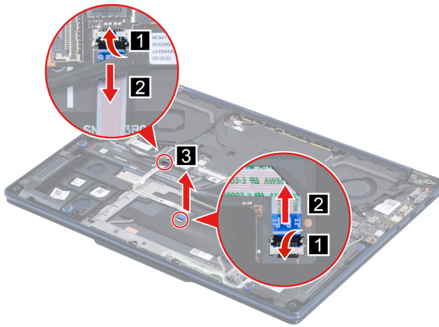
Figure 12. Remove the touchpad cable
