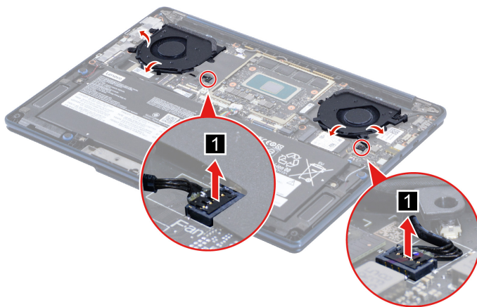
Figure 18. Disconnect two fan cables from the system board
