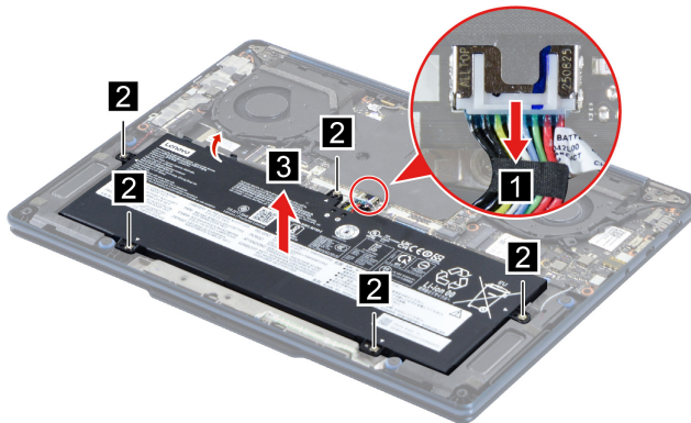
Figure 5. Remove the battery pack
