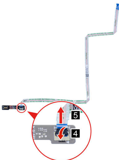
Figure 14. Remove the microphone cable
