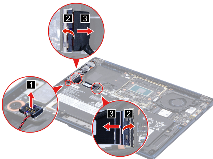
Figure 20. Disconnect the cables
