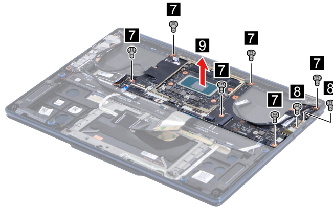
Figure 24. Remove eight screw and remove the system board
