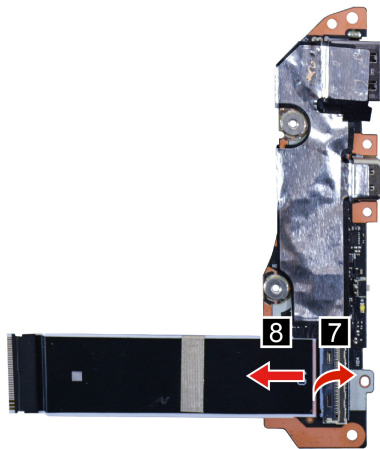
Figure 22. Remove the I/O board FFC
