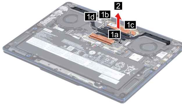
Figure 15. Loosen four screws and remove the heat sink
