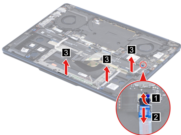
Figure 13. Remove the microphone board
