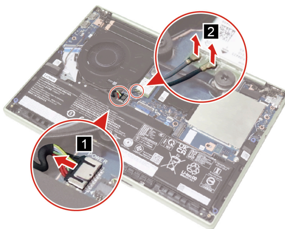
Figure 12. Disconnect the battery pack cable and antennas
