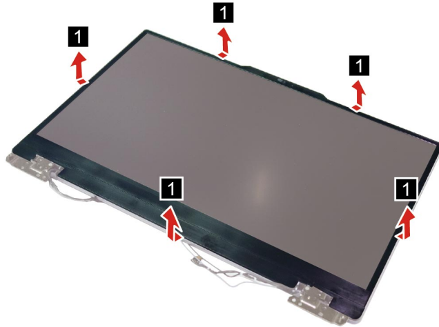
Figure 26. Remove the LCD bezel
