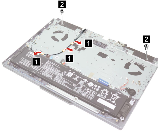
Figure 24. Remove two screws and remove the antennas from the cable guide
