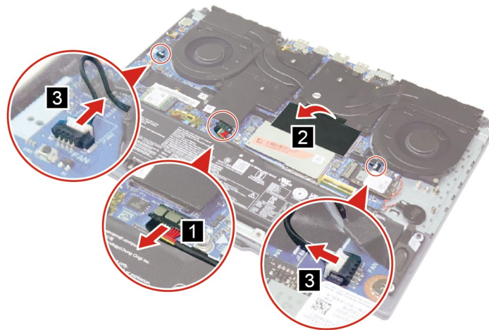
Figure 18. Disconnect the battery pack cable, peel back the mylar, and disconnect the fan cables
