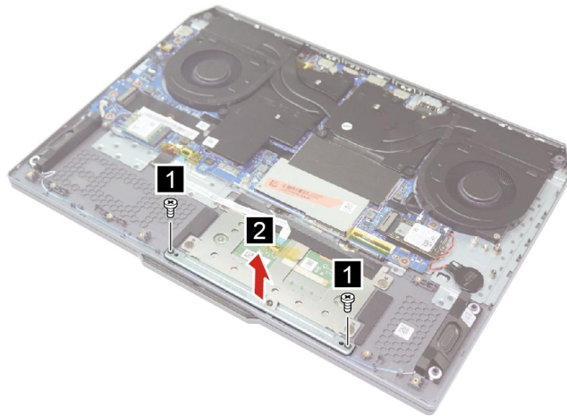
Figure 5. Remove two screws and remove the touchpad bracket
