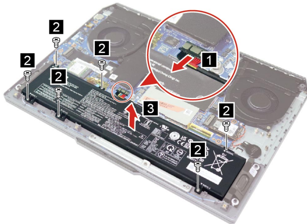
Figure 4. Remove six screws and the battery pack
