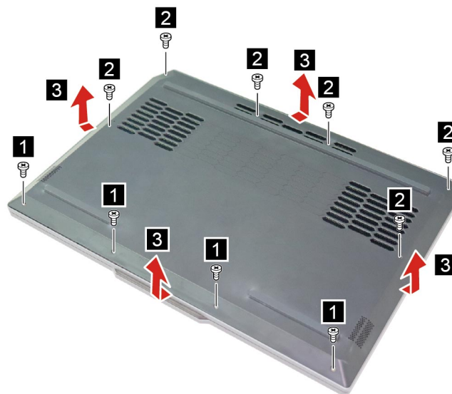
Figure 3. Remove ten screws and the lower case
