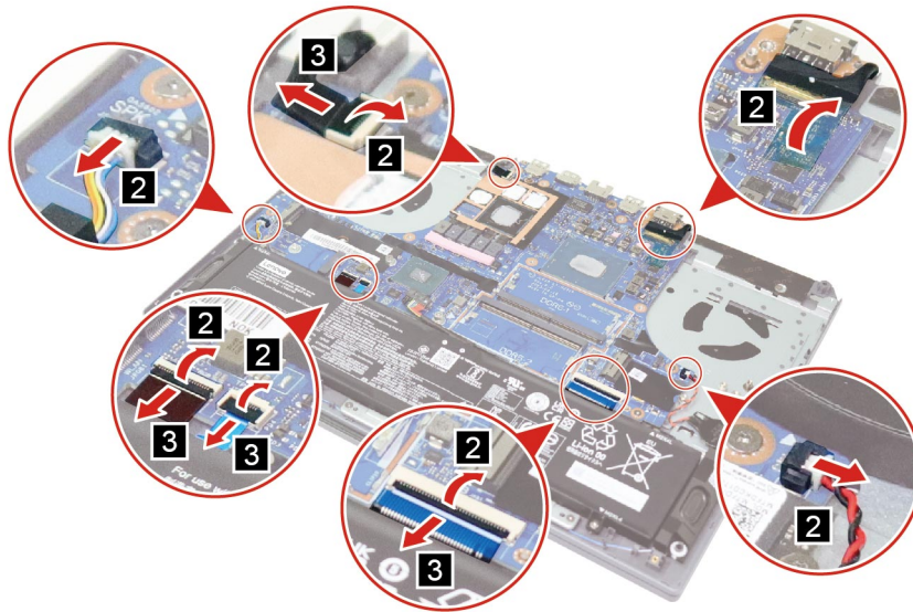
Figure 21. Disconnect all the cables and peel back the mylar
