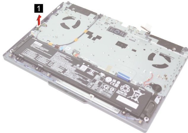
Figure 23. Remove the Type-C bracket
