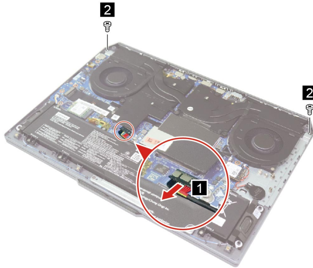
Figure 16. Disconnect the battery pack cable and remove two screws
