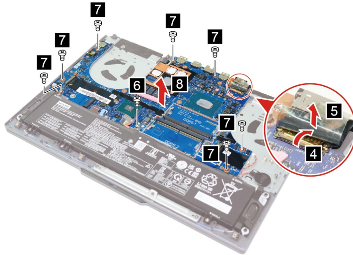
Figure 22. Disconnect the EDP cable, remove eight screws, and remove the system board
