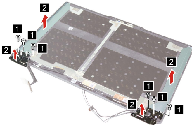
Figure 32. Remove six screws and the hinges
