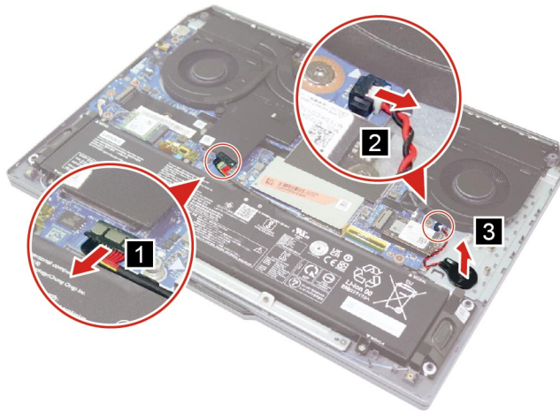
Figure 12. Disconnect the battery pack cable, disconnect the CMOS battery cable, and remove the CMOS battery
