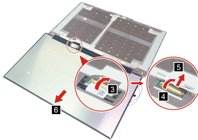
Figure 28. Disconnect the EDP cable and remove the LCD panel
