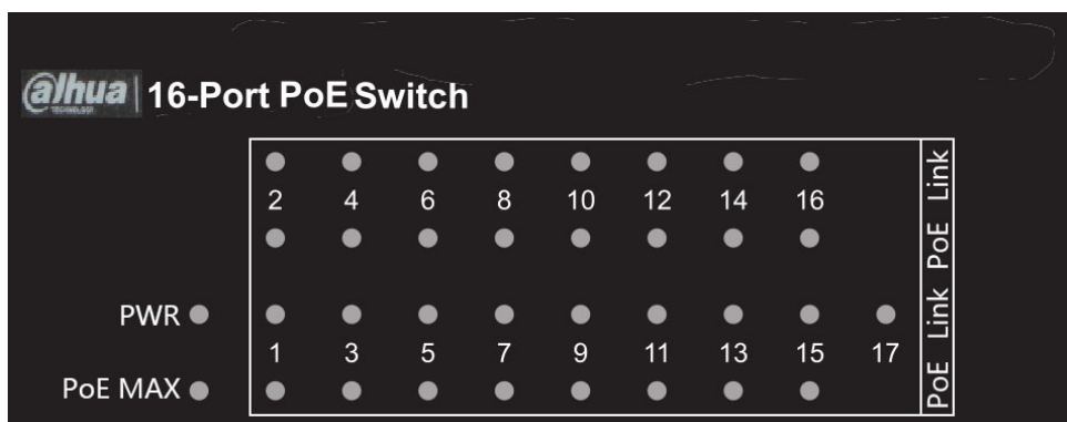
Figure 1-2 LED indicator
