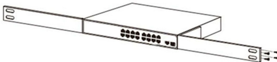
Figure 2-2 Rack installation
