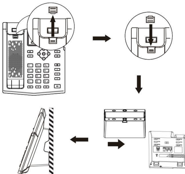
Picture 2 - Wall-mounted installation
