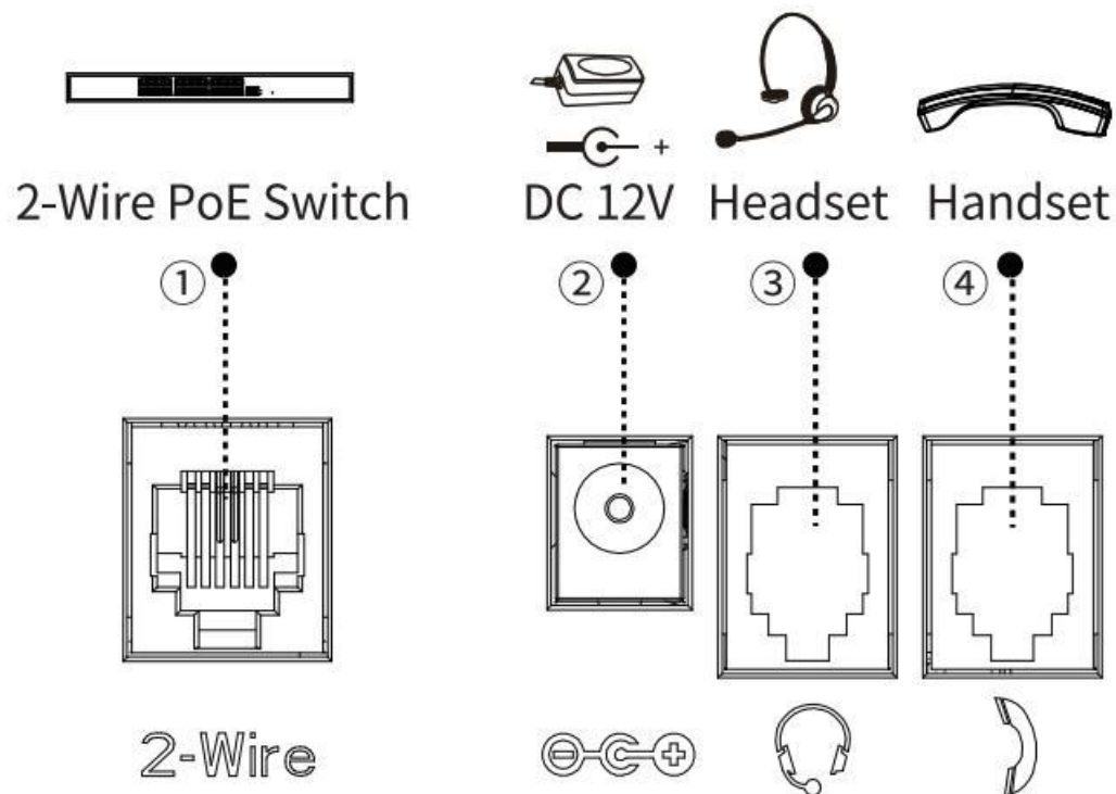
Picture 3 - Connecting to the Device
