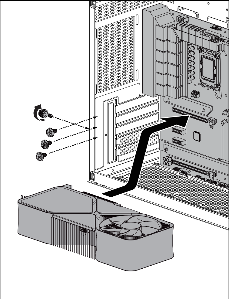
▼ GPU Installation
