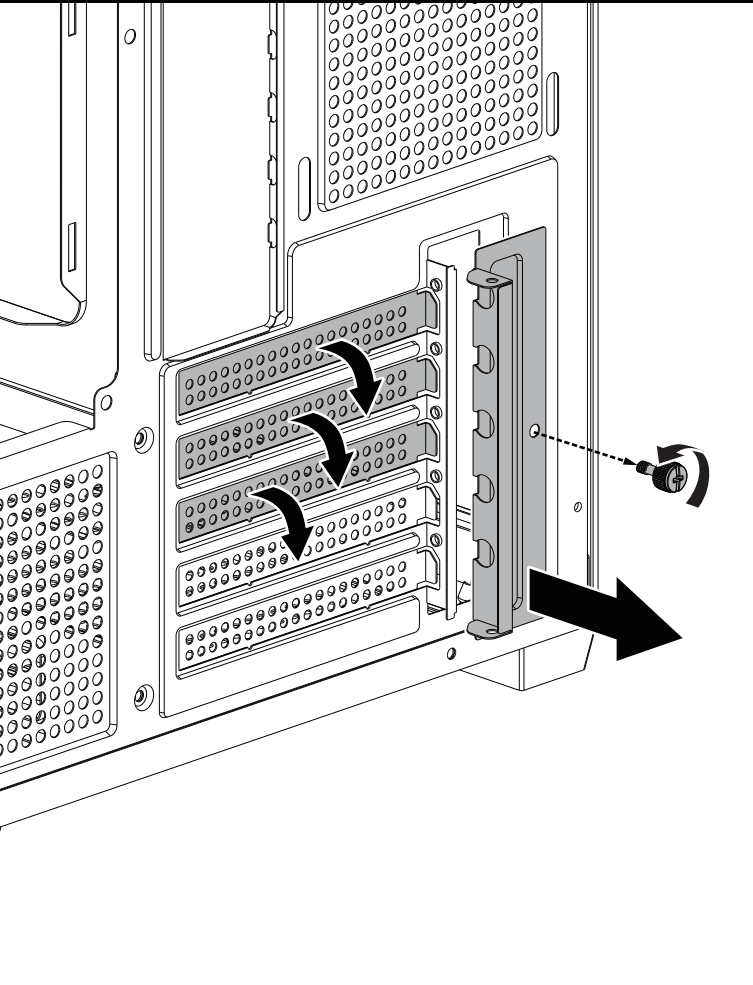
▼ GPU Installation
