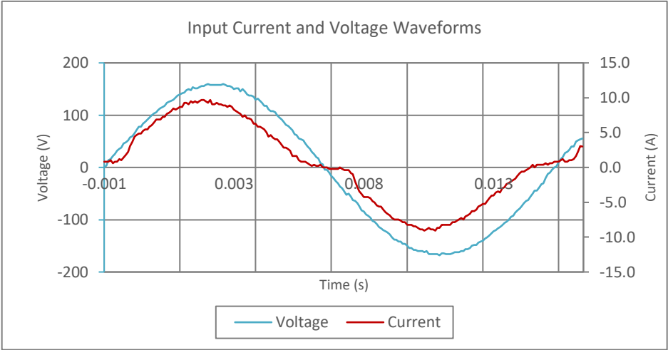
Input AC Current Waveform (ITHD = 15.78%, 50% Load)
