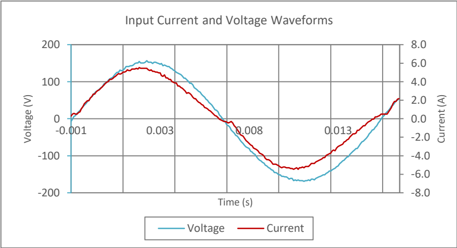
Input AC Current Waveform (ITHD = 8.22%, 50% Load)
