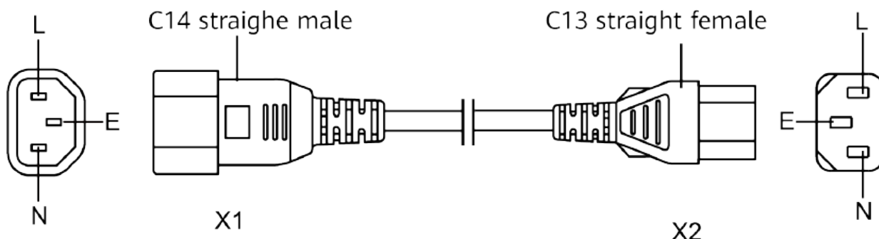
Figure 6-16 Structure of a C14 straight male to C13 straight female AC power cable
