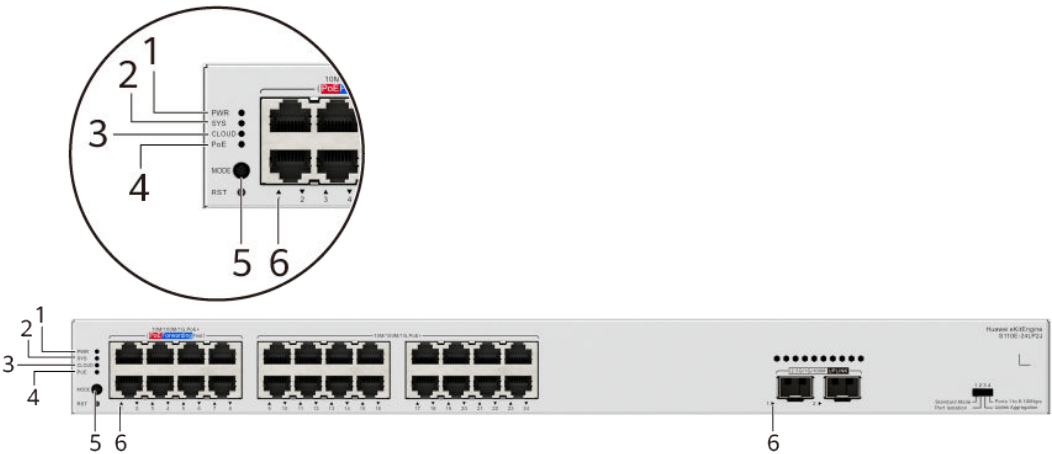
Figure 4-18 Indicators on the Switch
