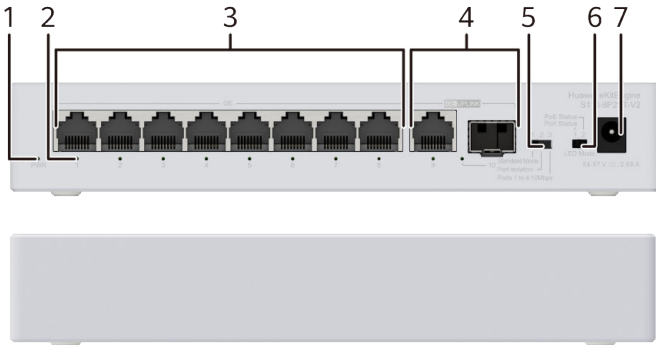
Figure 4-7 S110-8P2ST-V2 appearance
