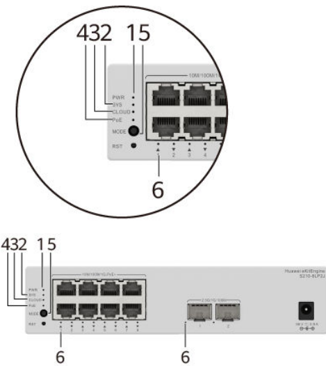
Figure 4-32 Indicators on the Switch
