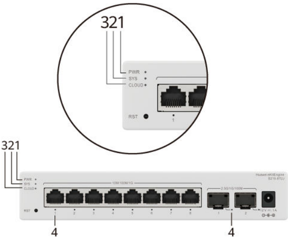
Figure 4-38 Indicators on the Switch
