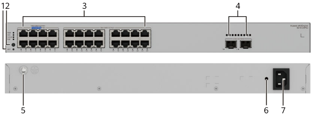
Figure 4-39 S210-24P2J appearance
