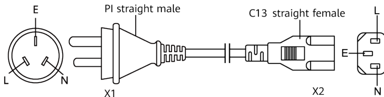
Figure 6-17 Structure of a PI straight male to C13 straight female AC power cable (used in China)
