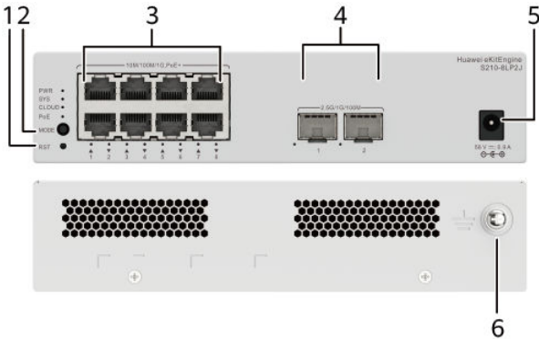
Figure 4-29 S210-8LP2J appearance
