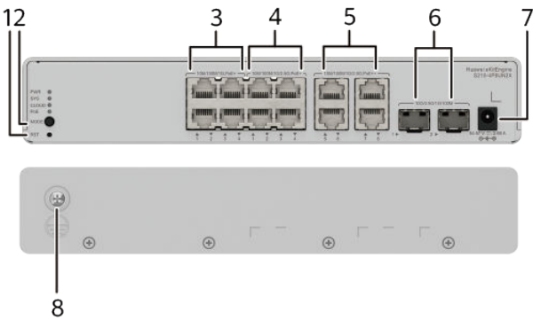
Figure 4-45 S210-4P8UN2X appearance
