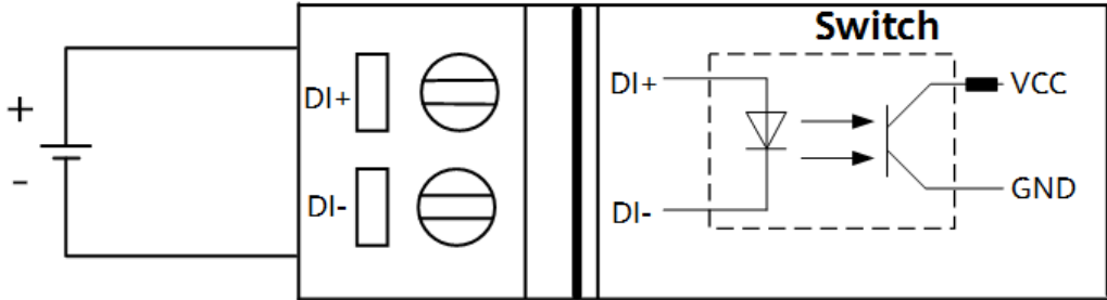
Figure 4-52 Typical connections of the DI port
