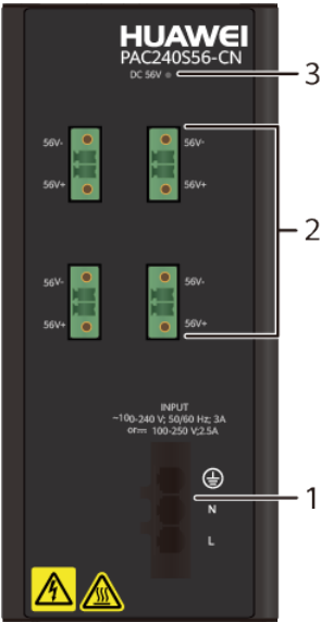
Figure 5-4 Panel of the PAC240S56-CN
