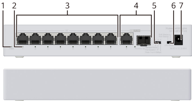
Figure 4-8 S110-8P2ST-V2 appearance
