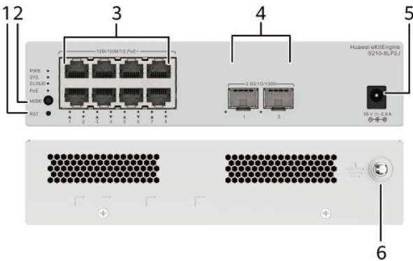
Figure 4-27 S210-8LP2J appearance
