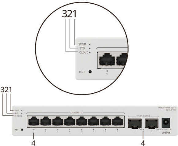
Figure 4-36 Indicators on the Switch
