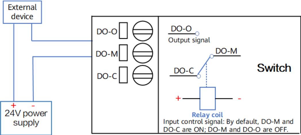
Figure 4-49 Typical connections of the DO port
