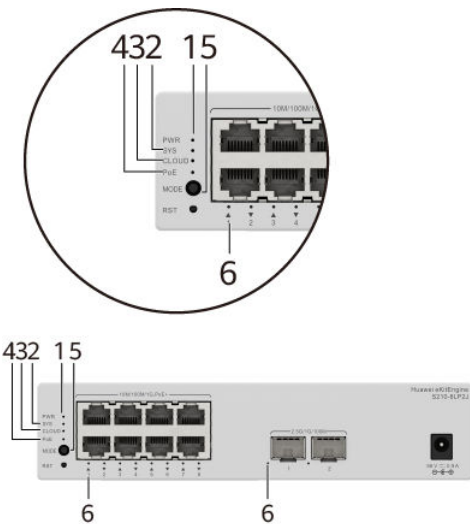
Figure 4-40 Indicators on the Switch
