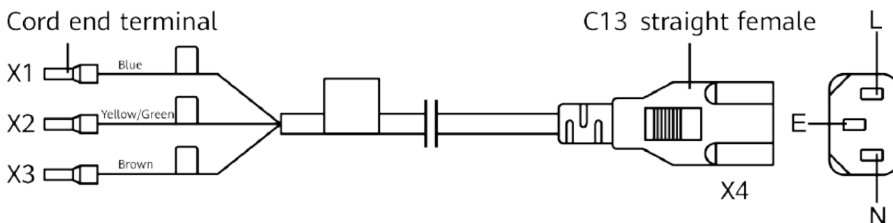
Figure 6-18 Structure of a Cord end to C13 straight female AC power cable (used in China)
