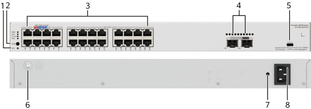
Figure 4-15 S110E-24LP2J appearance
