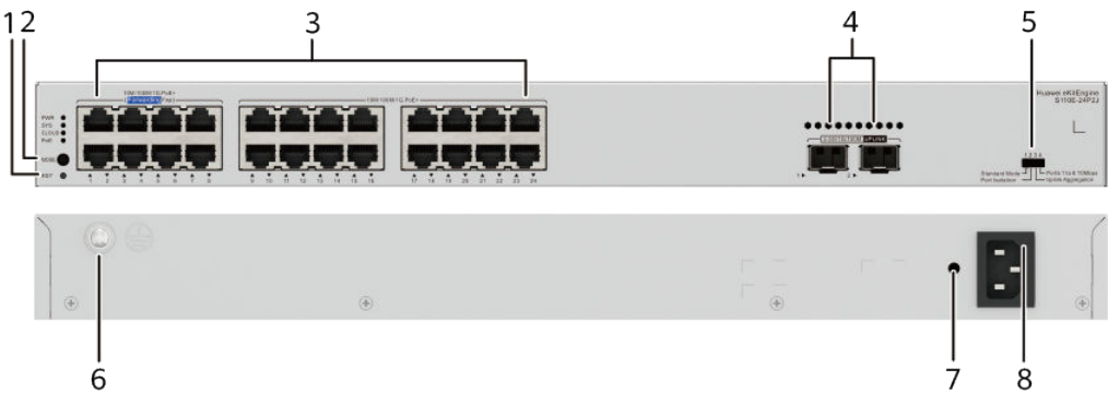
Figure 4-17 S110E-24P2J appearance
