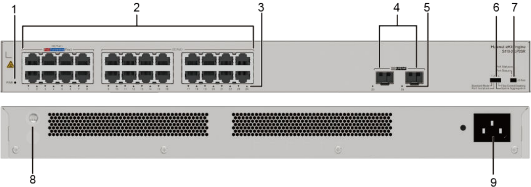
Figure 4-12 S110-24LP2SR appearance
