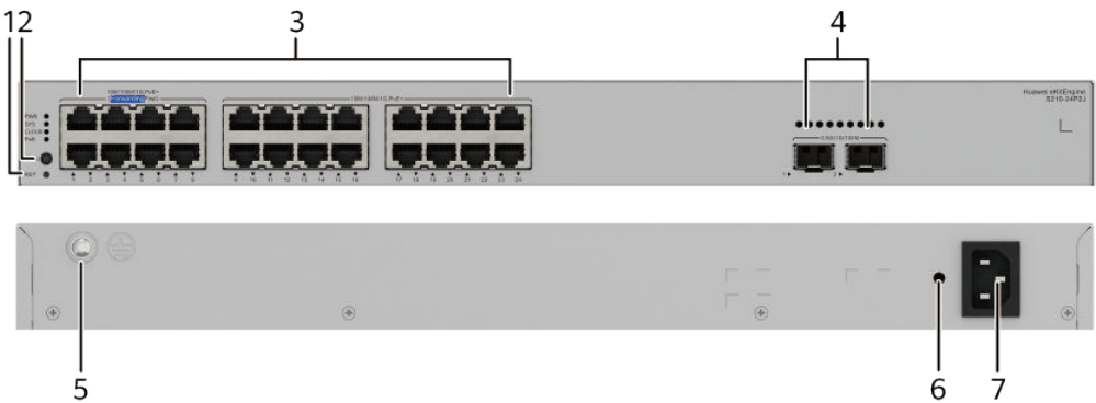
Figure 4-41 S210-24P2J appearance
