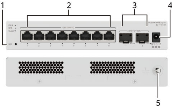
Figure 4-23 S210-8T2J appearance
