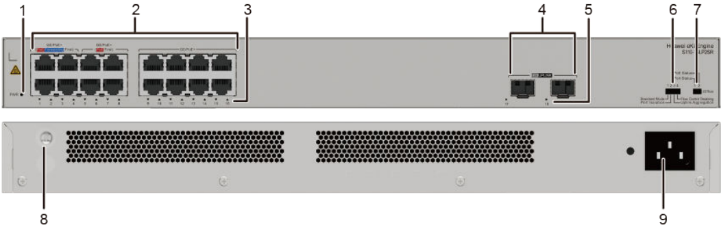
Figure 4-10 S110-16LP2SR appearance
