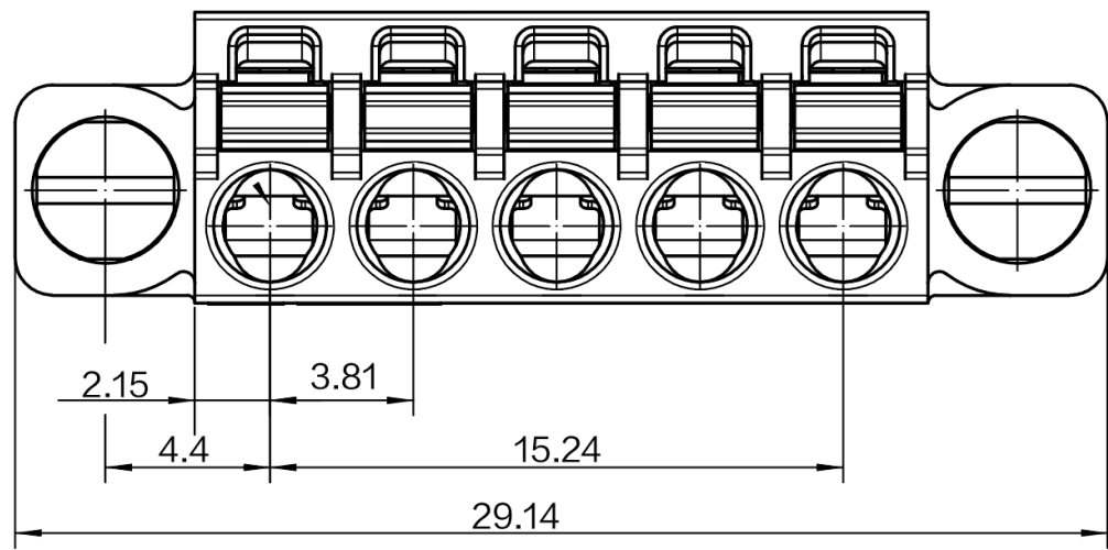
Figure 6-21 Phoenix connector dimensions
