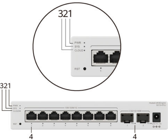
Figure 4-20 Indicators on the Switch
