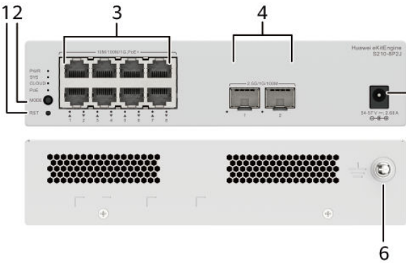
Figure 4-33 S210-8P2J appearance
