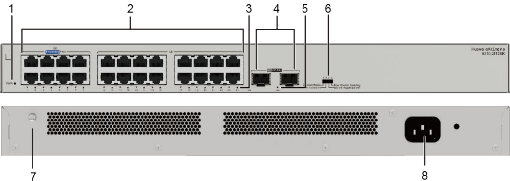
Figure 4-11 S110-24T2SR appearance
