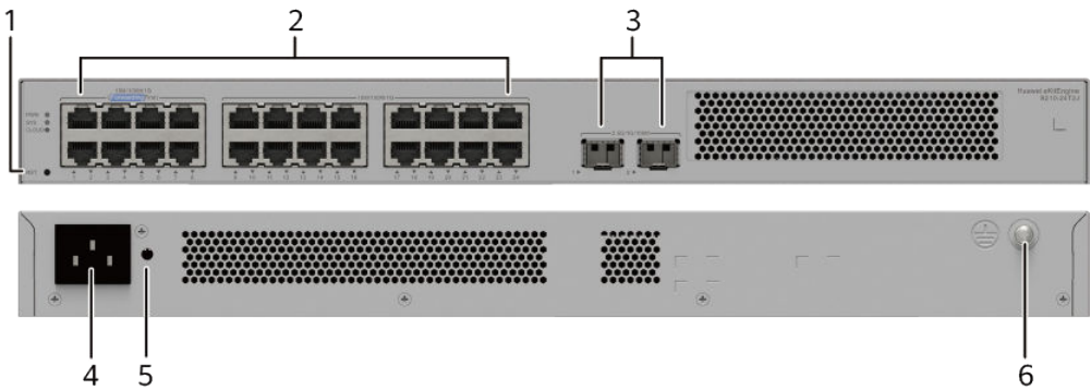
Figure 4-35 S210-24T2J appearance
