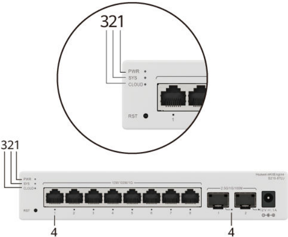
Figure 4-22 Indicators on the Switch
