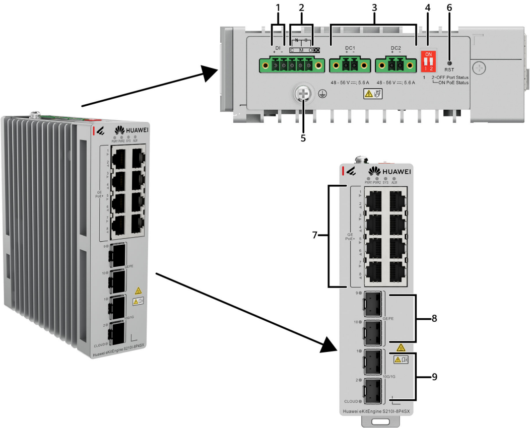
Figure 4-55 S210I-8P4SX appearance
