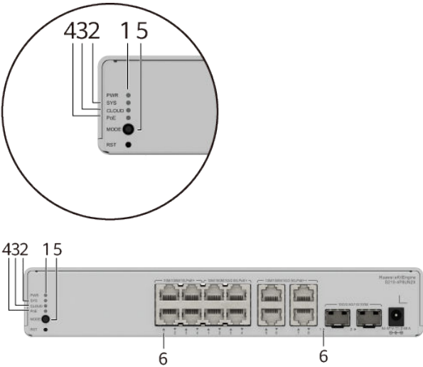
Figure 4-46 Indicators on the Switch
