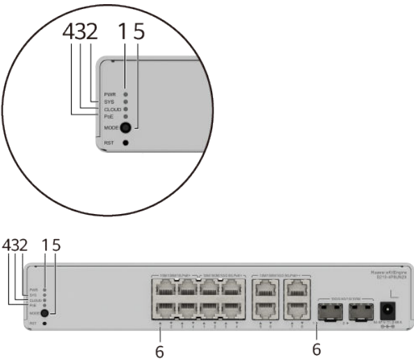
Figure 4-44 Indicators on the Switch
