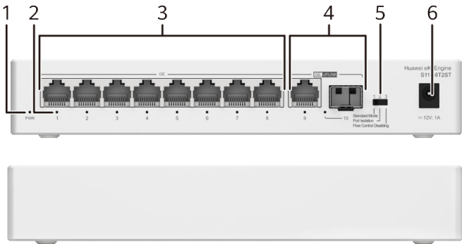
Figure 4-3 S110-8T2ST appearance
