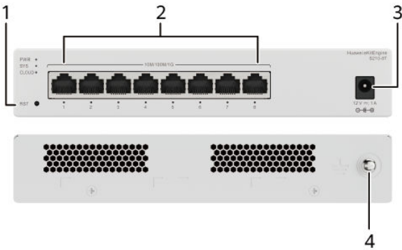
Figure 4-19 S210-8T appearance
