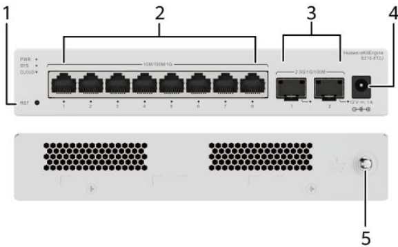
Figure 4-25 S210-8T2J appearance
