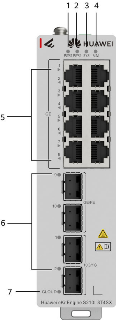
Figure 4-54 Indicators on the device
