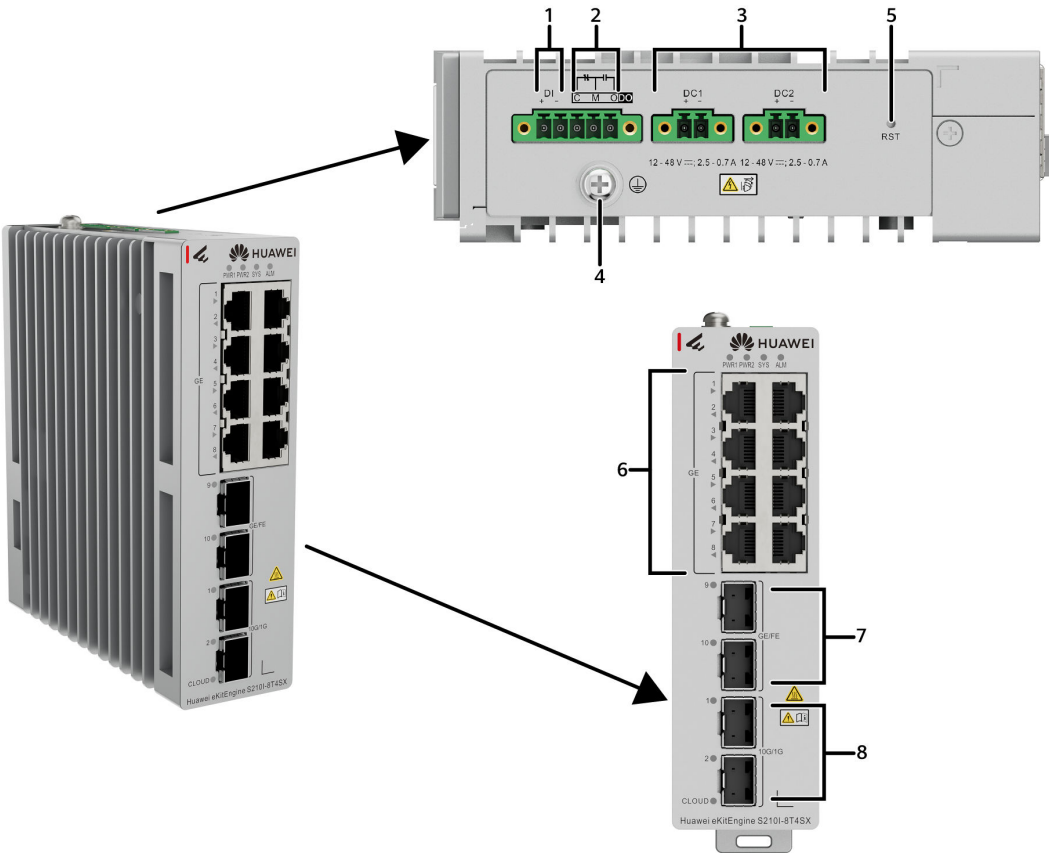
Figure 4-51 S210I-8T4SX appearance
