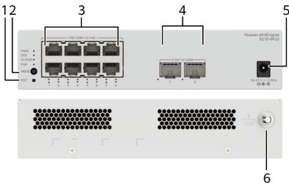
Figure 4-31 S210-8P2J appearance
