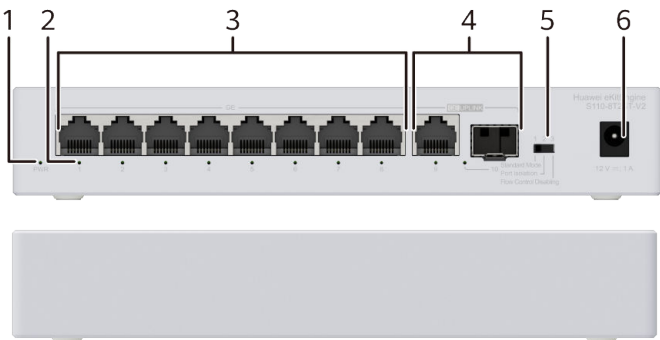
Figure 4-4 S110-8T2ST-V2 appearance
