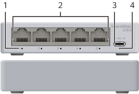
Figure 4-2 S110-5T appearance
