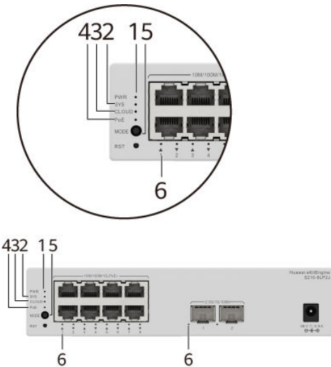
Figure 4-28 Indicators on the Switch
