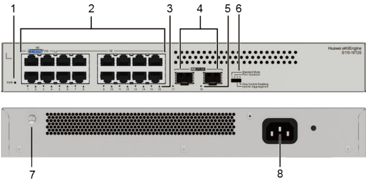
Figure 4-9 S110-16T2S appearance
