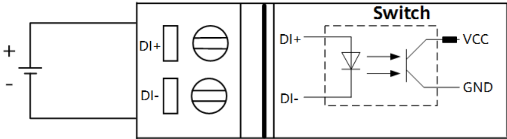
Figure 4-60 Typical connections of the DI port
