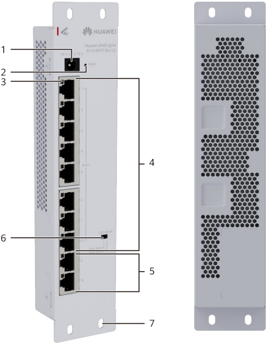
Figure 4-14 S110-8P2T-BU-V2 appearance
