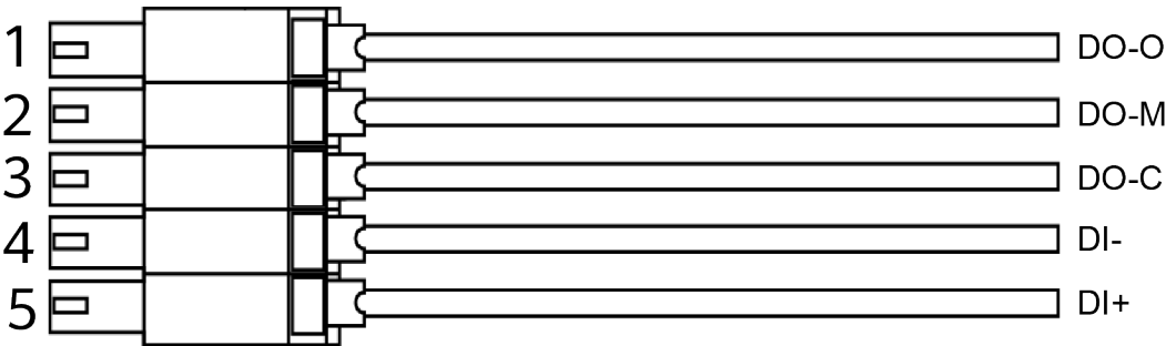
Figure 6-20 Structure of a 5-pin Phoenix connector (DI/DO)
