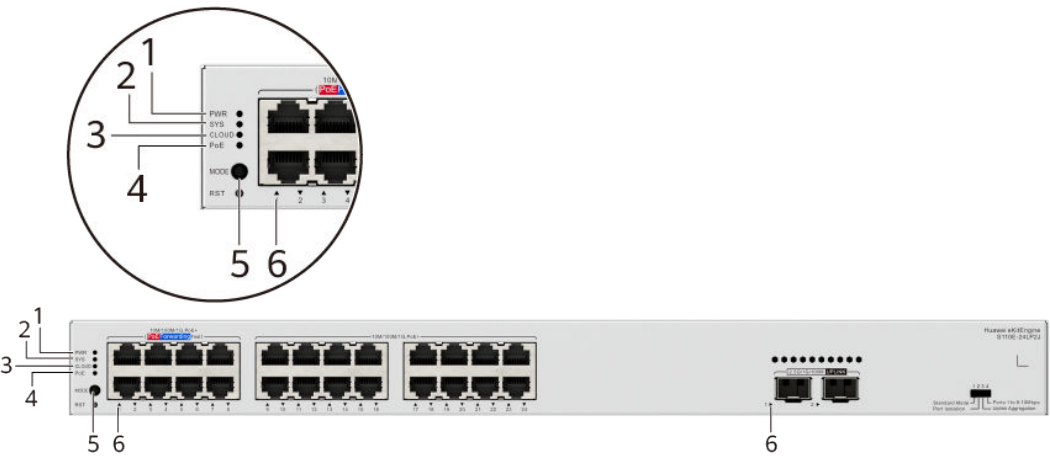
Figure 4-16 Indicators on the Switch
