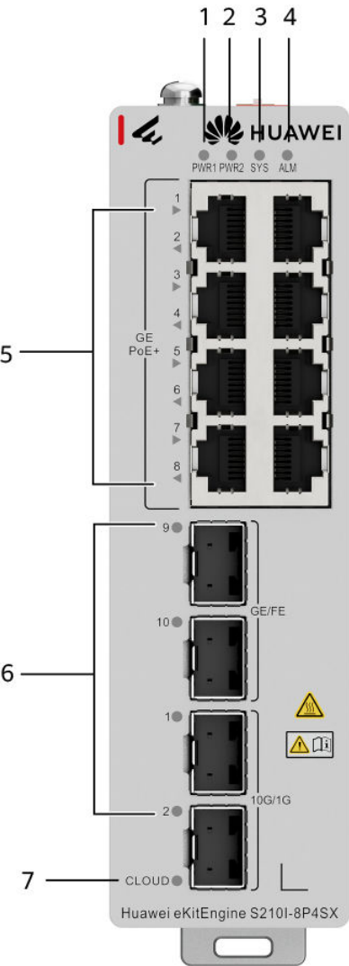
Figure 4-58 Indicators on the device
