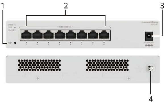
Figure 4-21 S210-8T appearance
