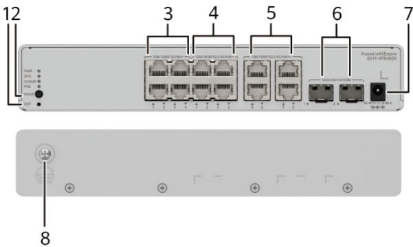
Figure 4-43 S210-4P8UN2X appearance
