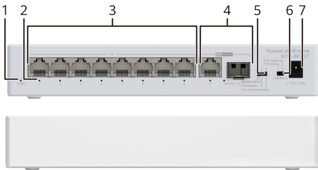
Figure 4-6 S110-8P2ST appearance
