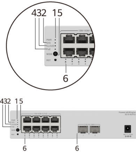
Figure 4-34 Indicators on the Switch
