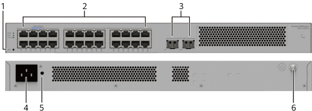
Figure 4-37 S210-24T2J appearance
