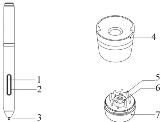
Image 3-1: Stylus and accessories
