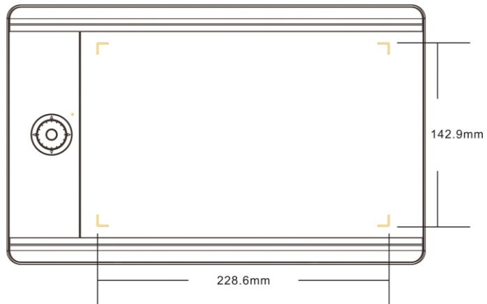
Image 2-2: Working area
