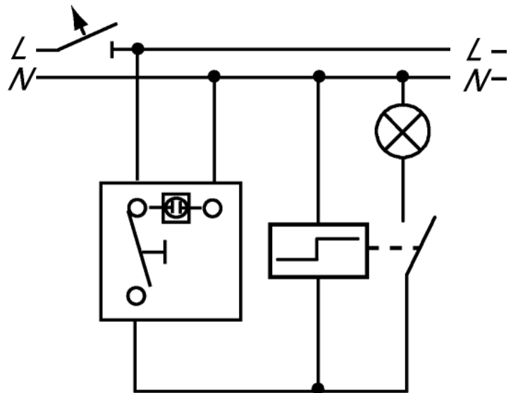
Push switch
