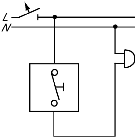
Push switch
