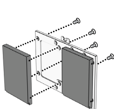
2.5" Drive
