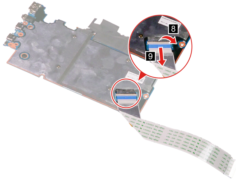
Figure 36. Remove the I/O board cable
