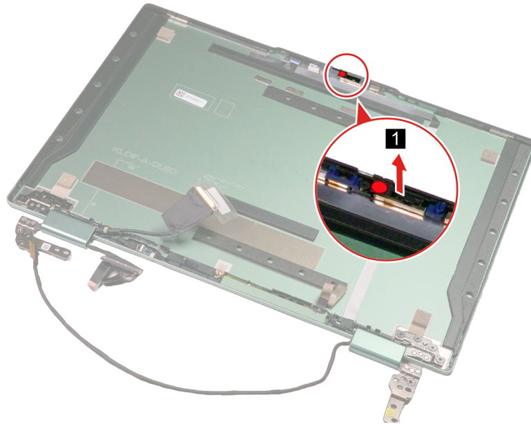
Figure 28. Remove the camera shutter
