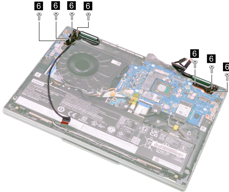
Figure 18. Remove seven screws
