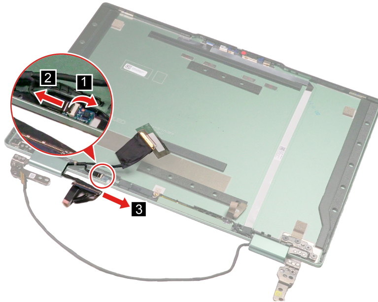
Figure 31. Remove the EDP cable
