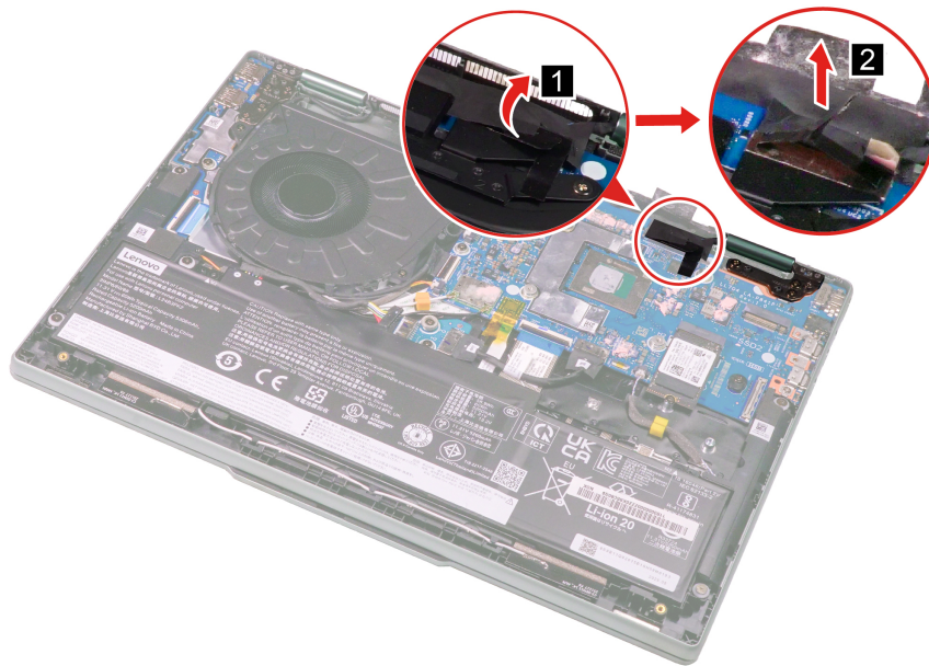
Figure 16. Disconnect the EDP cable connector
