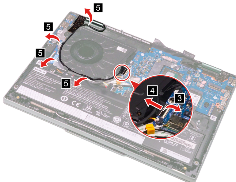
Figure 17. Disconnect the camera cable connector
