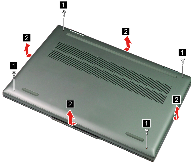
Figure 1. Remove four screws and the lower case
