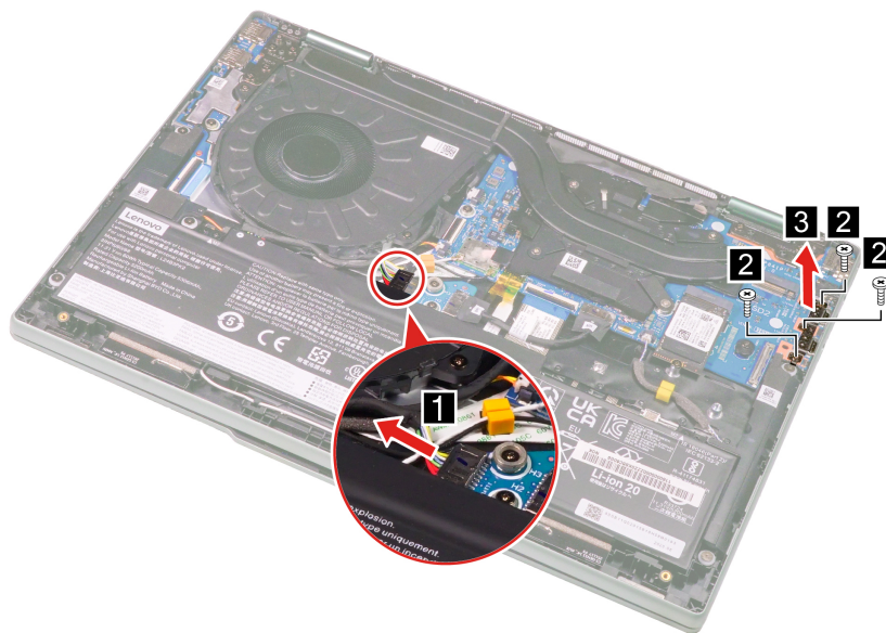
Figure 10. Remove the Type-C bracket
