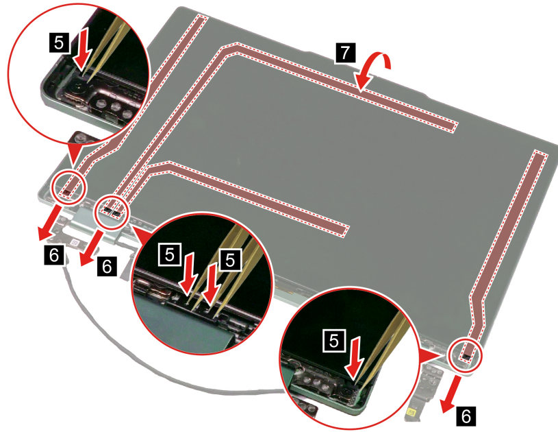
Figure 23. Take out four stretch-release tapes and lift the display panel
