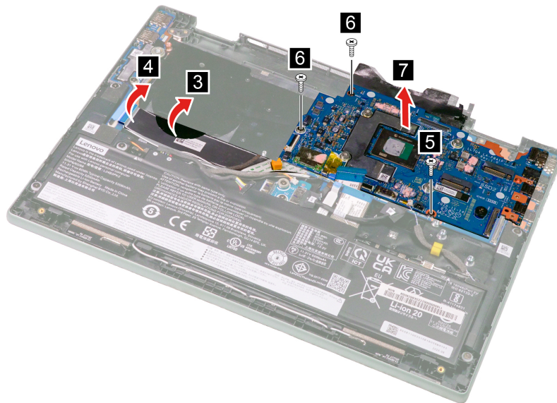
Figure 35. Remove the system board
