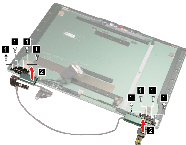
Figure 32. Remove the hinges
