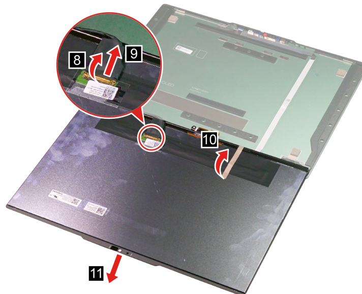
Figure 24. Disconnect the EDP cable and remove the display panel
