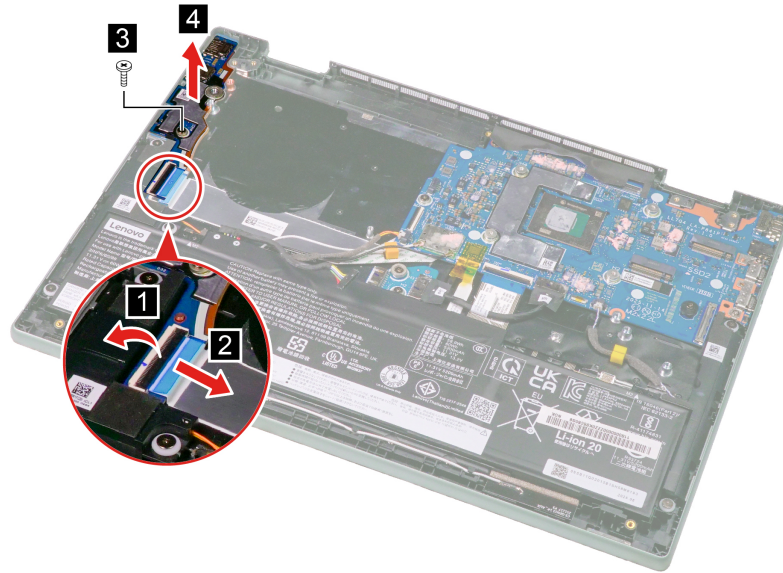
Figure 33. Remove the I/O board
