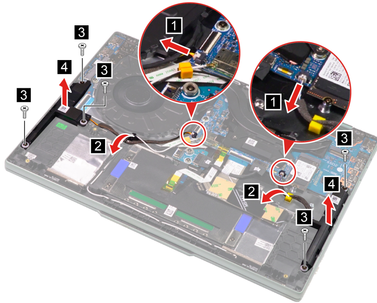
Figure 11. Remove the speakers
