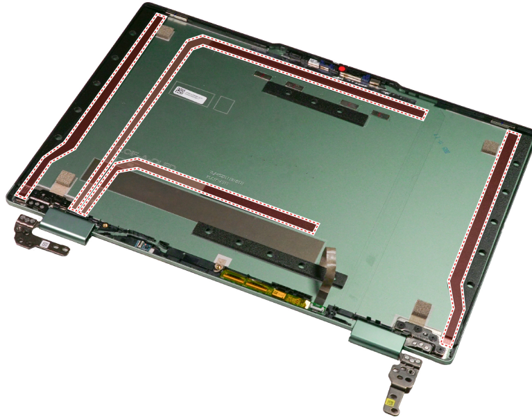
Figure 25. The locations of the stretch-release tapes
