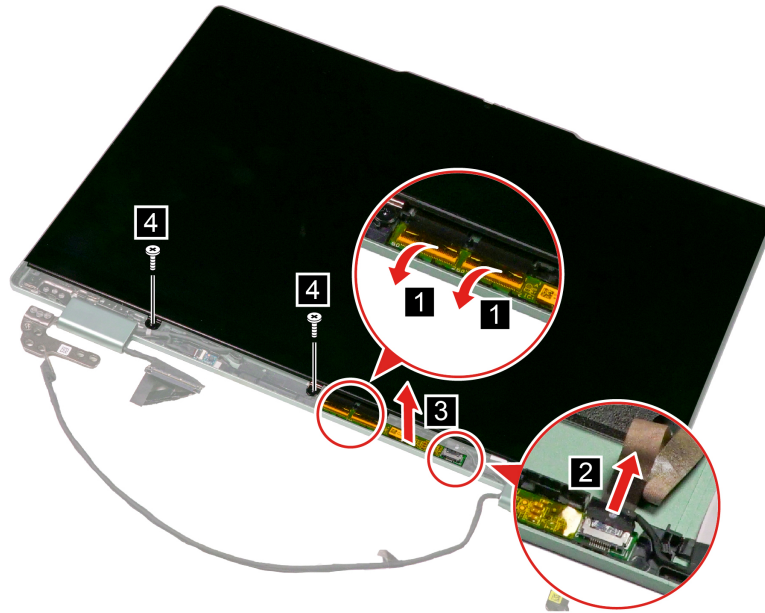
Figure 22. Disconnect the touch board connectors, pry up the touch board, and remove two screws
