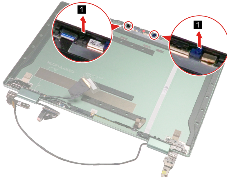
Figure 26. Remove the microphone rubbers
