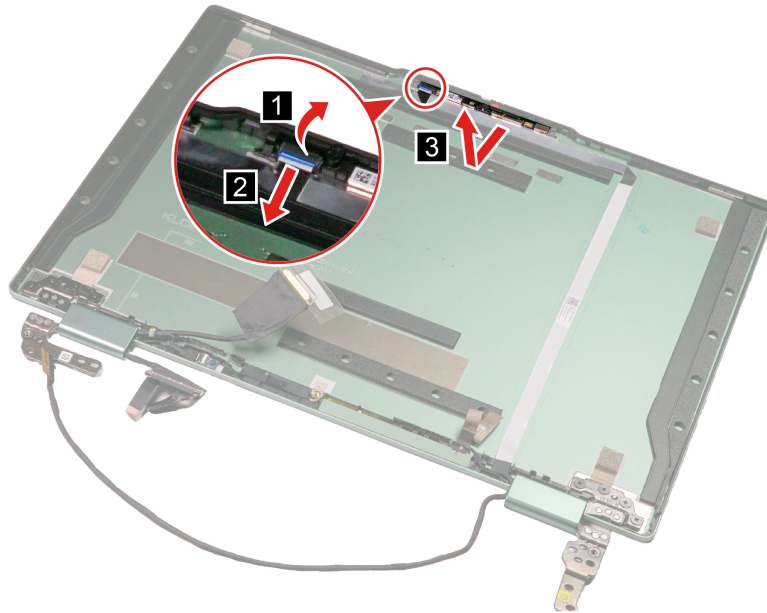
Figure 29. Remove the camera board
