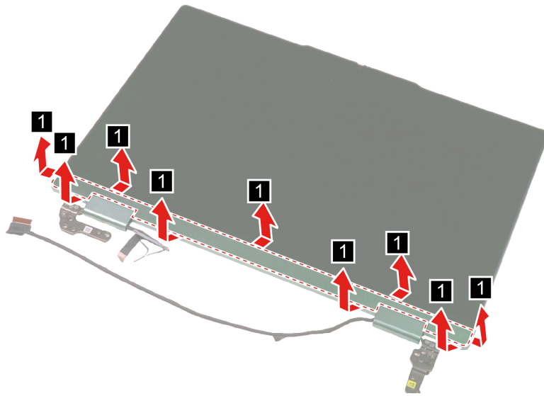
Figure 20. Remove the strip cover
