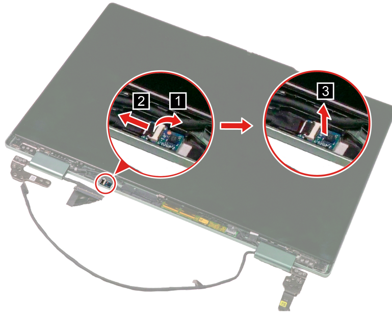
Figure 21. Remove the sensor board
