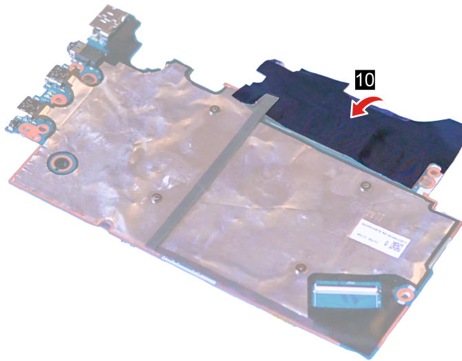
Figure 37. Peel off the MB acetate tape covering the PMIC board and the PMIC cable
