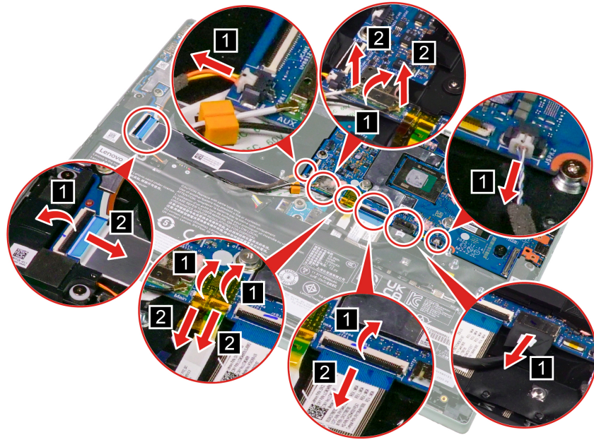
Figure 34. Disconnect all the cables
