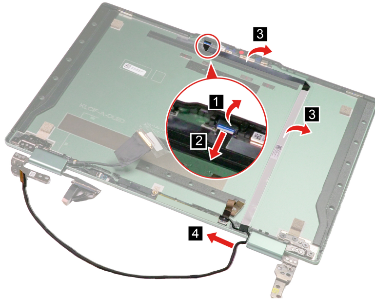
Figure 30. Remove the camera cable
