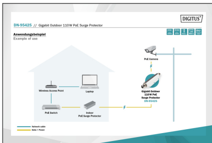
Gigabit Outdoor 110 W PoE Surge Protector
