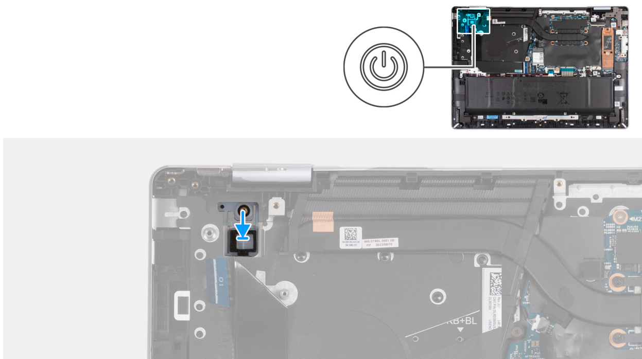
Figure 43. Installing power button
