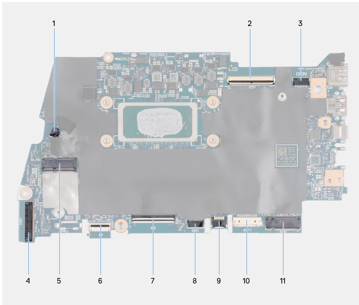
Figure 48. System board callouts
