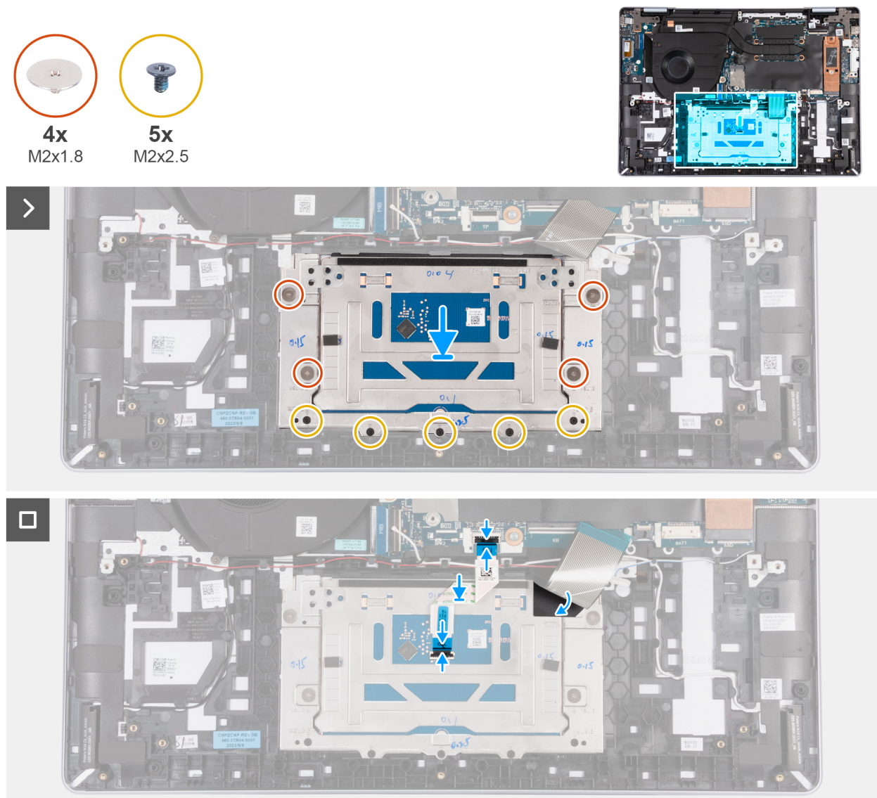
Figure 55. Installing the touchpad
