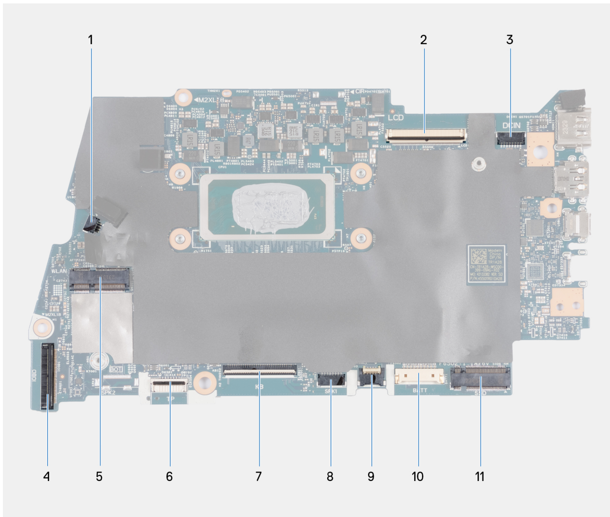
Figure 51. System board callouts
