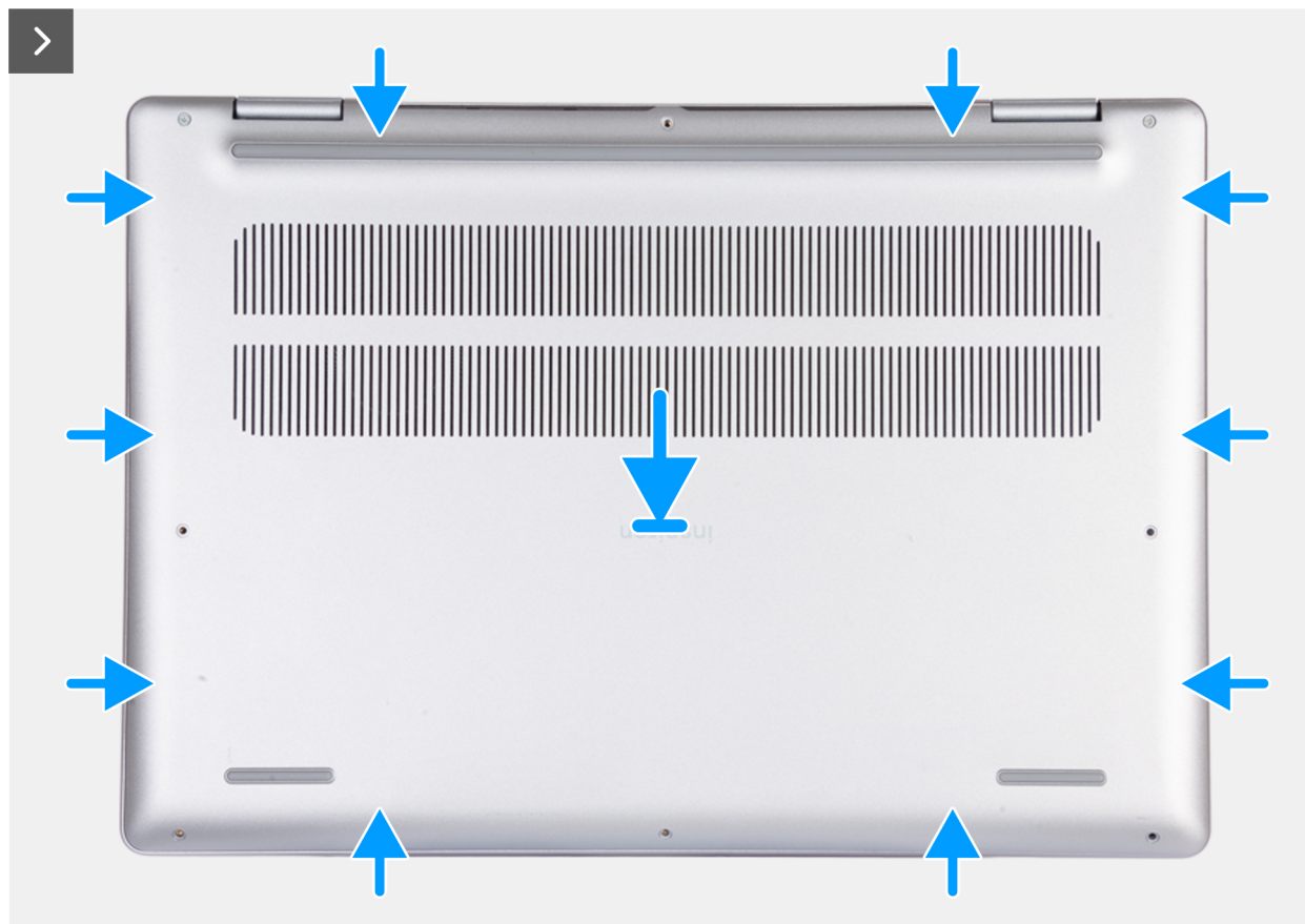
Figure 11. Installing the base cover 1
