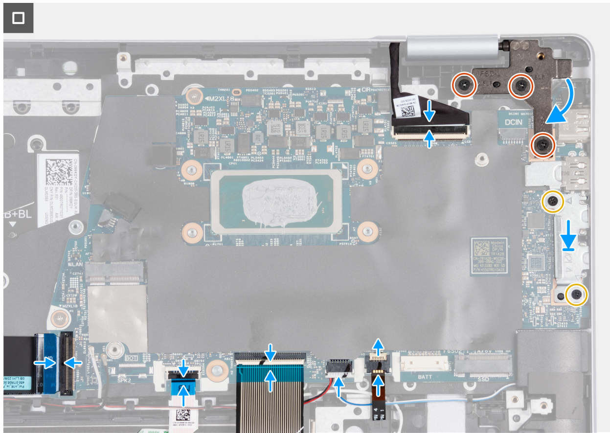
Figure 53. Installing the system board 2
