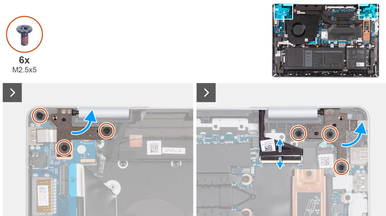
Figure 31. Removing the display assembly 1
