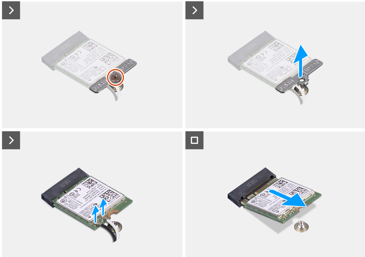
Figure 19. Removing the wireless card
