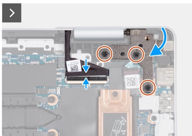
Figure 35. Installing the display assembly 2
