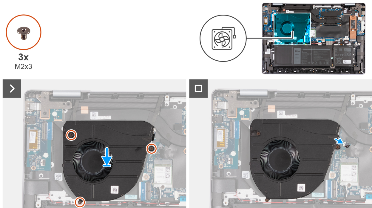
Figure 18. Installing the fan
