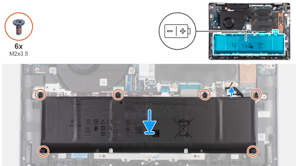
Figure 24. Installing the 6-cell battery (90 Wh)
