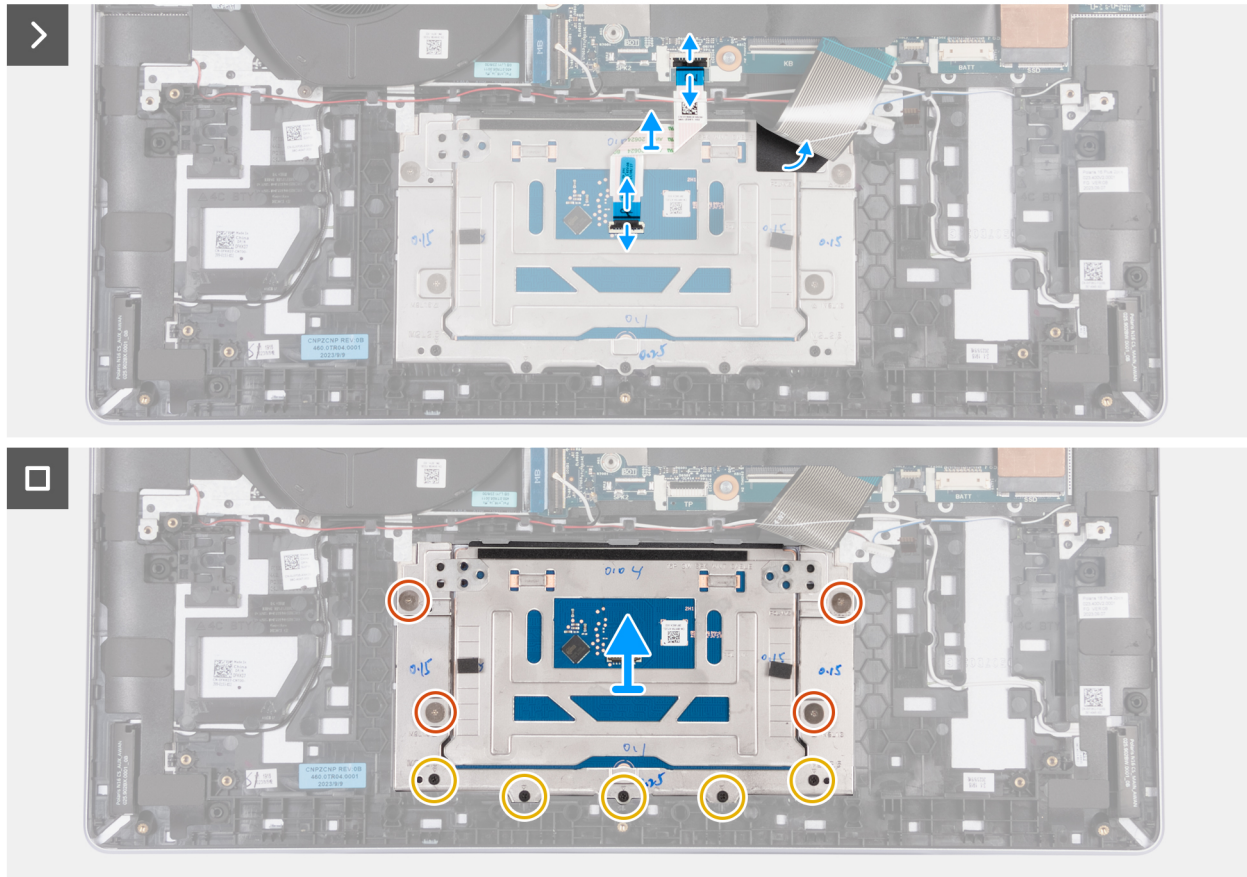
Figure 54. Removing the touchpad
