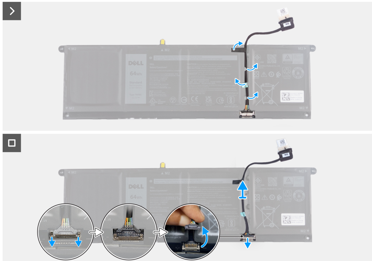
Figure 25. Removing the 64 Wh battery cable
