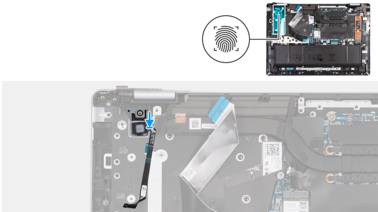
Figure 42. Installing power button with an optional fingerprint reader
