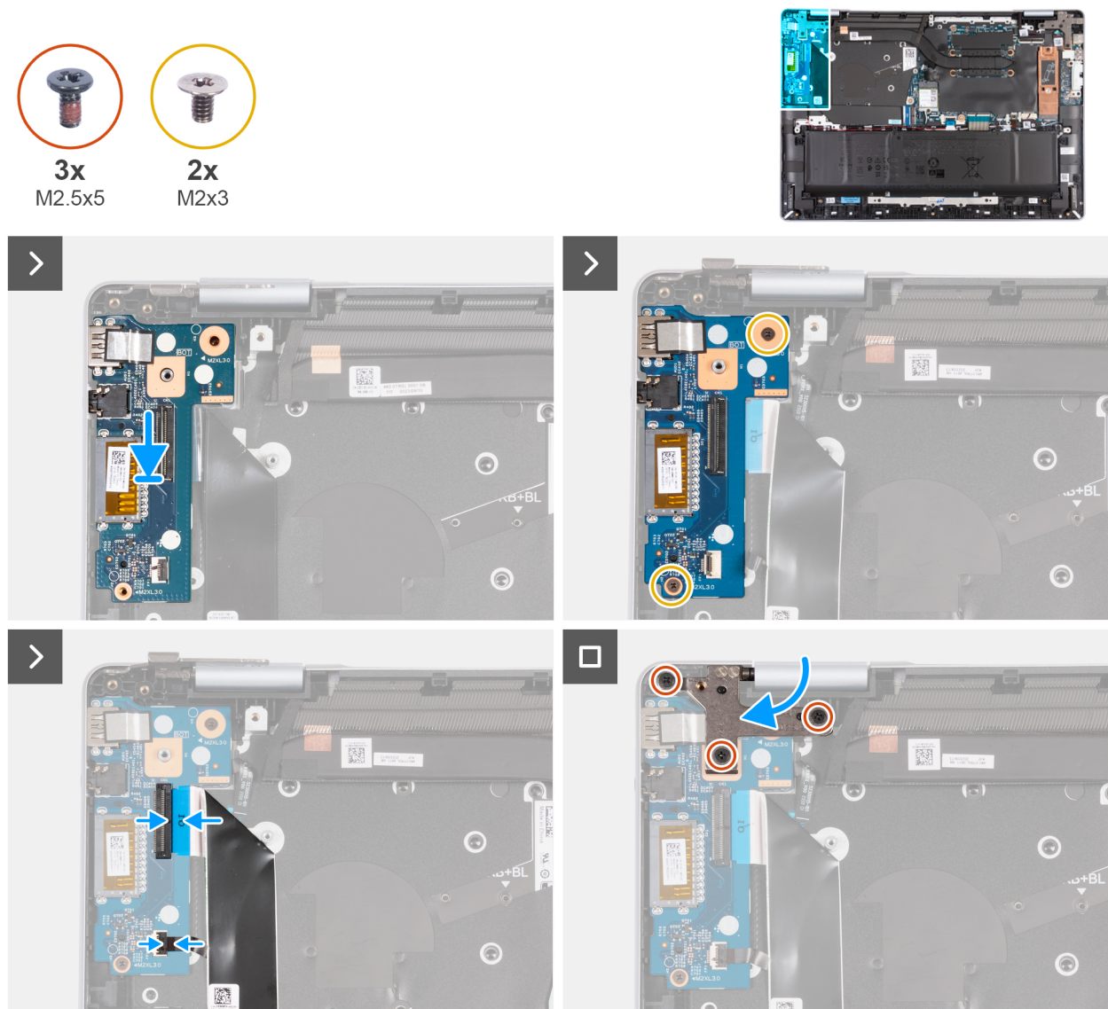
Figure 37. Installing the I/O board
