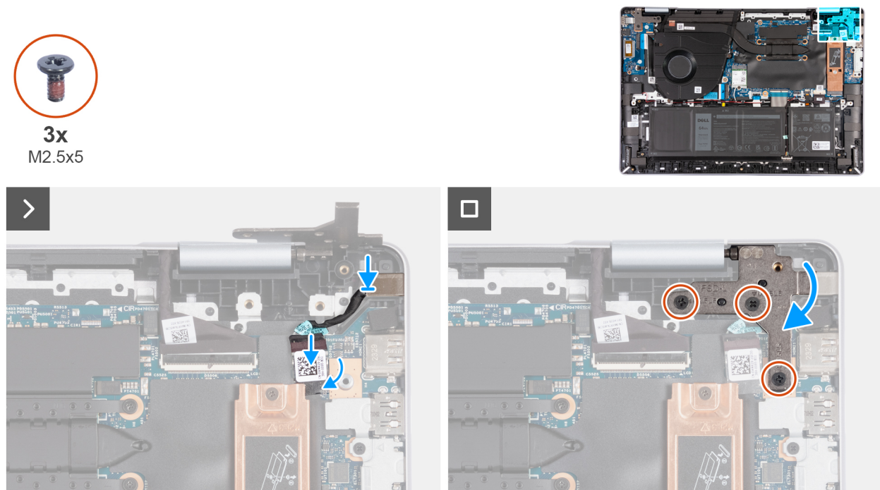
Figure 45. Installing the power-adapter port
