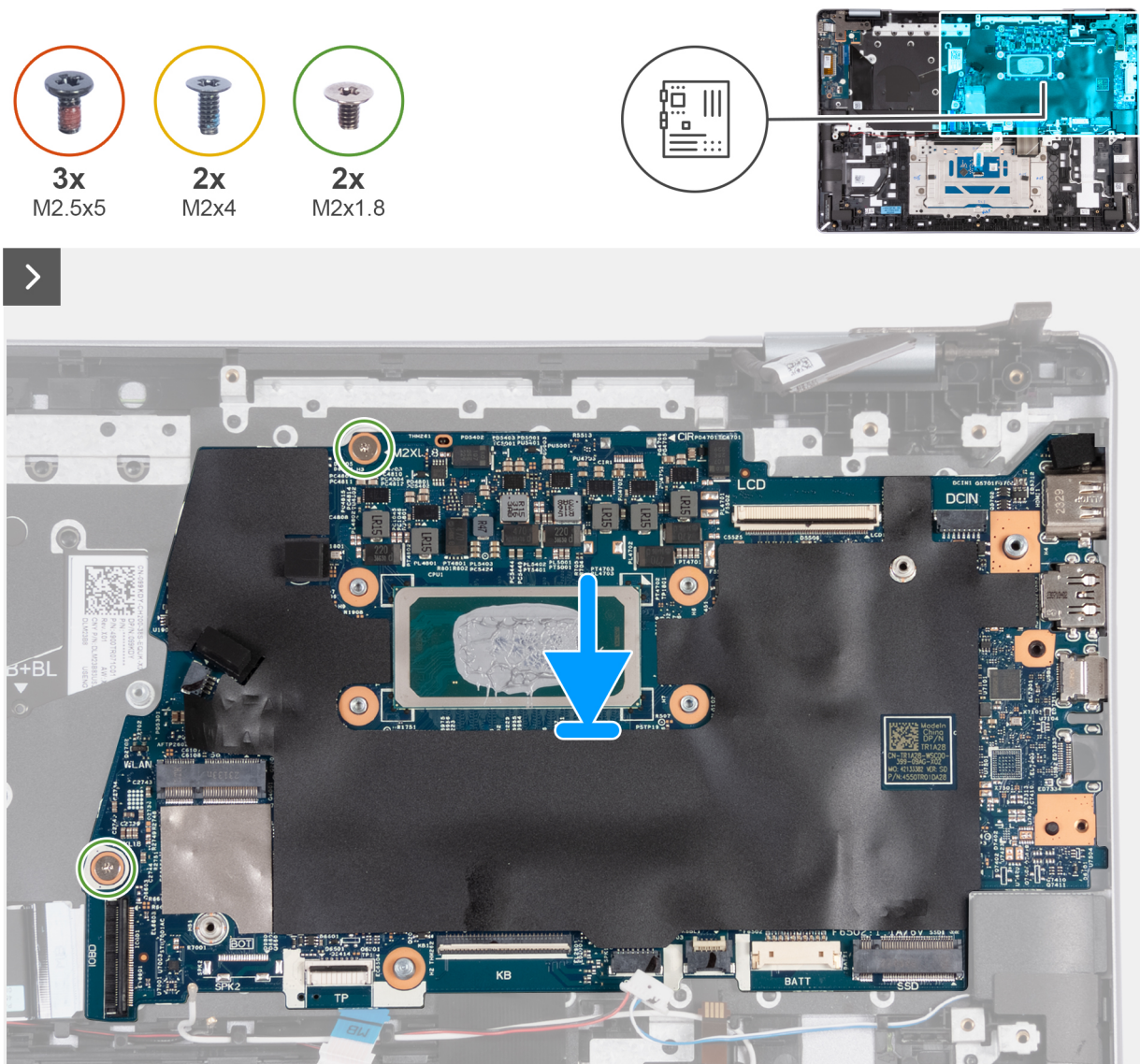
Figure 52. Installing the system board 1
