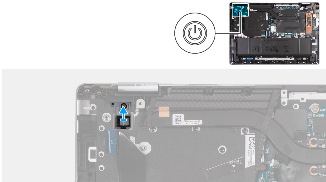
Figure 41. Removing the power button
