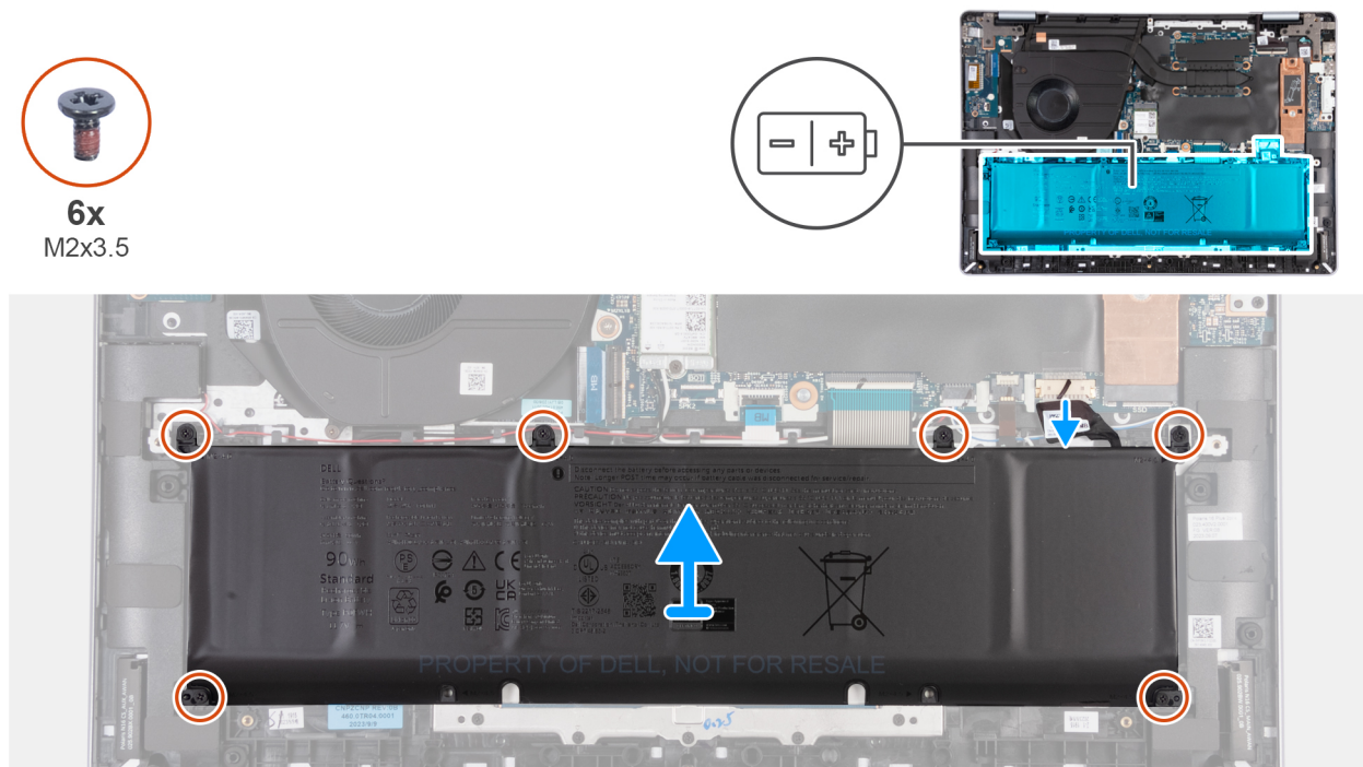
Figure 23. Removing the 6-cell battery (90 Wh)
