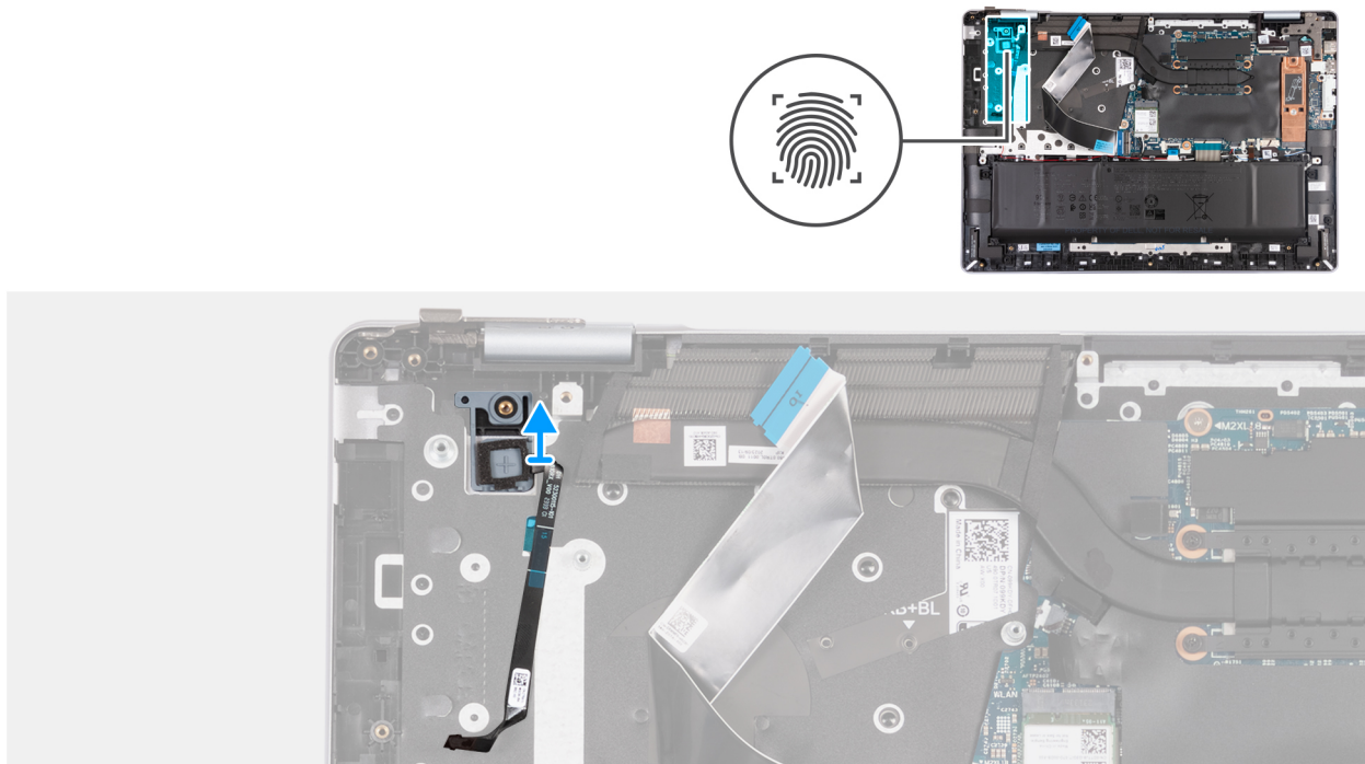
Figure 40. Removing the power button with an optional fingerprint reader
