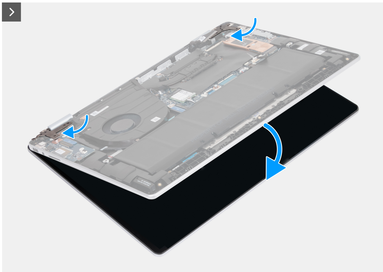
Figure 34. Installing the display assembly 1
