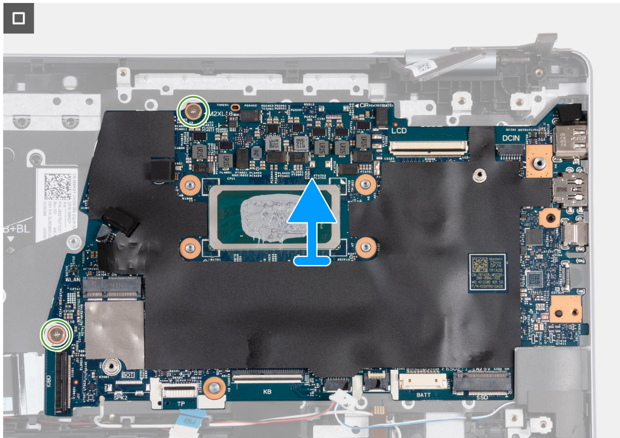
Figure 50. Removing the system board 2
