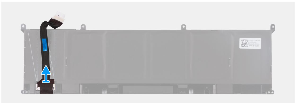
Figure 27. Removing the 90 Wh battery cable
