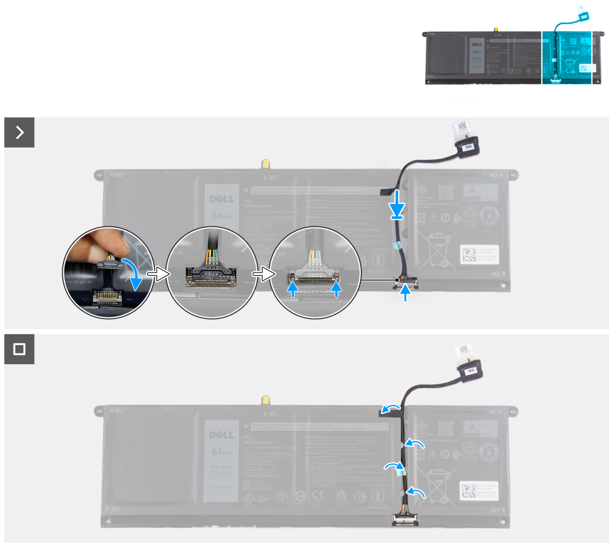
Figure 26. Installing the 64 Wh battery cable
