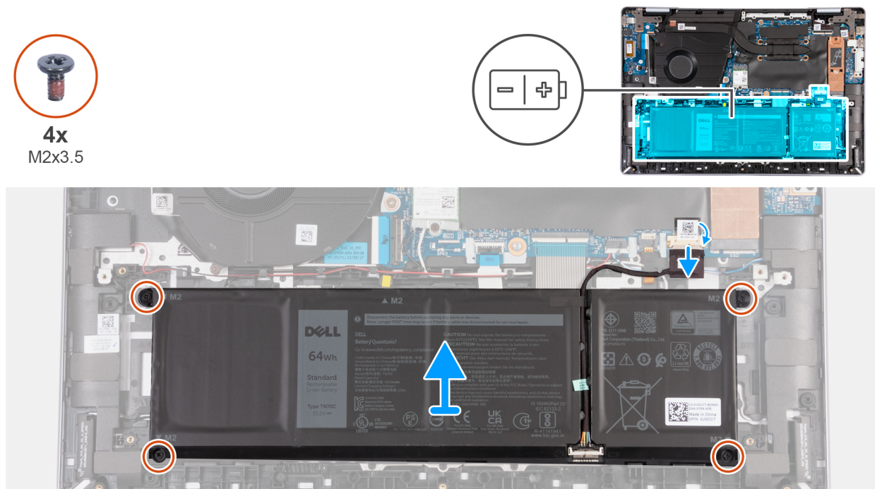
Figure 21. Removing the 4-cell battery (64 Wh)
