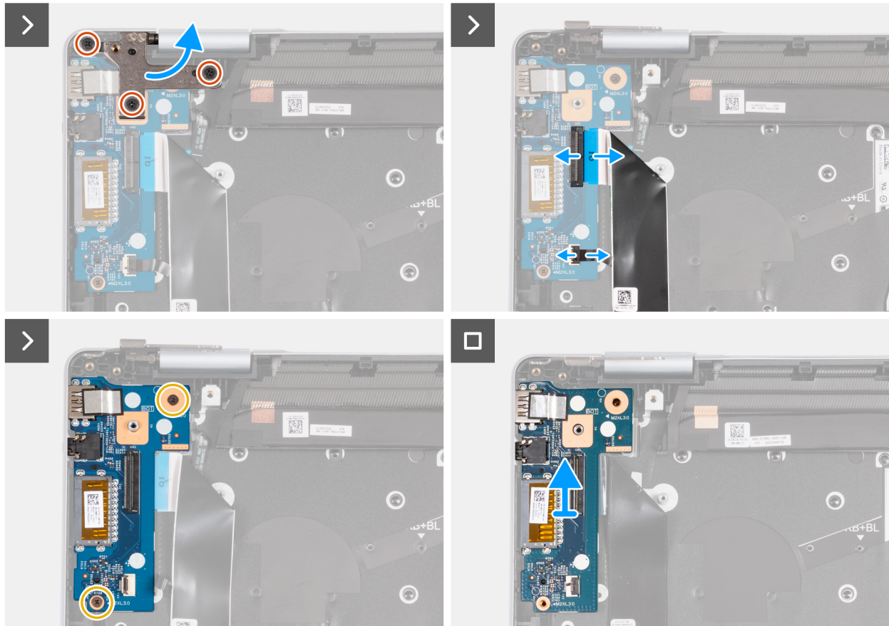
Figure 36. Removing the I/O board
