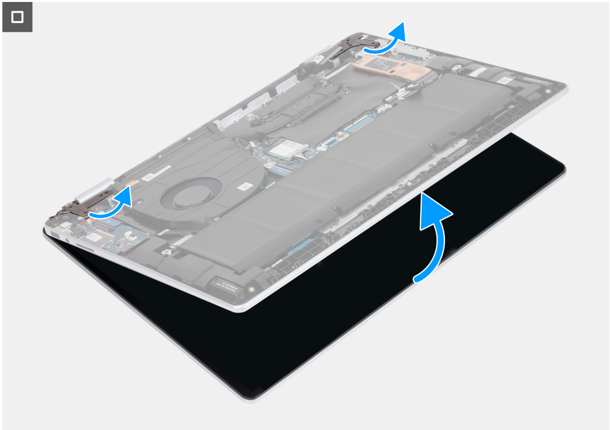
Figure 32. Removing the display assembly 2
