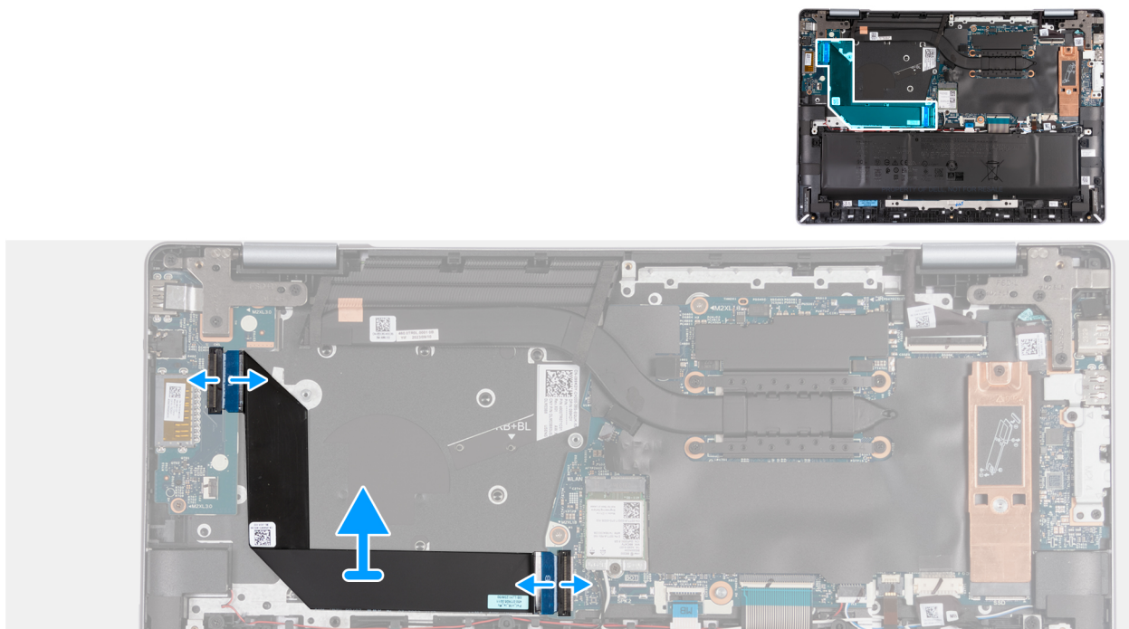
Figure 38. Removing the I/O-board cable
