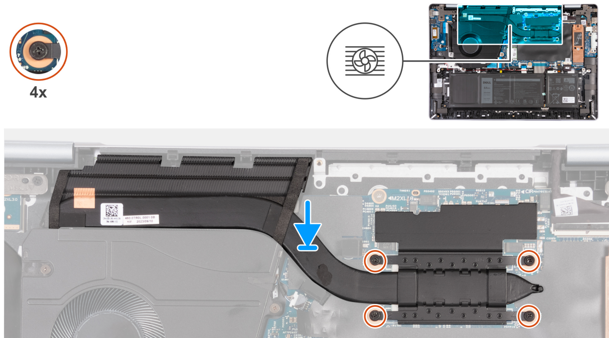
Figure 47. Installing the heat sink
