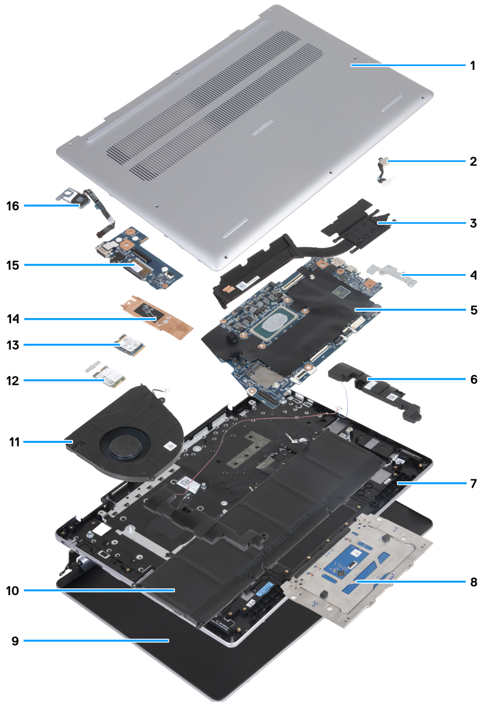
Figure 8. Major components of Inspiron 16 Plus 7640
