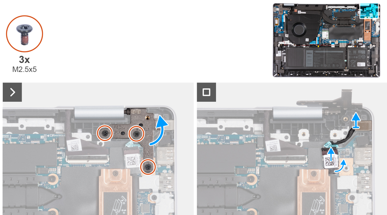
Figure 44. Removing the power-adapter port
