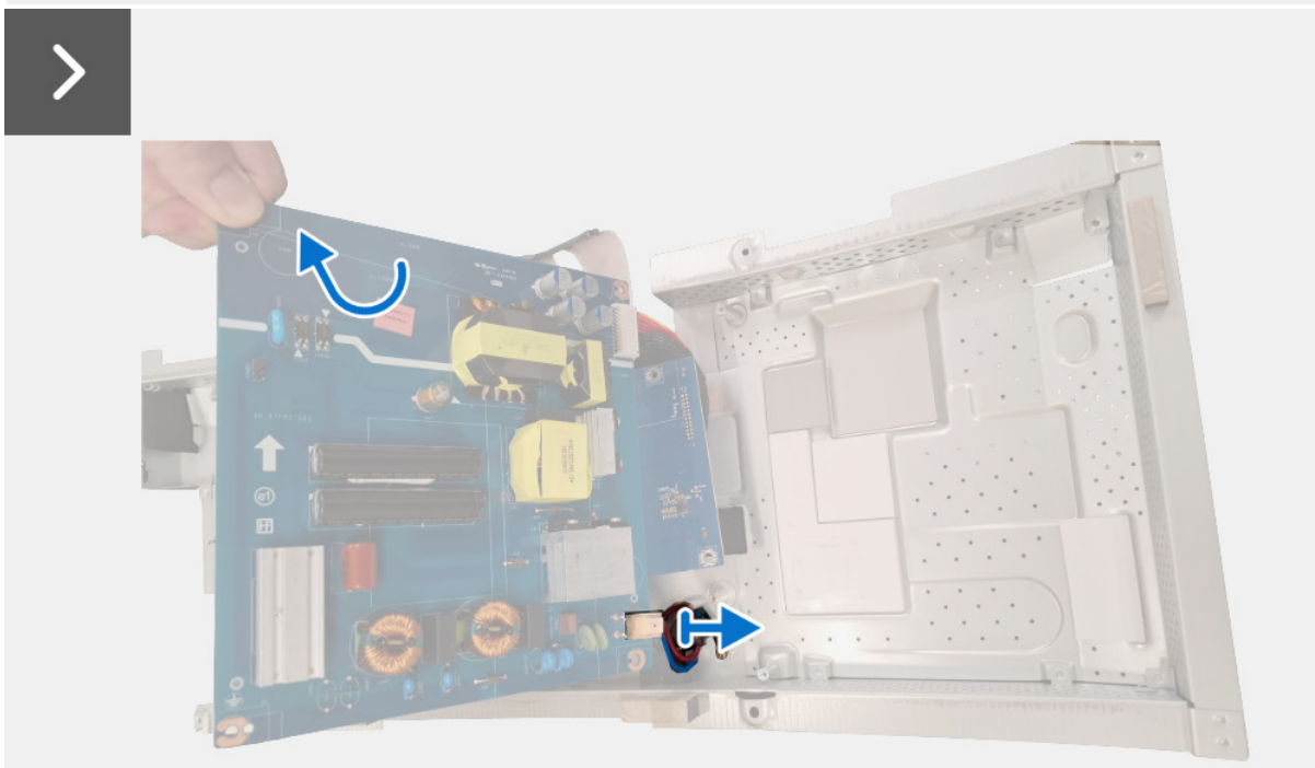
Figure 28. Removing the power board
