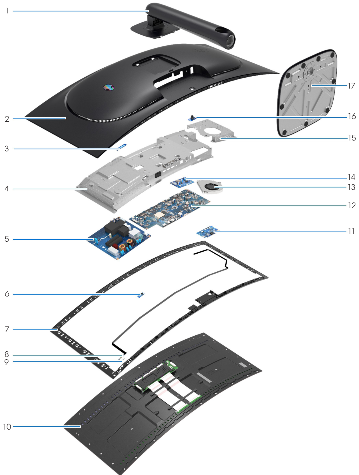
Figure 5. Major components of AW3926QW monitor
