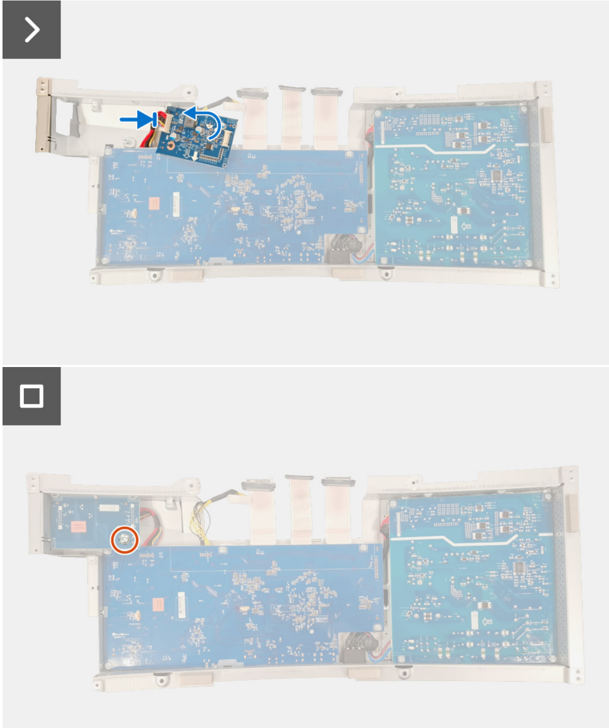
Figure 27. Installing the DC-DC board
