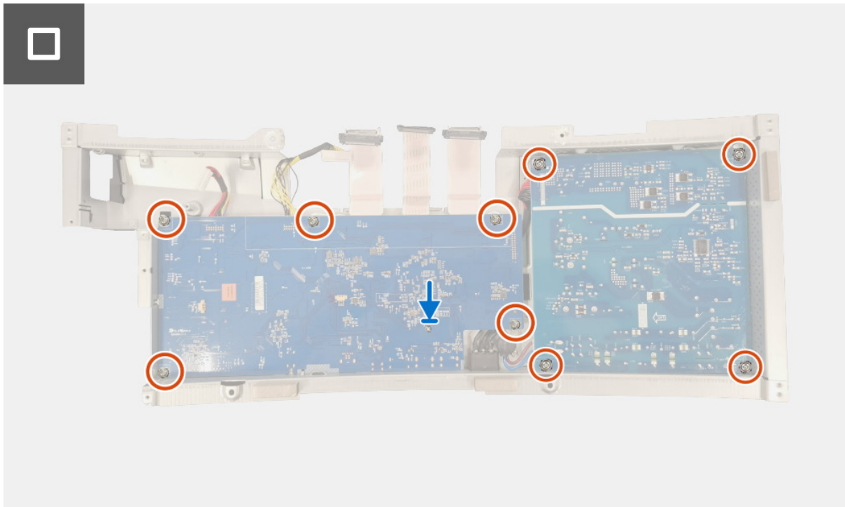
Figure 31. Installing the power board
