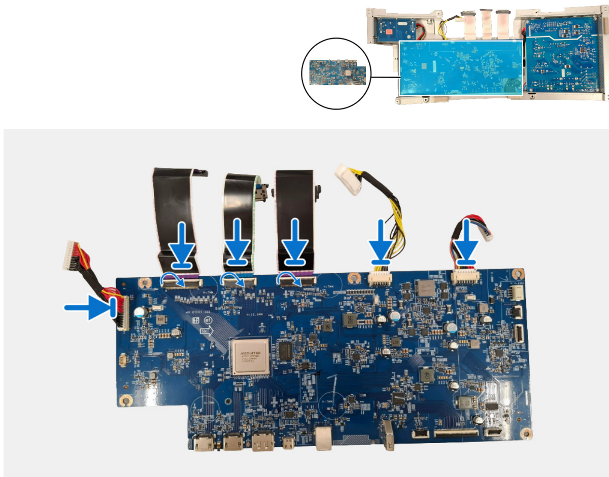
Figure 34. Installing the interface board
