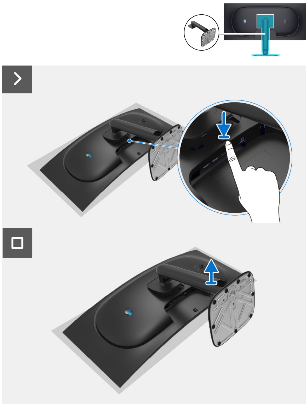
Figure 13. Removing the stand
