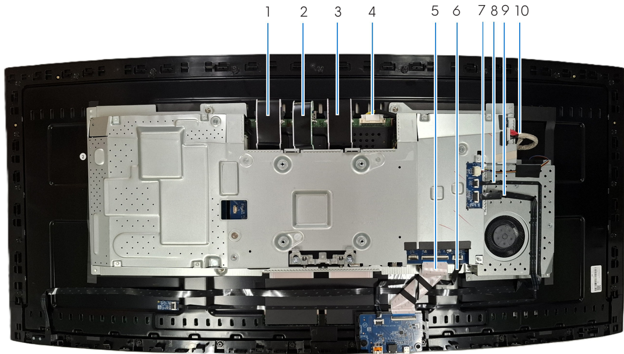
Figure 6. Wiring connectivity on display assembly
