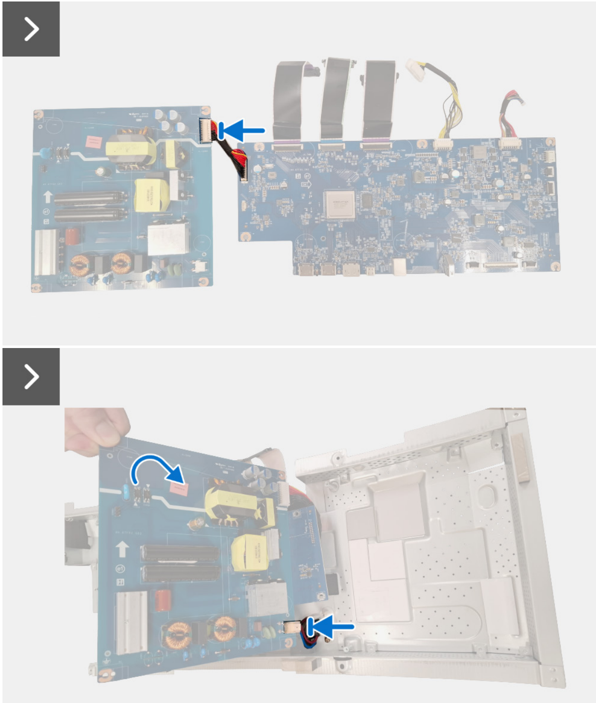
Figure 30. Installing the power board
