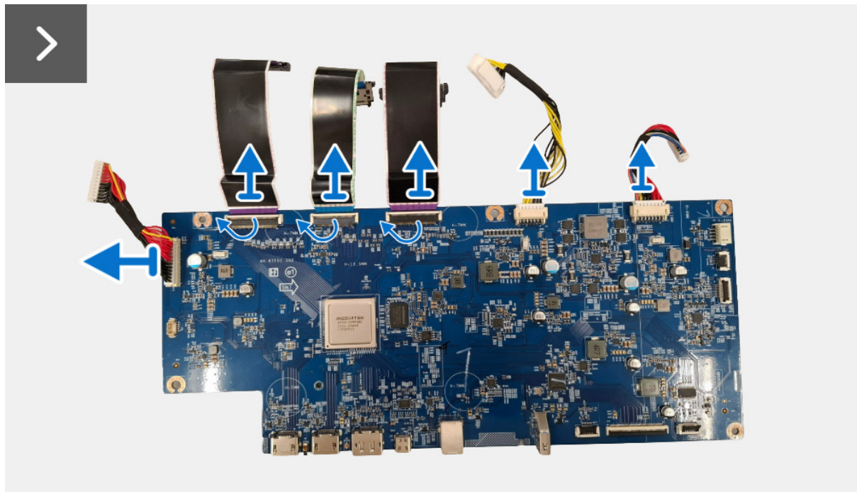
Figure 32. Removing the interface board
