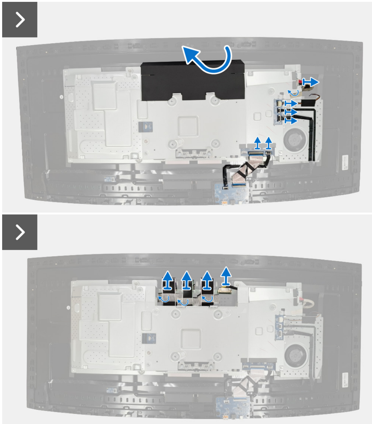
Figure 19. Removing the metal shield
