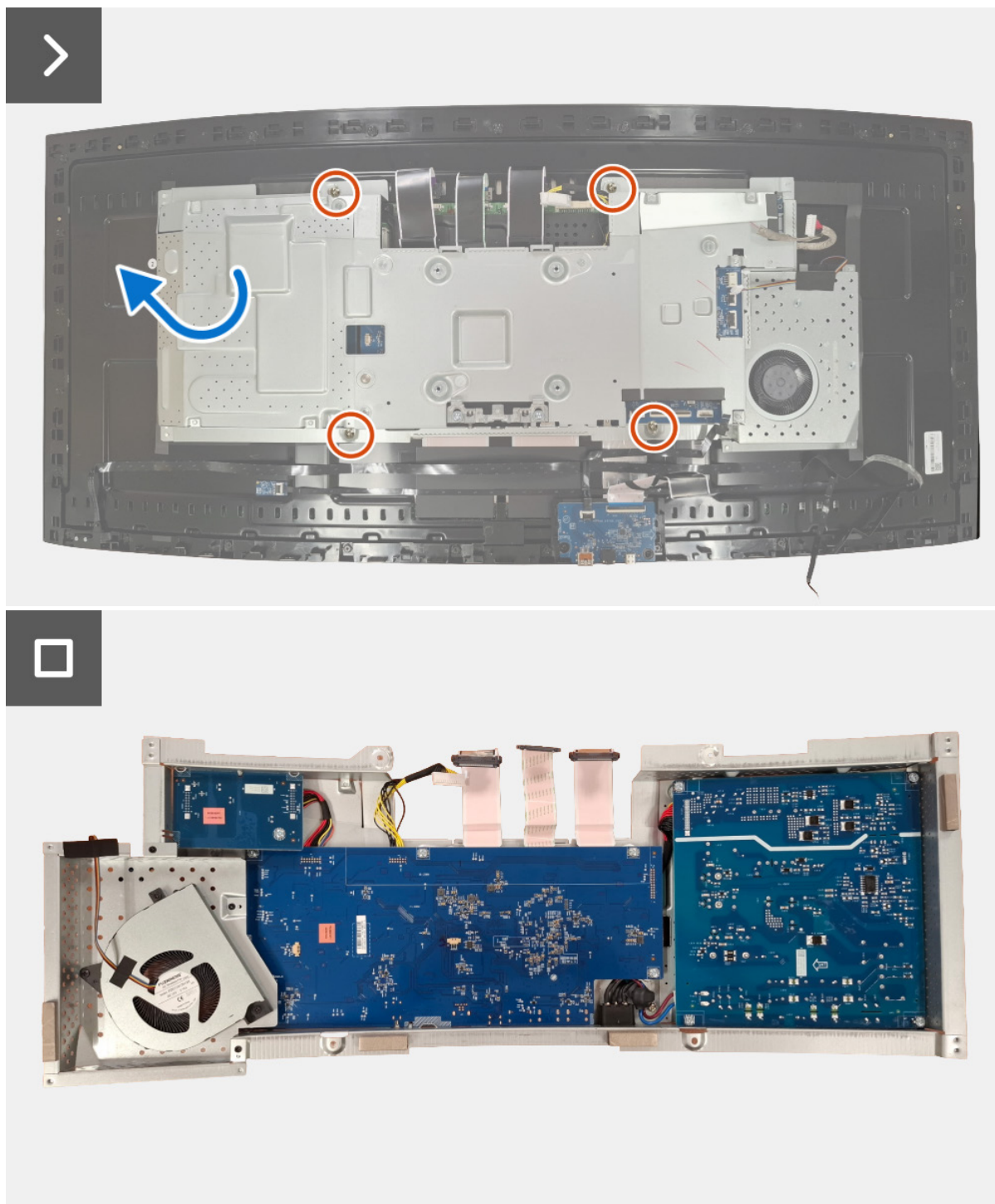
Figure 20. Removing the metal shield
