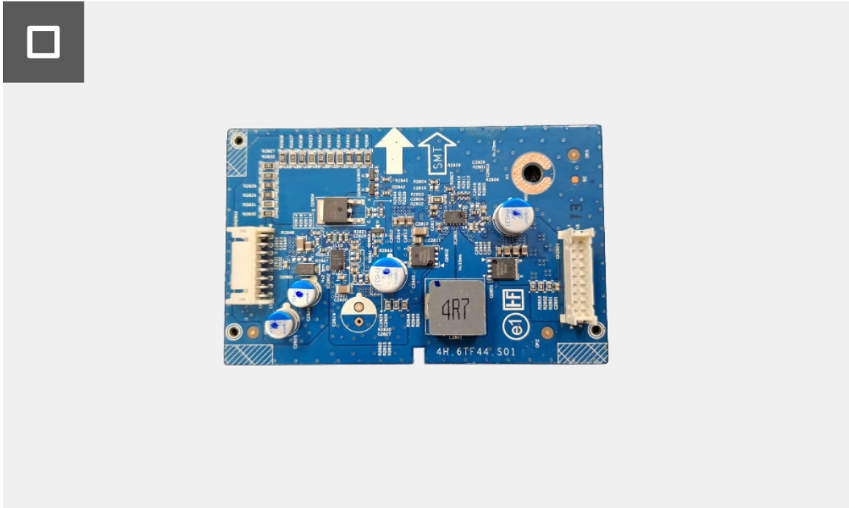
Figure 26. Removing the DC-DC board
