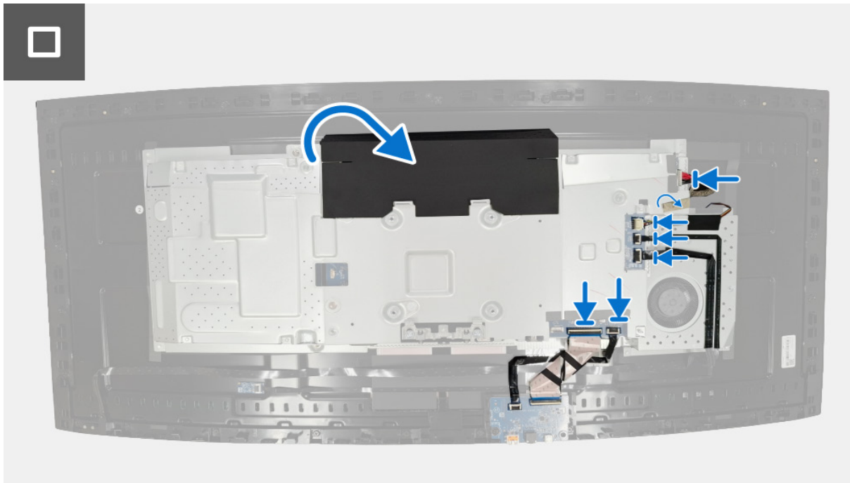
Figure 22. Installing the metal shield
