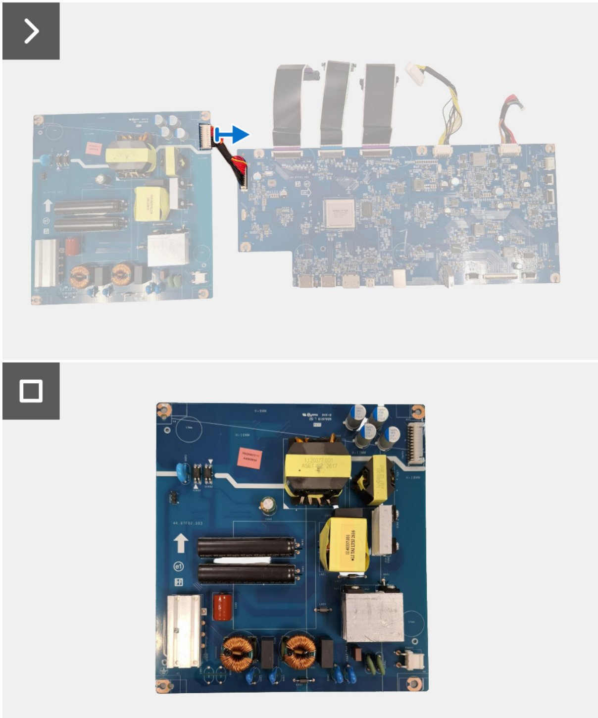
Figure 29. Removing the power board
