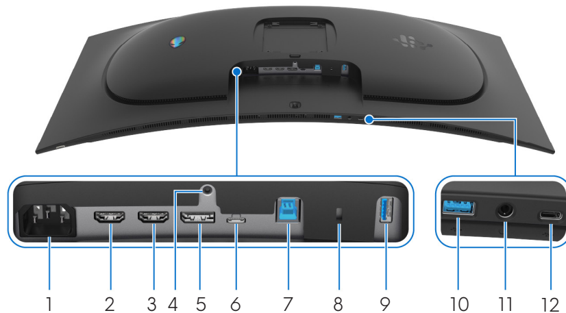
Figure 4. Bottom view of the monitor (without monitor stand)
