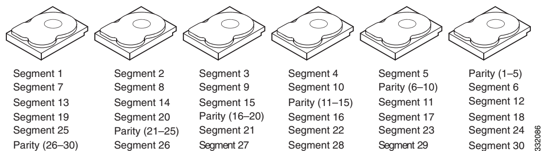
Figure 1-3 Example of Distributed Parity (RAID 5)
