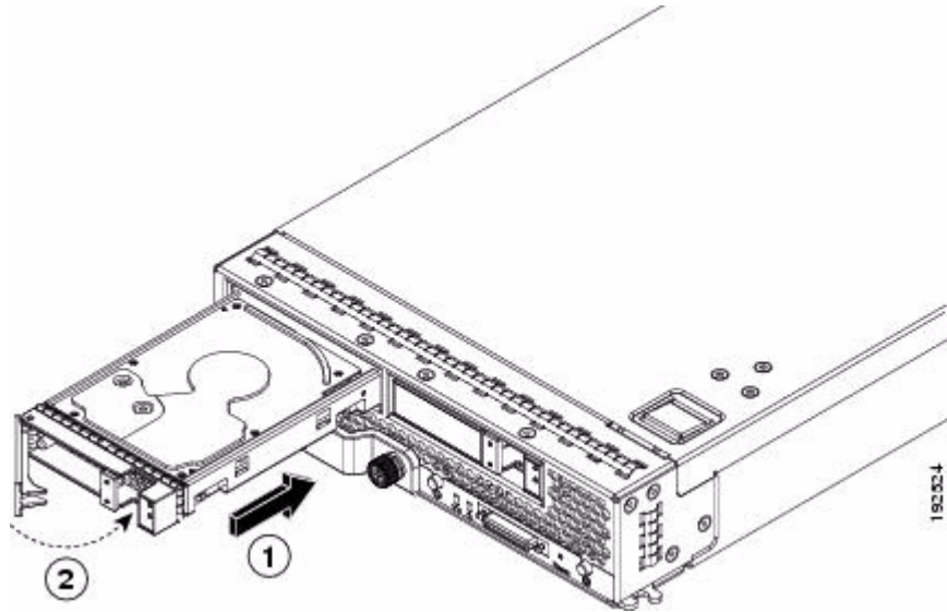
Figure 1-14 Installing a Hard Drive in a Blade Server
