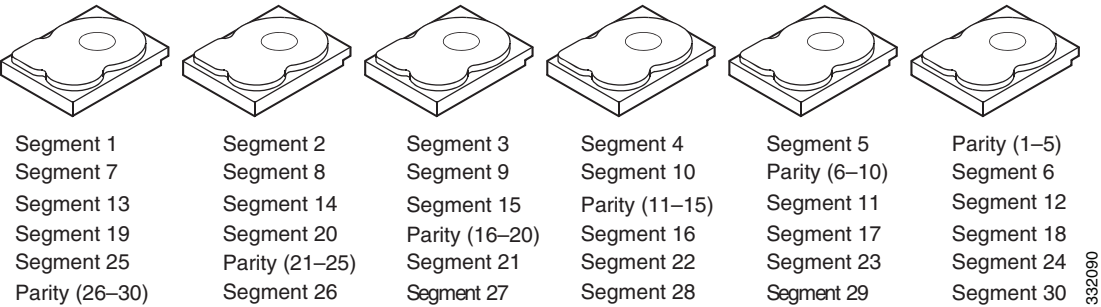
Figure 1-7 RAID 5 Drive Group Example
