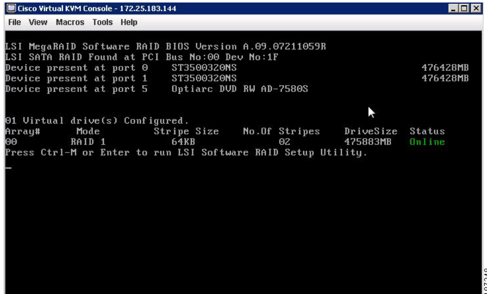
Figure 4-9 ICH10R Launch Window
