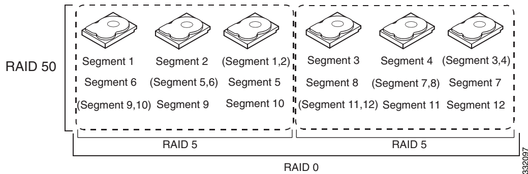
Figure 1-11 RAID 50 Virtual Drive Example
