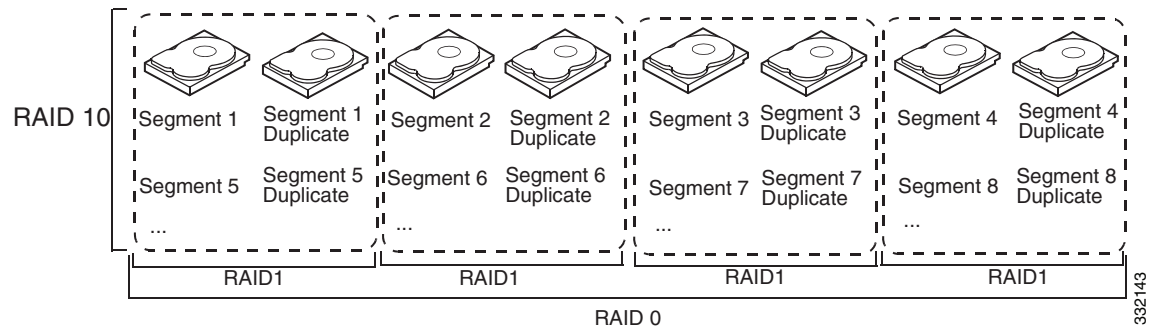
Figure 1-10 RAID 10 Virtual Drive Example
