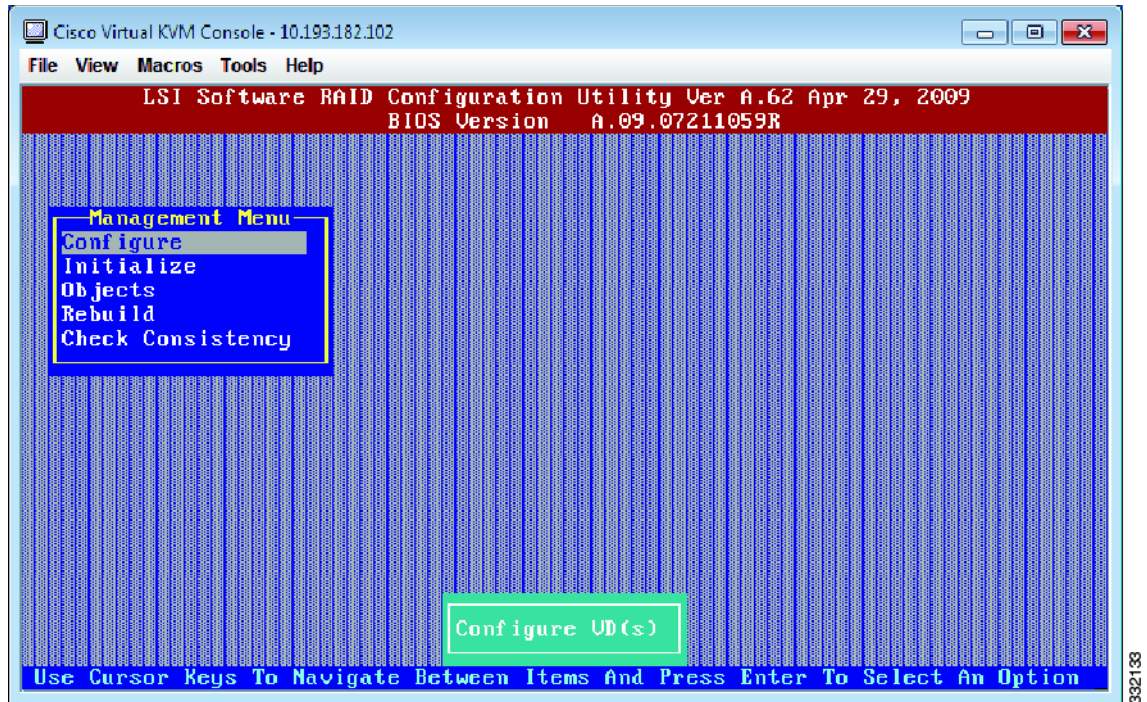
Figure 6-1 Main Setup Utility Window
