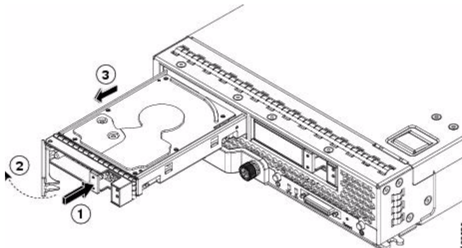
Figure 1-13 Removing the Drive
