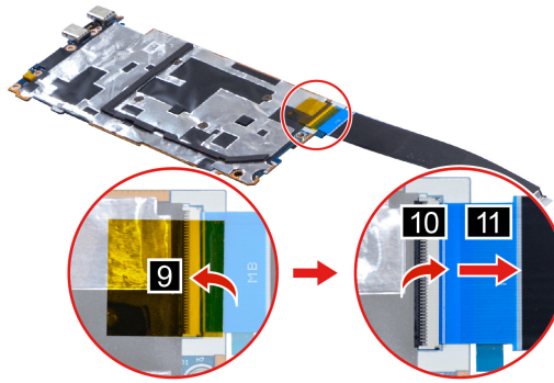
Figure 21. Disconnect the I/O board cable from the system board
