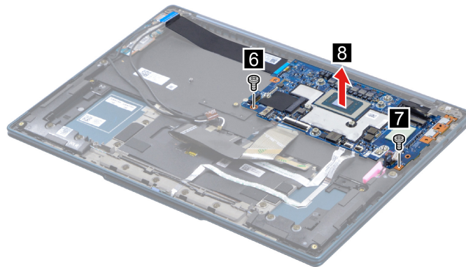
Figure 20. Remove two screws and remove the system board
