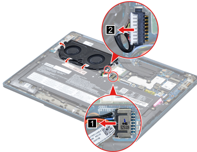
Figure 8. Disconnect the fan cable
