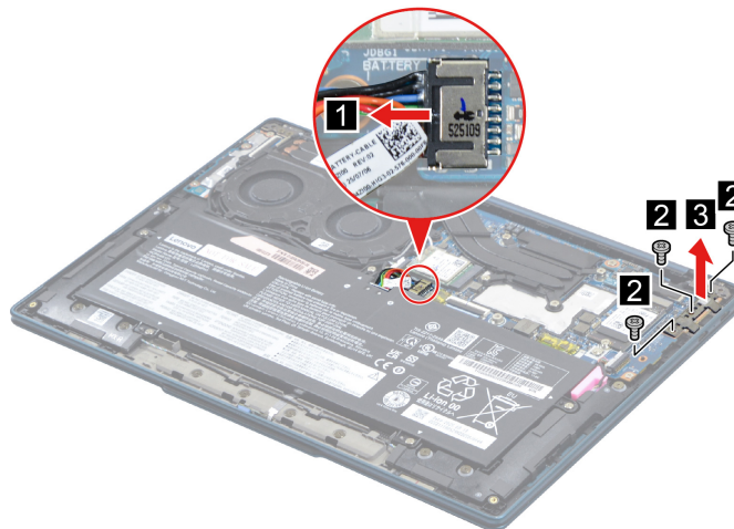
Figure 17. Remove three screws and remove the USB-C bracket
