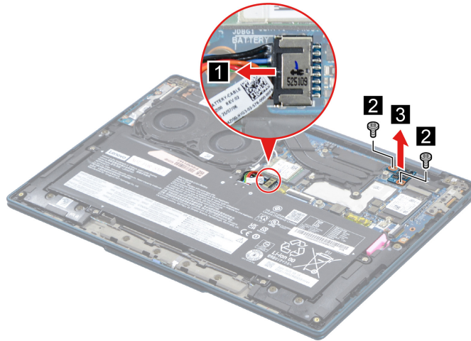
Figure 16. Remove two screws and remove the PMIC board
