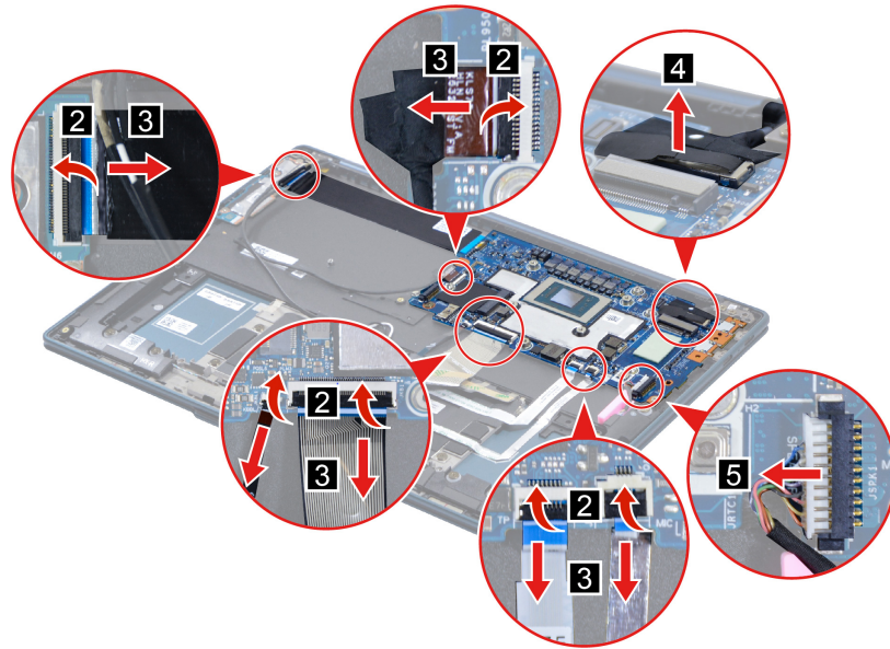
Figure 19. Disconnect cables
