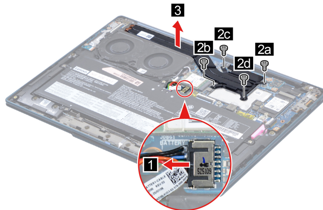
Figure 10. Remove four screws and remove the heat sink
