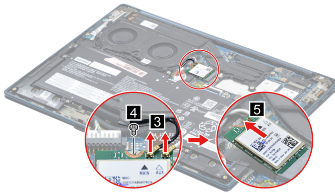
Figure 14. Disconnect cables, remove the screw and remove the Wi-Fi card
