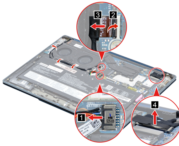
Figure 30. Disconnect the battery pack cable , camera cable and EDP cable from the system board
