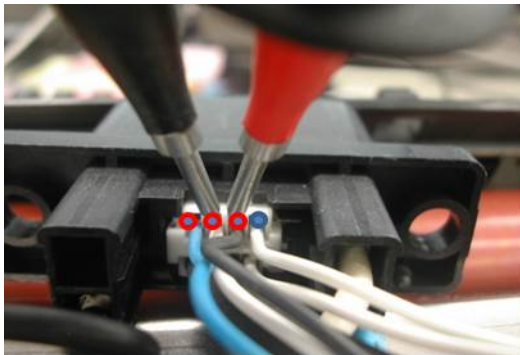
Center Thermistor
