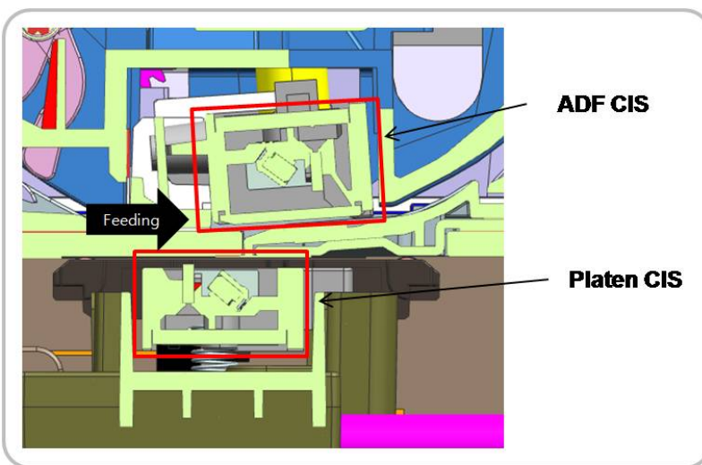
[ Dual scanning system ]
