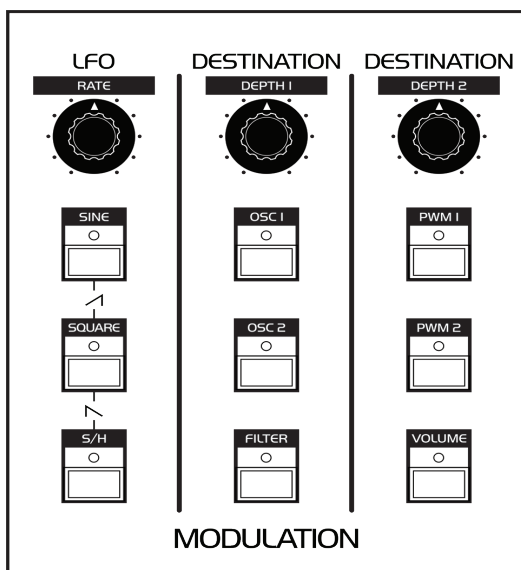
Modulation section
