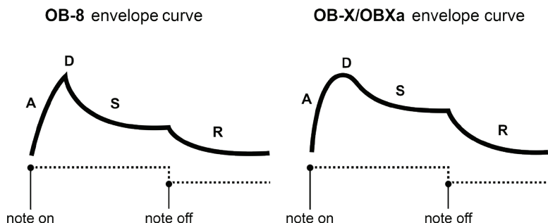
Differences between OB-8 and OB-X/OBXa envelope response
