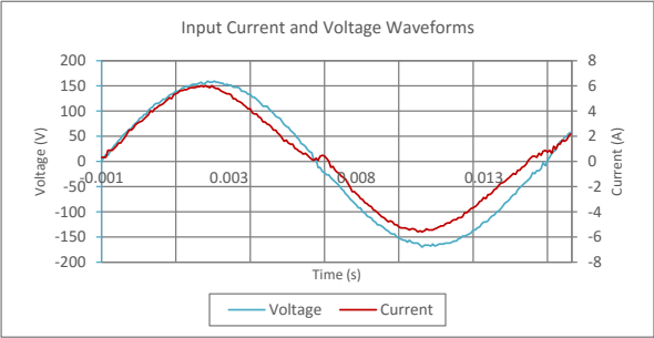
Input AC Current Waveform (ITHD = 10.04%, 50% Load)
